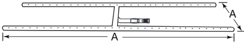
Fig. 1 H-Burner Dimensions (length & width); refer to Table 1.
