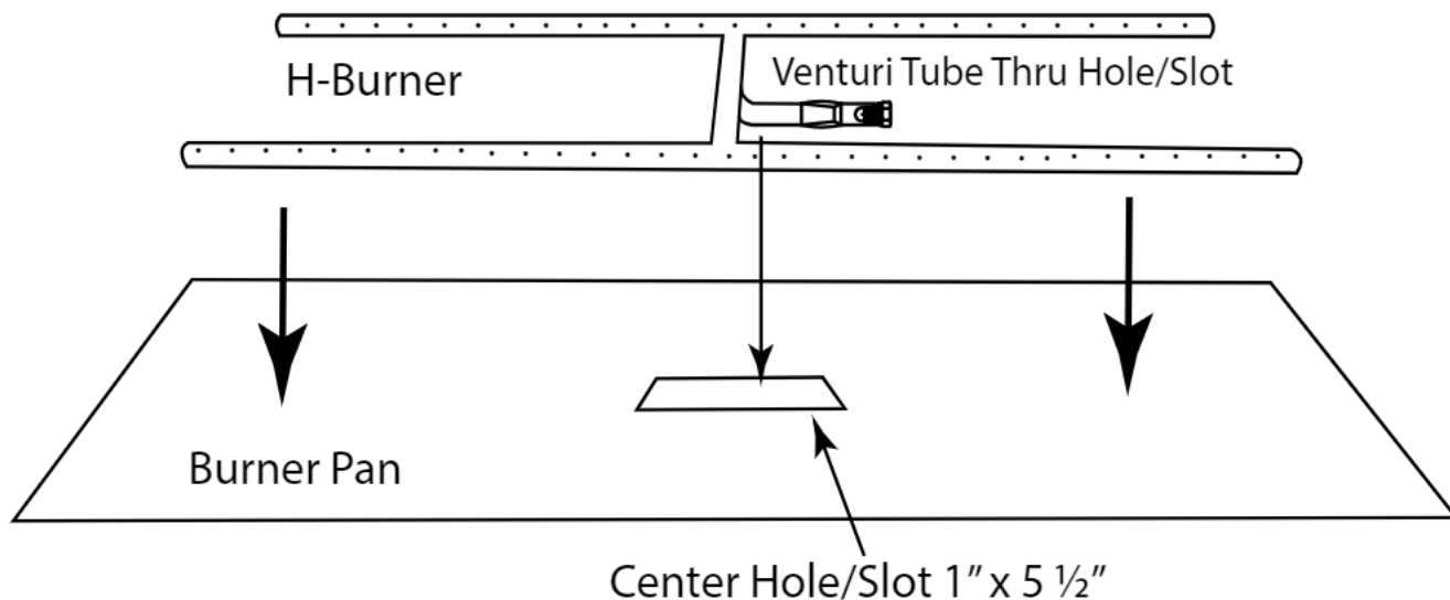
Fig. 4 Installing H-Burner into a pan.
