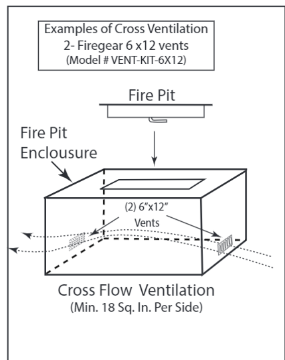
Fig. 3 Cross Ventilation Example
