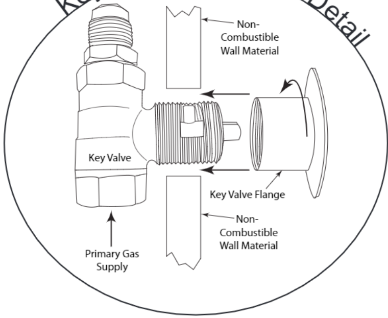
Fig. 10 Typical installations.
