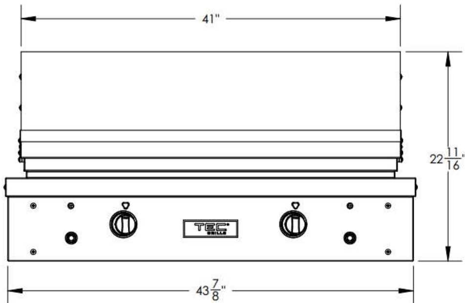
FRONT VIEW
