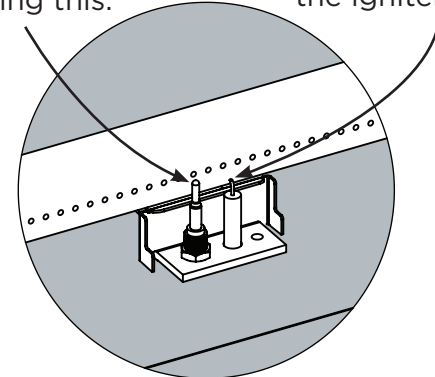
Igniter Housing removed for visibility
