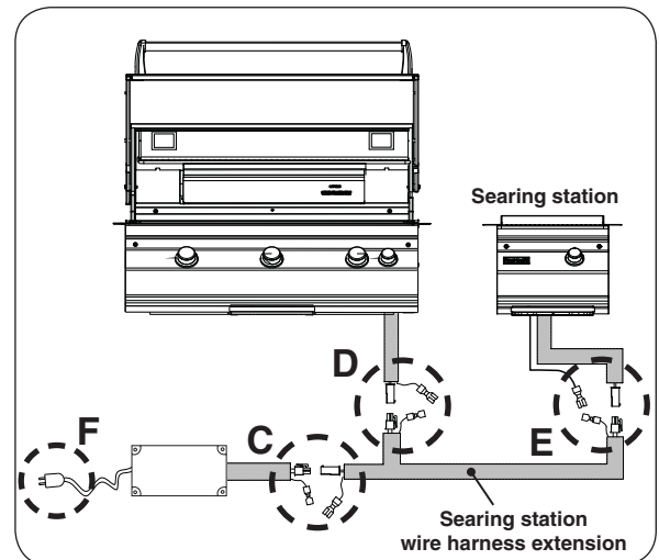
Fig. 17-3 Connect searing station to grill setup
