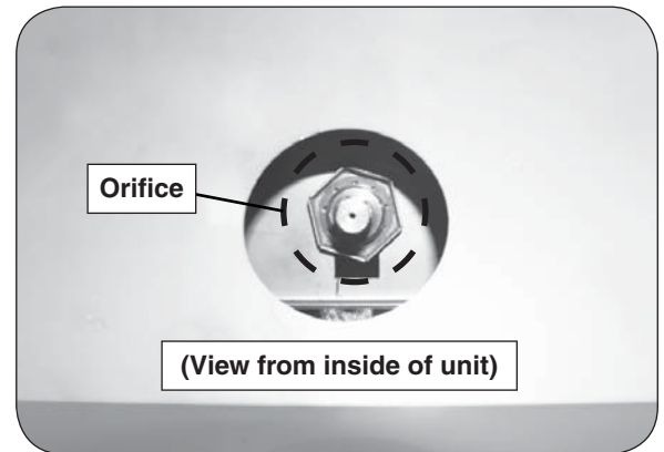
Fig. 27-2 Orifice location
