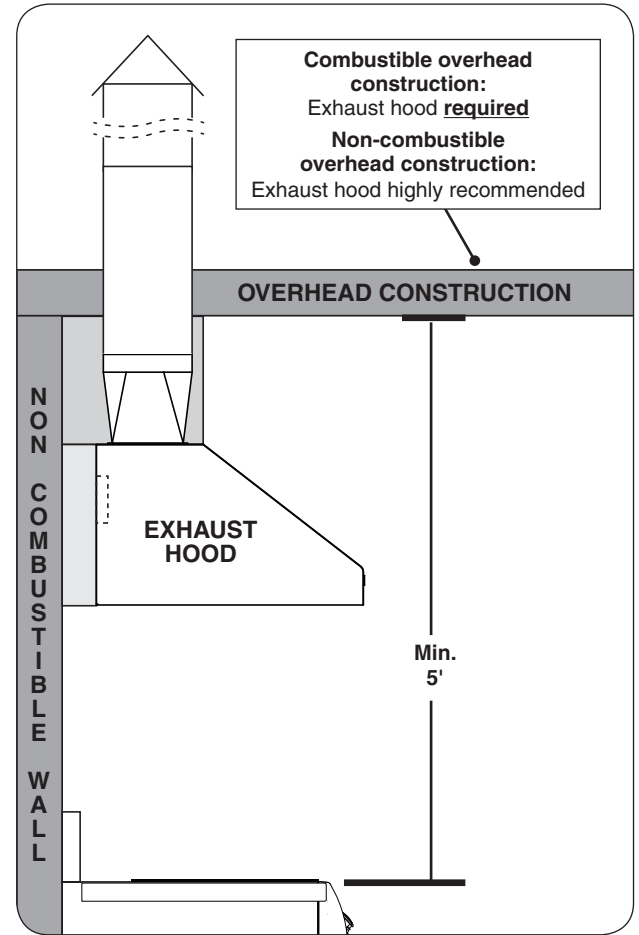
Fig. 9-1 Overhead requirements
