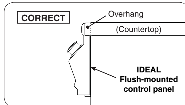
Fig. 16-2 Countertop overhang - correct cutout
