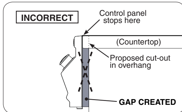
Fig. 16-1 Countertop overhang - incorrect cutout
