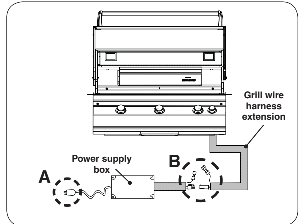
Fig. 17-2 Disconnect grill connections
