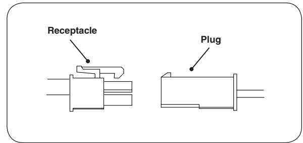
Fig. 17-1 Connection detail
