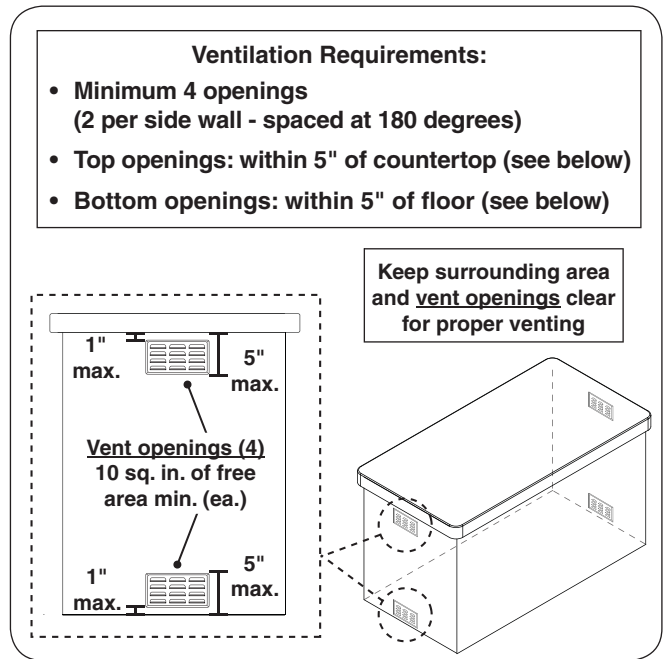
Fig. 12-1 Ventilation detail
