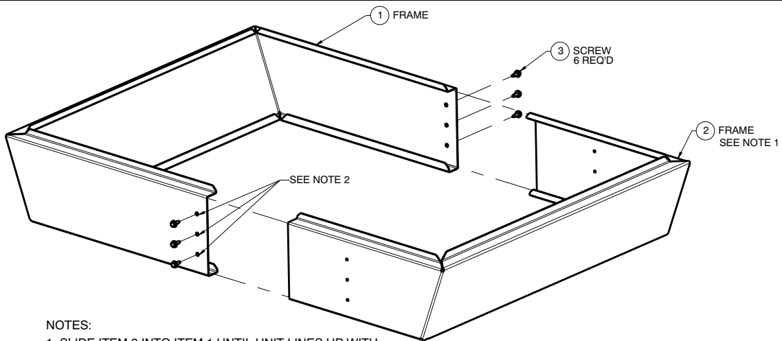
Figure 3 Coil Adapter – Coil One Size Wider than Furnace, Coil Centered on Furnace
