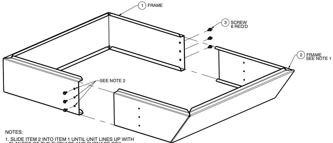
Figure 2 Coil Adapter – Coil One Size Wider than Furnace, Coil Offset to One Side of Furnace
