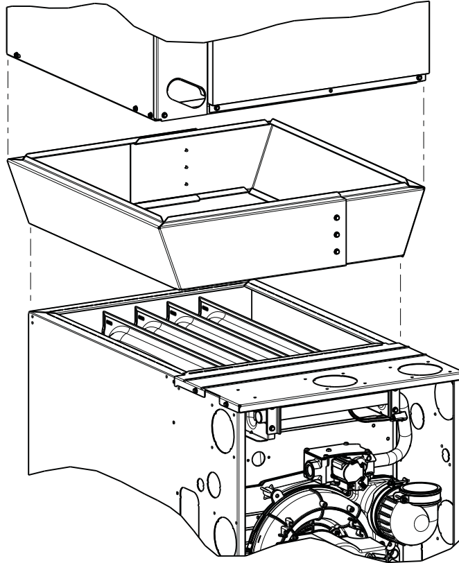
Horizontal-Right Installation
