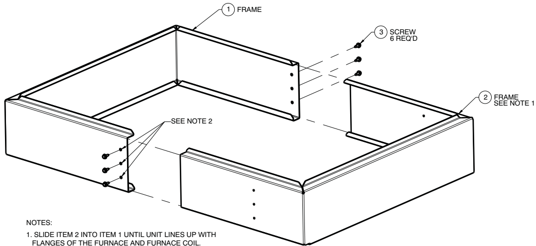
Figure 1 Coil Adapter – Coil Width Same as Furnace
