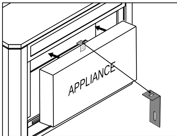
Appliance secure bracket installation location.
