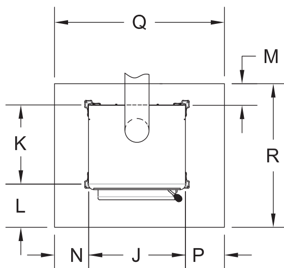
FLOOR PROTECTOR DIMENSIONS
