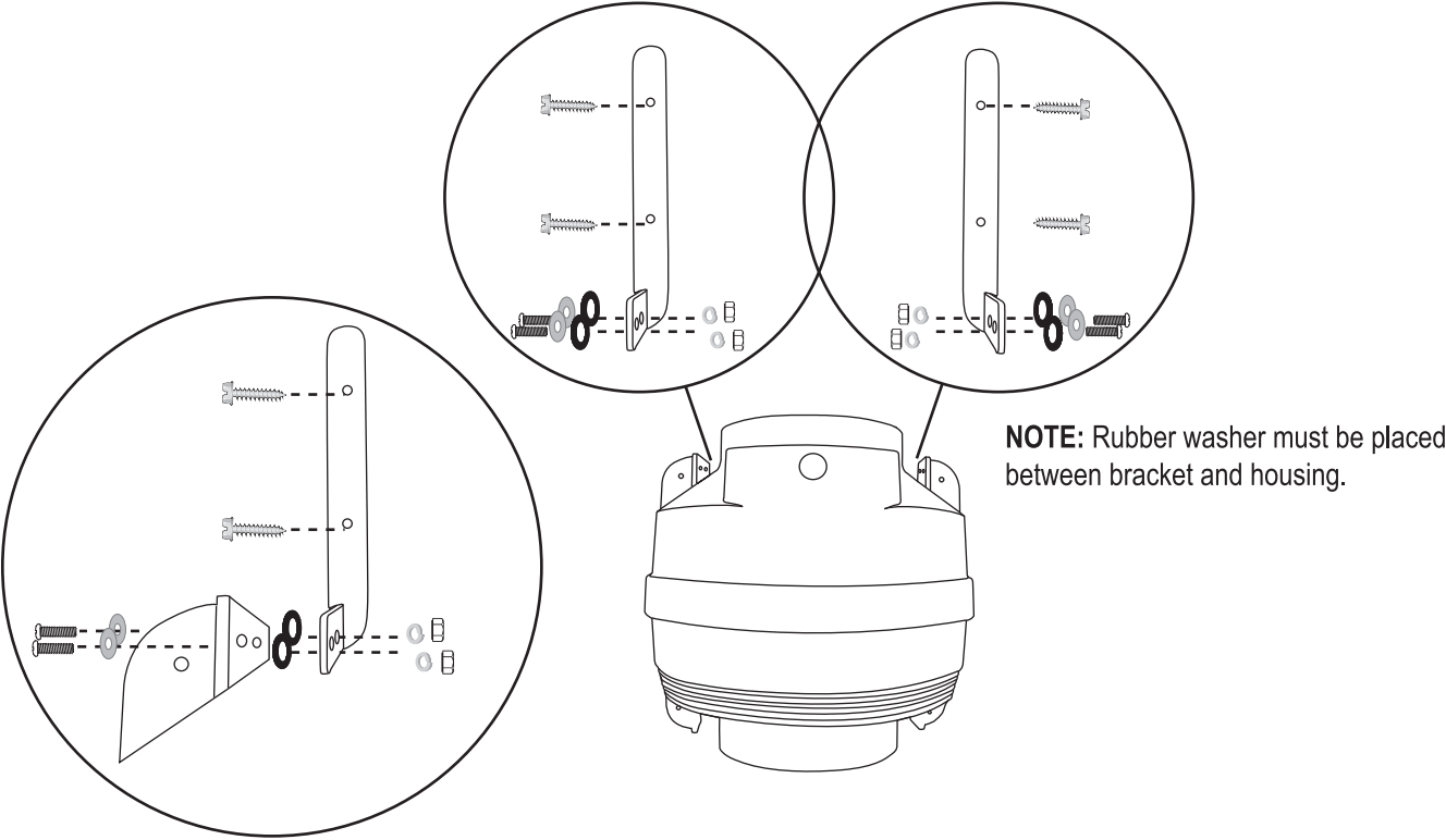
FIGURE 1: MOUNTING BRACKETS
