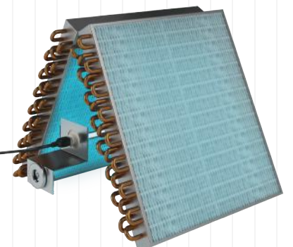
AC Coil with UV Light
