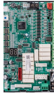
INDOOR AHU CONTROL BOARD
