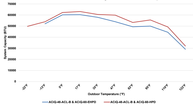
48K A-Coils & 60K Condenser Cooling Performance at 80°F Setpoint
