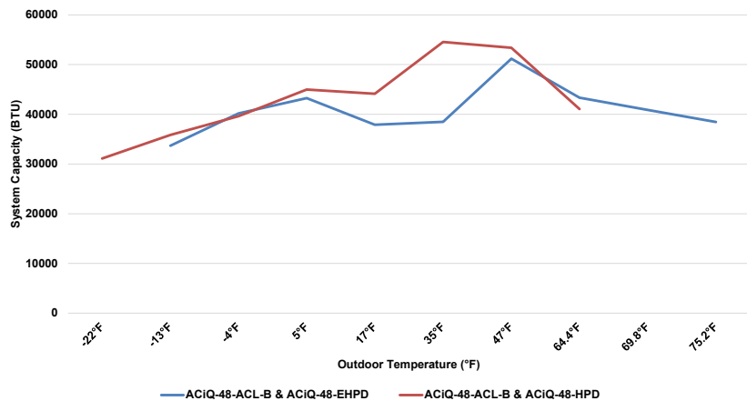
48K A-Coils & 48K Condenser Heating Performance at 70°F Setpoint
