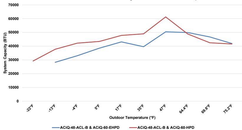
48K A-Coils & 60K Condenser Heating Performance at 70°F Setpoint
