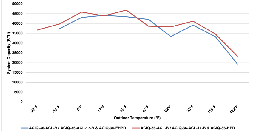
36K A-Coils & 36K Condenser Cooling Performance at 80°F Setpoint
