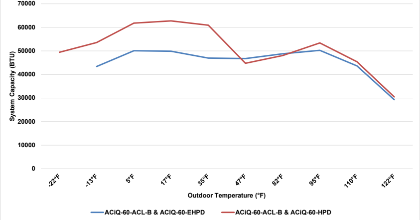
60K A-Coils & 60K Condenser Cooling Performance at 80°F Setpoint
