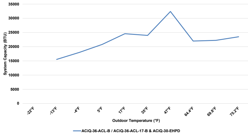
36K A-Coils & 30K Condenser Heating Performance at 70°F Setpoint
