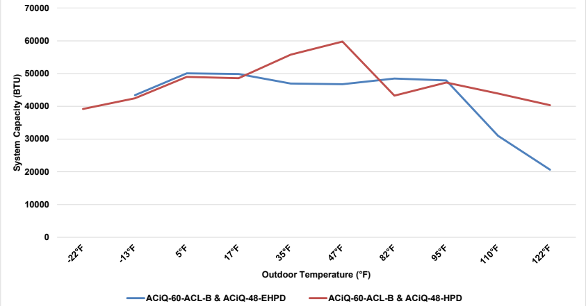
60K A-Coils & 48K Condenser Cooling Performance at 80°F Setpoint
