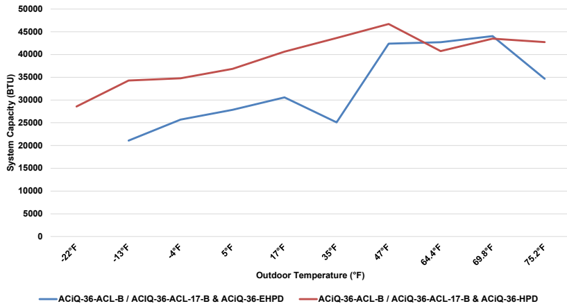
36K A-Coils & 36K Condenser Heating Performance at 70°F Setpoint
