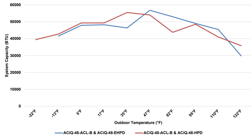
48K A-Coils & 48K Condenser Cooling Performance at 80°F Setpoint
