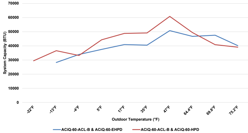
60K A-Coils & 60K Condenser Heating Performance at 70°F Setpoint
