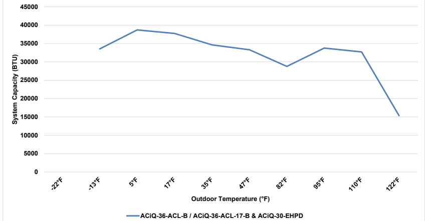
36K A-Coils & 30K Condenser Cooling Performance at 80°F Setpoint
