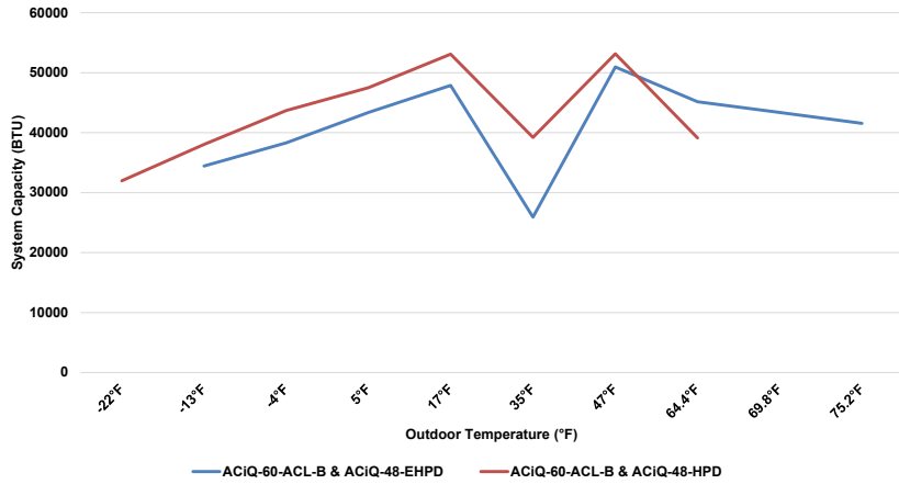
60K A-Coils & 48K Condenser Heating Performance at 70°F Setpoint
