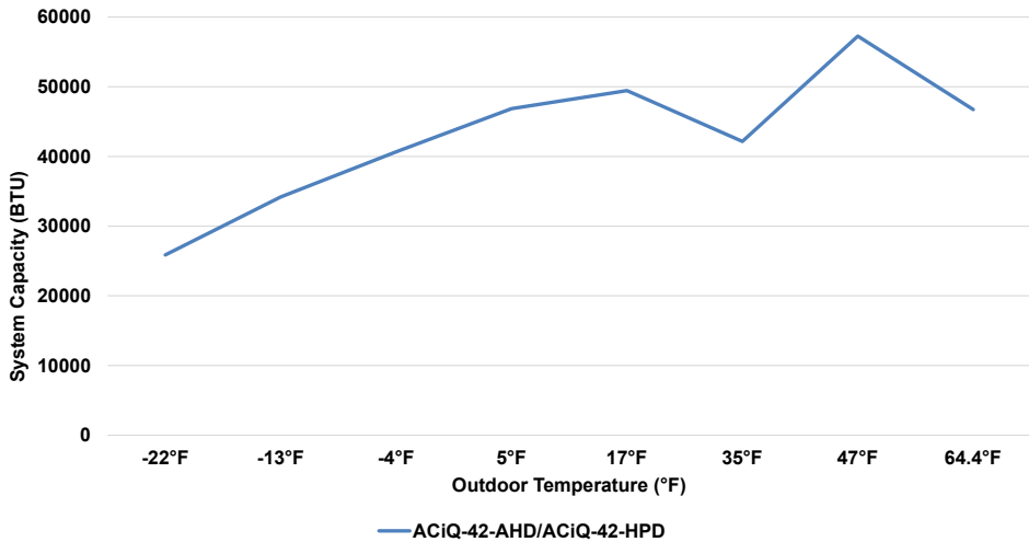
42K System Heating Performance at 70°F Setpoint
