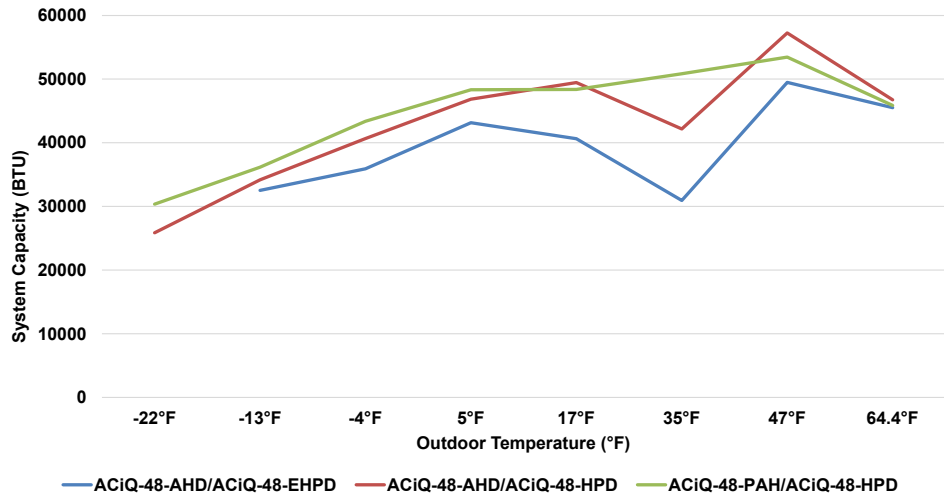
48K System Heating Performance at 70°F Setpoint
