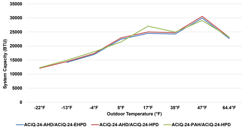
24K System Heating Performance at 70°F Setpoint
