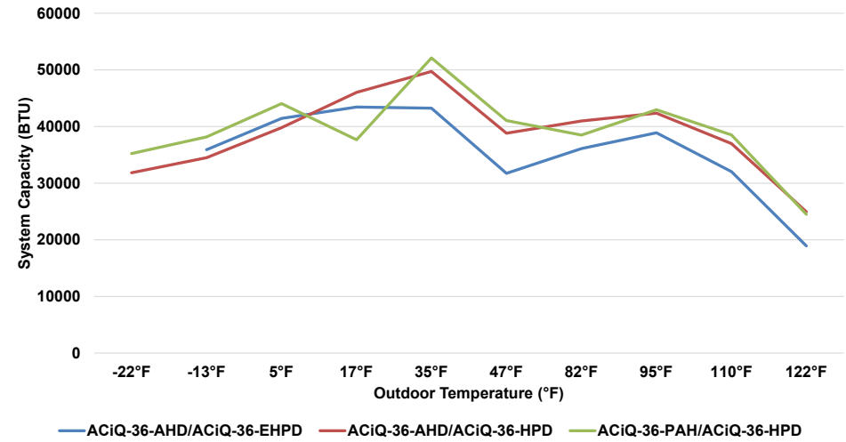
36K System Cooling Performance at 80°F Setpoint
