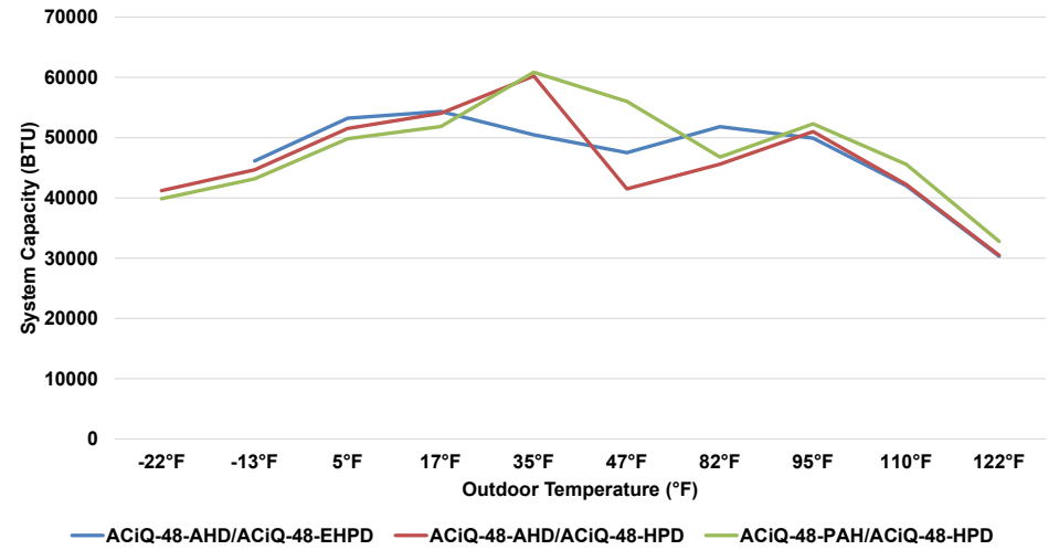
48K System Cooling Performance at 80°F Setpoint
