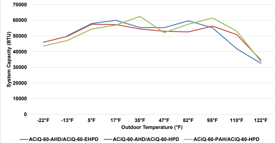
60K System Cooling Performance at 80°F Setpoint
