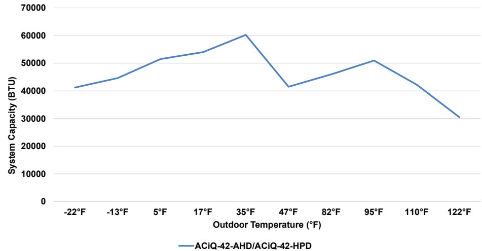
42K System Cooling Performance at 80°F Setpoint
