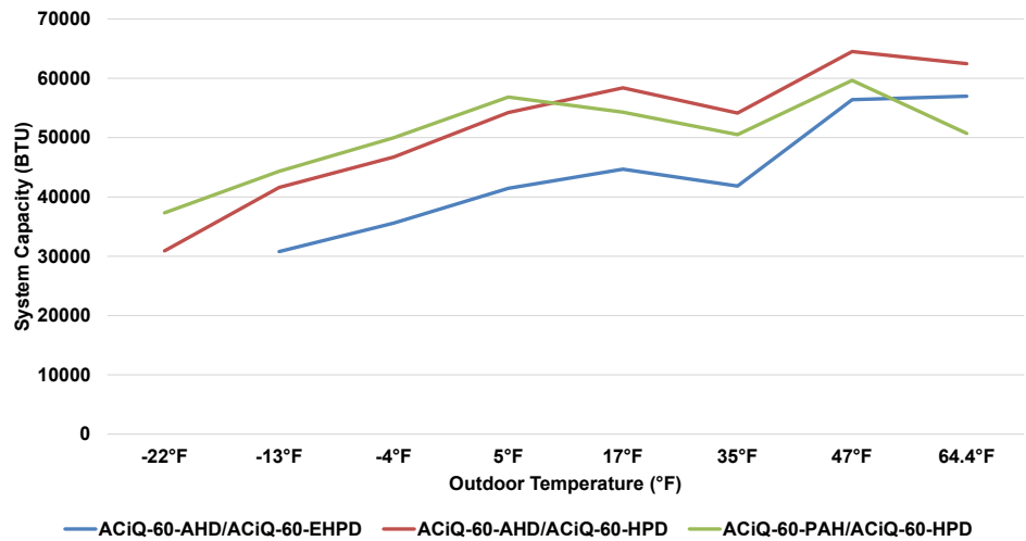
60K System Heating Performance at 70°F Setpoint
