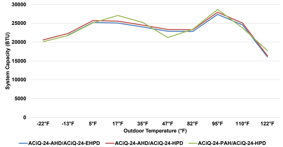
24K System Cooling Performance at 80°F Setpoint
