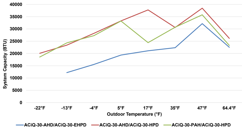
30K System Heating Performance at 70°F Setpoint
