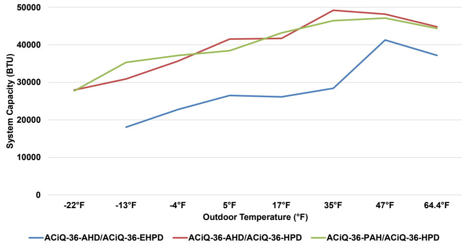
36K System Heating Performance at 70°F Setpoint
