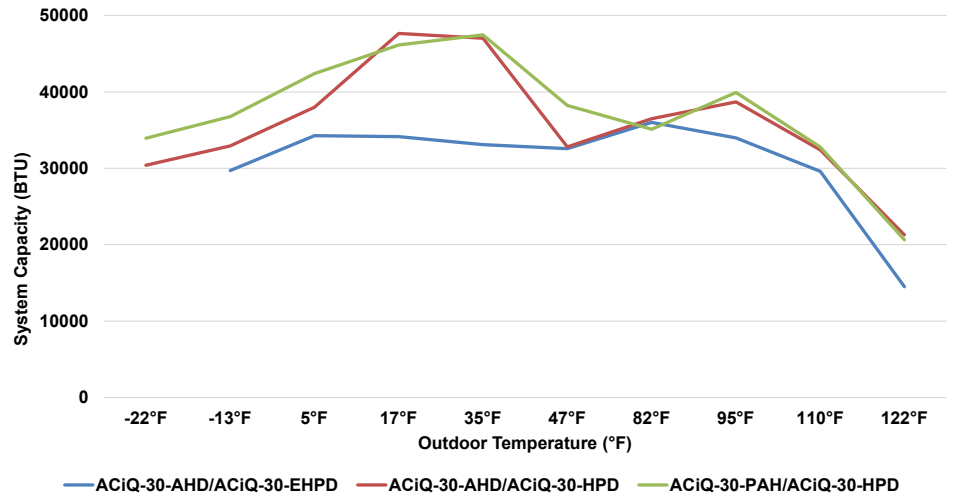
30K System Cooling Performance at 80°F Setpoint
