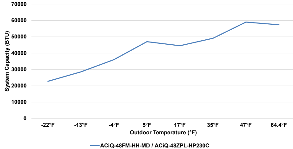
48K Console/Floor & Ceiling Mounted Air Handler & 48K Ext. Heat Single-Zone Condenser Heating Performance at 70°F Setpoint
