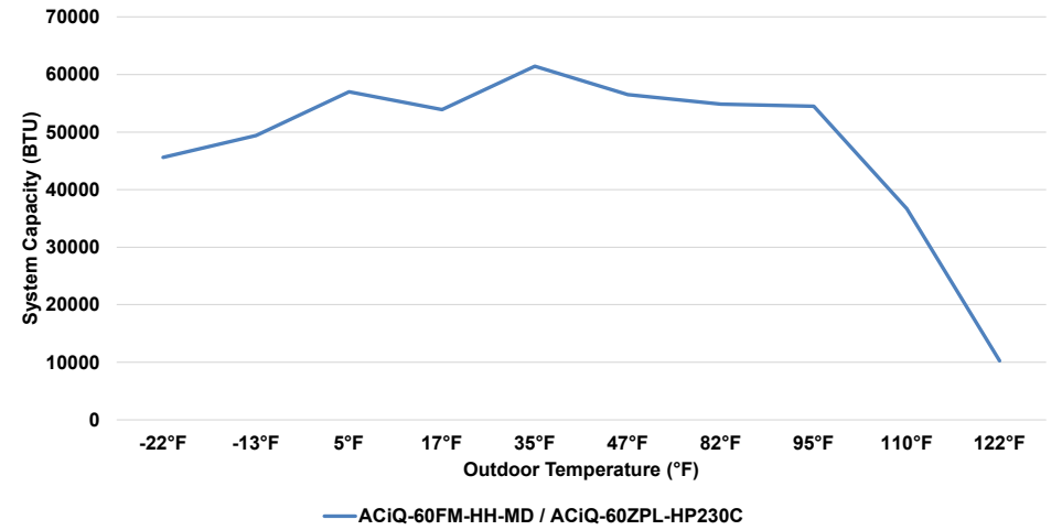
60K Console/Floor & Ceiling Mounted Air Handler & 60K Ext. Heat Single-Zone Condenser Cooling Performance at 80°F Setpoint
