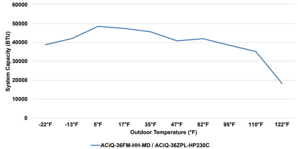
36K Console/Floor & Ceiling Mounted Air Handler & 36K Ext. Heat Single-Zone Condenser Cooling Performance at 80°F Setpoint
