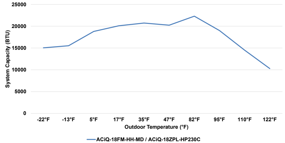
18K Console/Floor & Ceiling Mounted Air Handler & 18K Ext. Heat Single-Zone Condenser Cooling Performance at 80°F Setpoint
