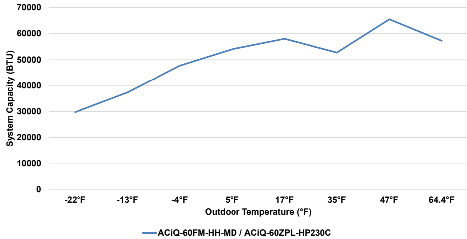
60K Console/Floor & Ceiling Mounted Air Handler & 60K Ext. Heat Single-Zone Condenser Heating Performance at 70°F Setpoint
