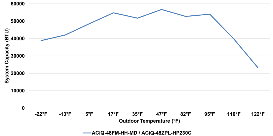
48K Console/Floor & Ceiling Mounted Air Handler & 48K Ext. Heat Single-Zone Condenser Cooling Performance at 80°F Setpoint
