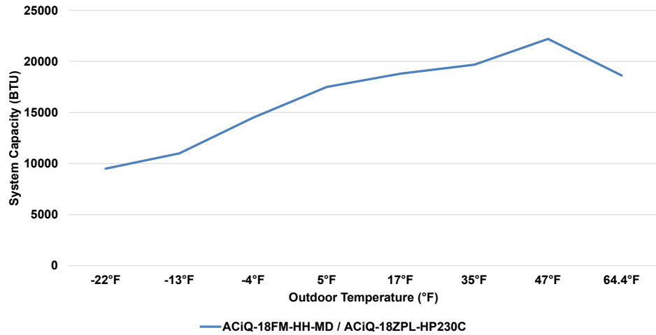
18K Console/Floor & Ceiling Mounted Air Handler & 18K Ext. Heat Single-Zone Condenser Heating Performance at 70°F Setpoint
