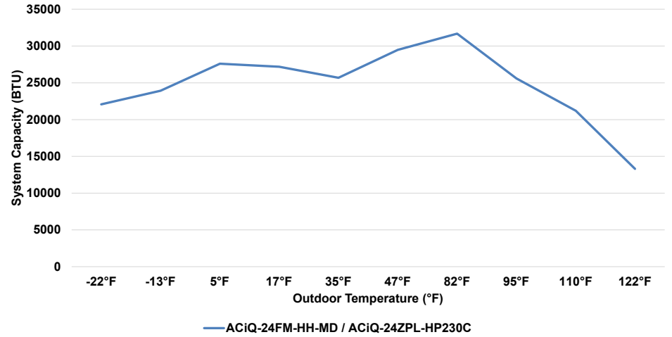
24K Console/Floor & Ceiling Mounted Air Handler & 24K Ext. Heat Single-Zone Condenser Cooling Performance at 80°F Setpoint
