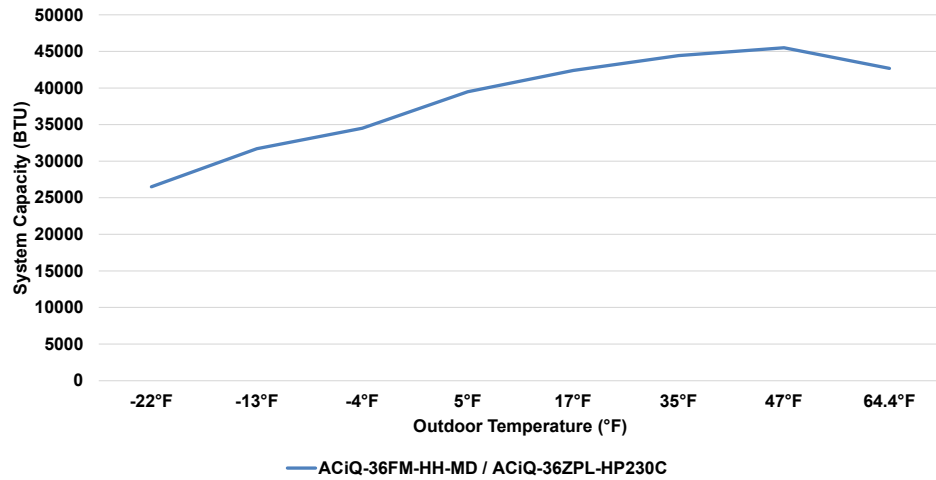
36K Console/Floor & Ceiling Mounted Air Handler & 36K Ext. Heat Single-Zone Condenser Heating Performance at 70°F Setpoint
