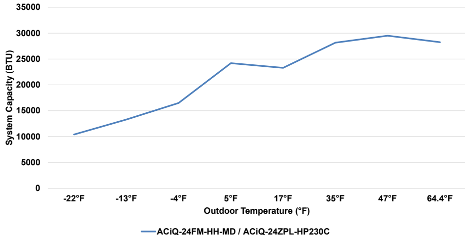
24K Console/Floor & Ceiling Mounted Air Handler & 24K Ext. Heat Single-Zone Condenser Heating Performance at 70°F Setpoint
