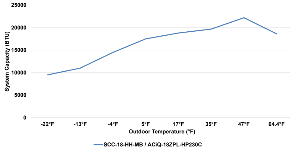
18K Slim Ceiling Cassette Air Handler & 18K Extreme Heat Single-Zone Condenser Heating Performance at 70°F Setpoint
