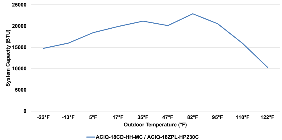
18K Concealed Duct Air Handler & 18K Extreme Heat Single-Zone Condenser Cooling Performance at 80°F Setpoint
