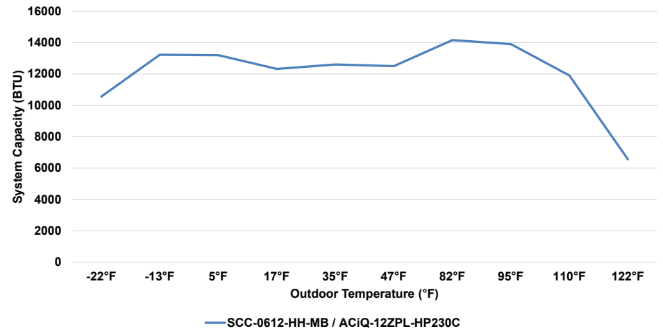
12K Slim Ceiling Cassette Air Handler & 12K Extreme Heat Single-Zone Condenser Cooling Performance at 80°F Setpoint
