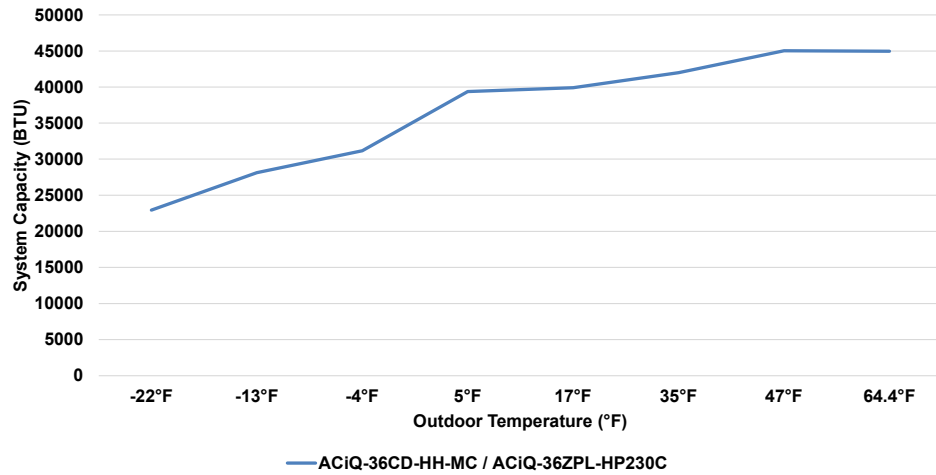
36K Cocealed Duct Air Handler & 36K Extreme Heat Single-Zone Condenser Heating Performance at 70°F Setpoint
