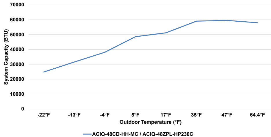
48K Concealed Duct Air Handler & 48K Extreme Heat Single-Zone Condenser Heating Performance at 70°F Setpoint
