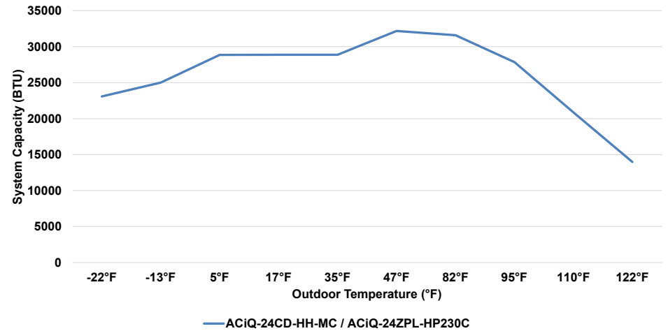
24K Concealed Duct Air Handler & 24K Extreme Heat Single-Zone Condenser Cooling Performance at 80°F Setpoint
