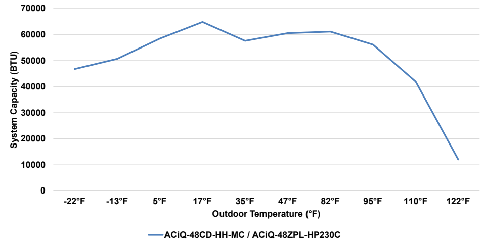
48K Concealed Duct Air Handler & 48K Extreme Heat Single-Zone Condenser Cooling Performance at 80°F Setpoint
