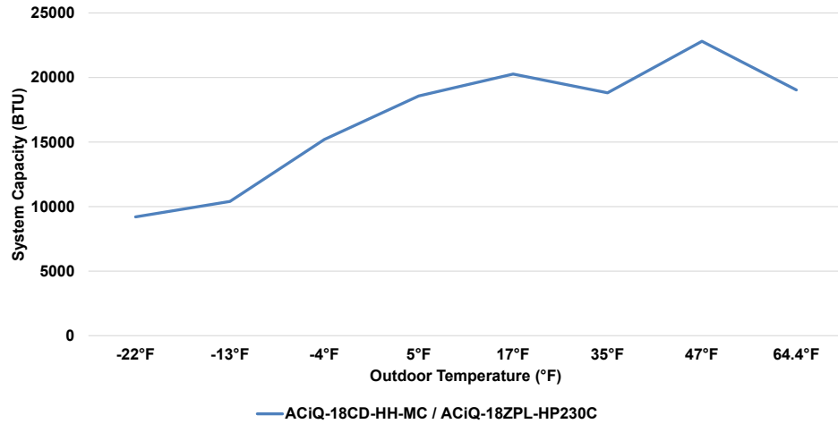
18K Concealed Duct Air Handler & 18K Extreme Heat Single-Zone Condenser Heating Performance at 70°F Setpoint
