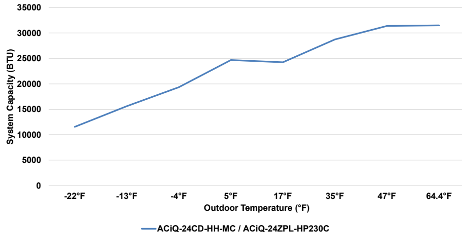
24K Concealed Duct Air Handler & 24K Extreme Heat Single-Zone Condenser Heating Performance at 70°F Setpoint
