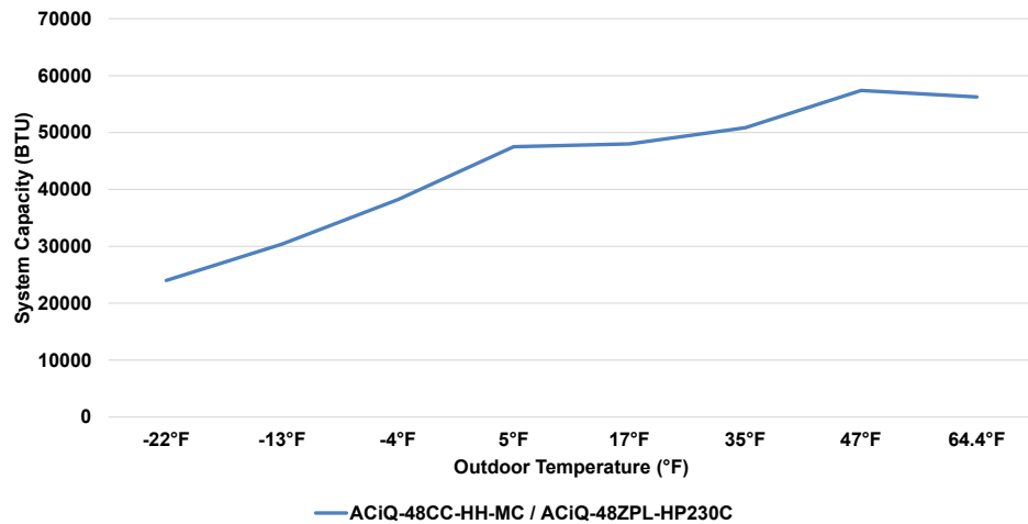
48K Ceiling Cassette Air Handler & 48K Extreme Heat Single-Zone Condenser Heating Performance at 70°F Setpoint
