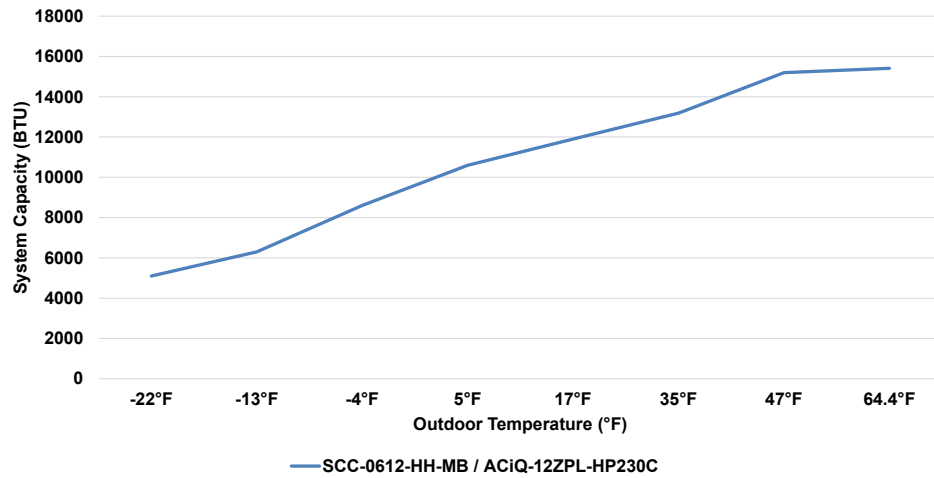
12K Slim Ceiling Cassette Air Handler & 12K Extreme Heat Single-Zone Condenser Heating Performance at 70°F Setpoint
