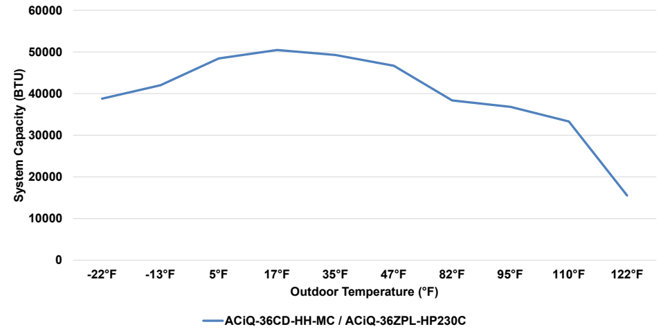
36K Concealed Duct Air Handler & 36K Extreme Heat Single-Zone Condenser Cooling Performance at 80°F Setpoint
