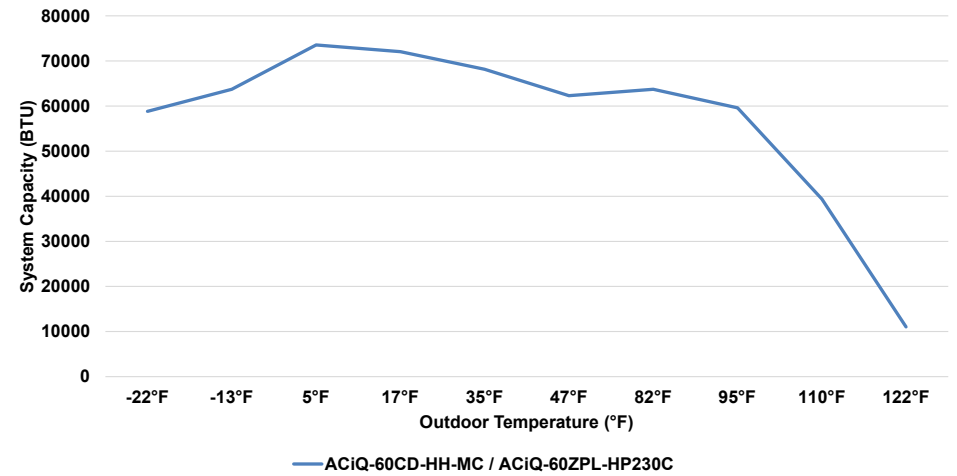
60K Concealed Duct Air Handler & 60K Extreme Heat Single-Zone Condenser Cooling Performance at 80°F Setpoint
