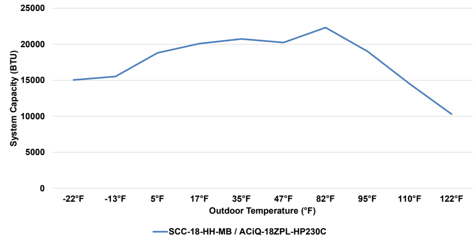
18K Slim Ceiling Cassette Air Handler & 18K Extreme Heat Single-Zone Condenser Cooling Performance at 80°F Setpoint
