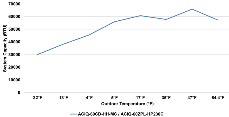
60K Concealed Duct Air Handler & 60K Extreme Heat Single-Zone Condenser Heating Performance at 70°F Setpoint
