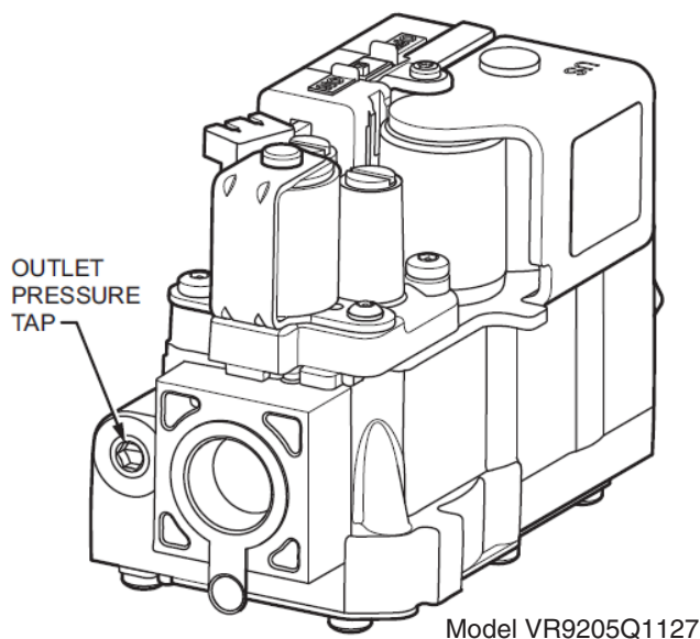
Fig. 7. Gas conversion kit: outlet
