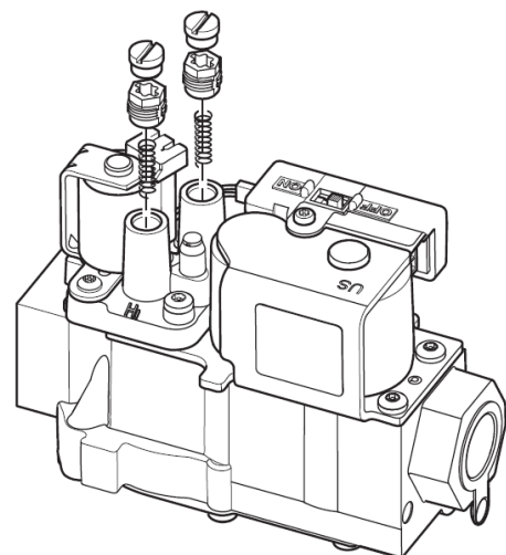
Fig. 6. Gas conversion kit.
