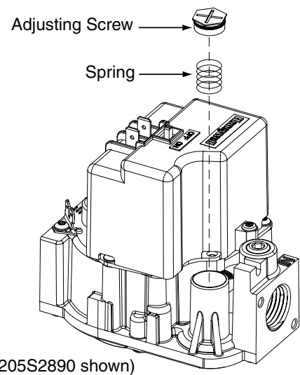
Figure 3. Pressure Regulator Spring & Adjustment Screw Removal
