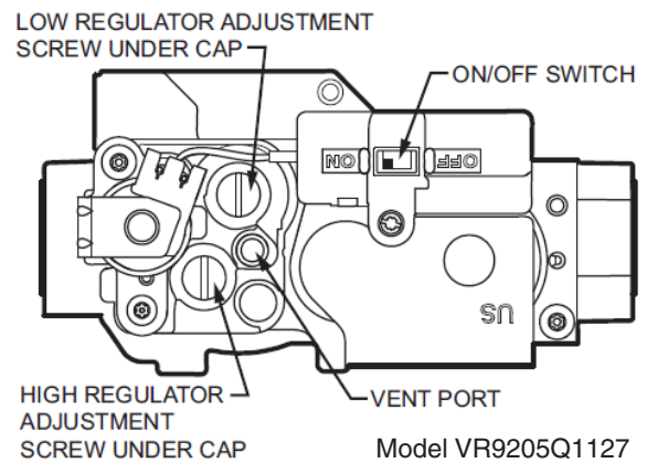
Fig. 5. Conversion kit installation regulator
