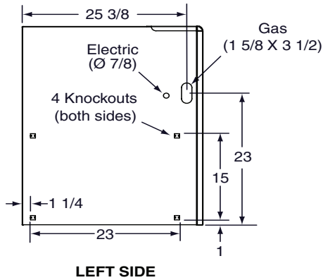
AC-N-KG7SA Single Stage Upflow/Horizontal Series
