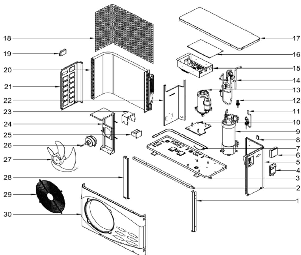
Unit Main Parts Diagram
