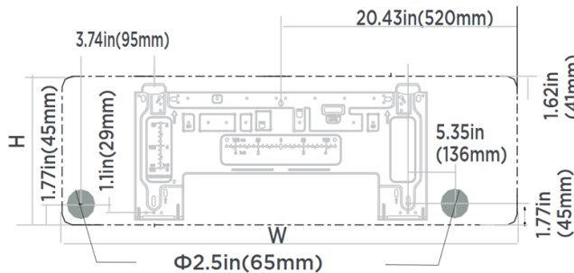
Indoor unit dimensions(WxH): 38.2in(971mm)x12.6in(321mm)
