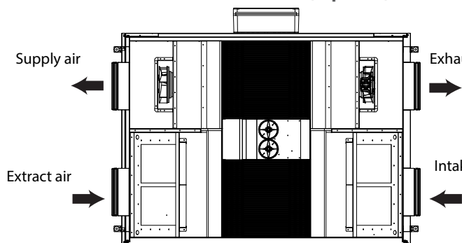
Left-sided modification (top view)
