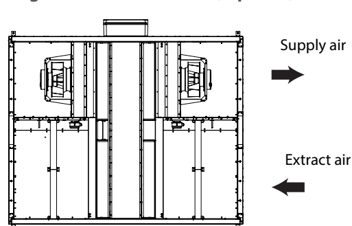
Right-sided modification (top view)
