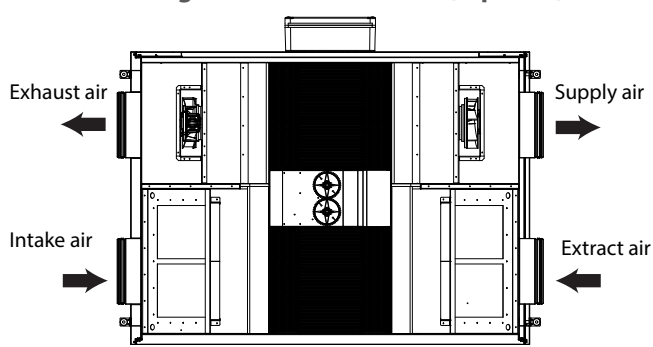
Right-sided modification (top view)
