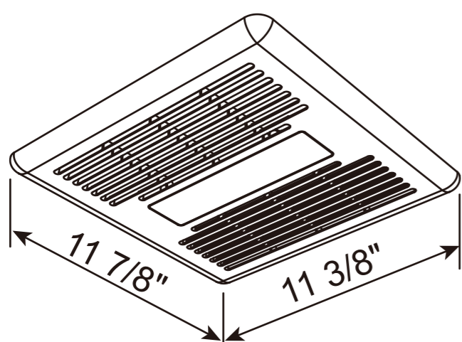
LED LIGHT GRILLE
