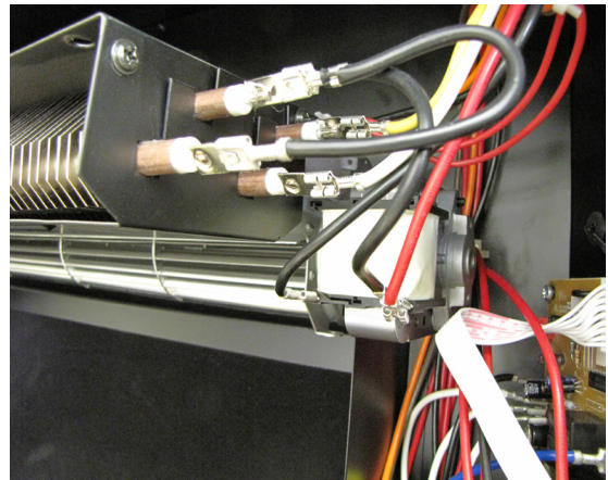
Voltage Selector Switch and Over Temperature Light (Interior View)
