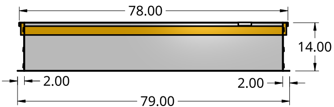
FRONT VIEW (FS)
