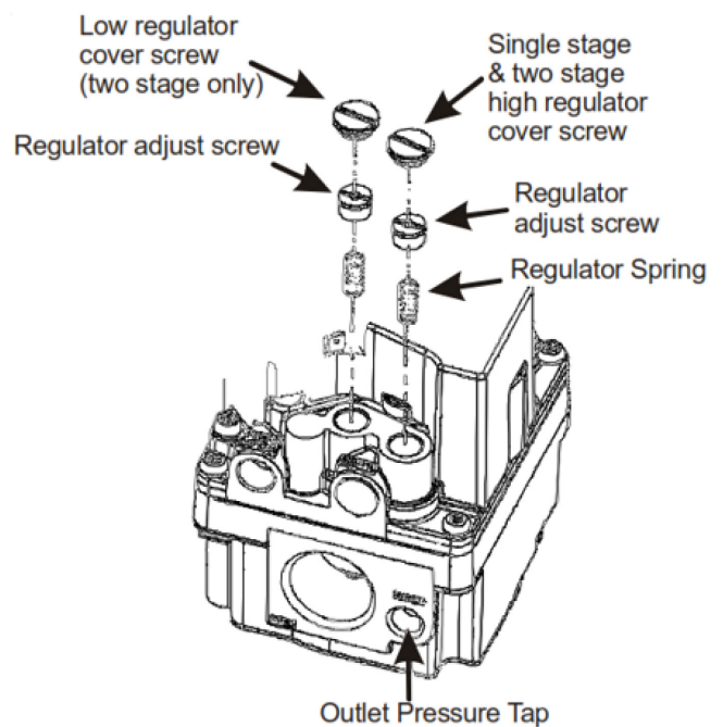
White-Rodgers 36H54 Springs and Regulator Screws Figure 4
