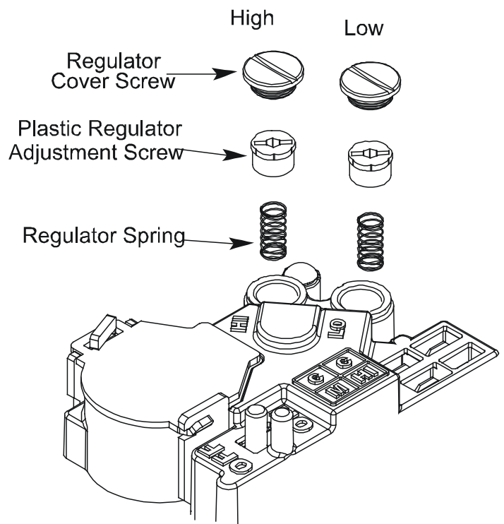
White-Rodgers 36G54 Springs and Regulator Screws Figure 3
