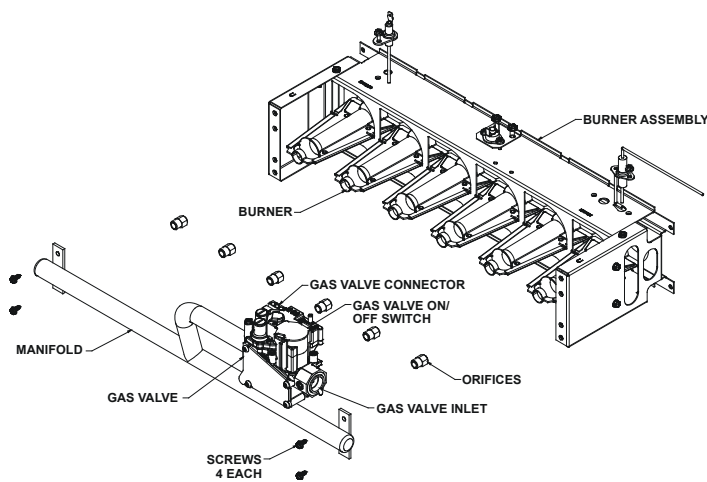
Burner Orifices Replacement Figure 2
