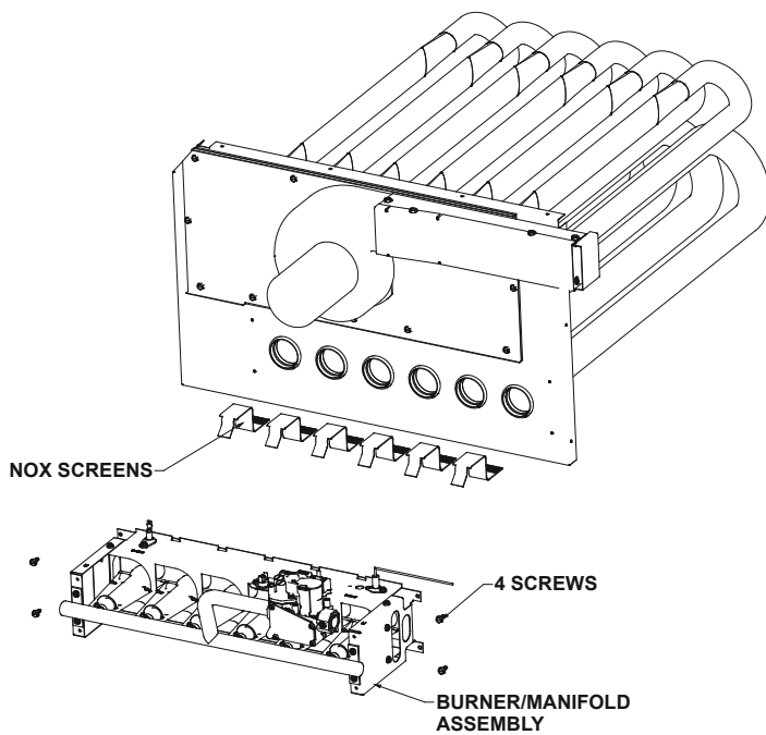
Typical NOx Screen Removal for 3 to 6 Ton Models Figure 1
