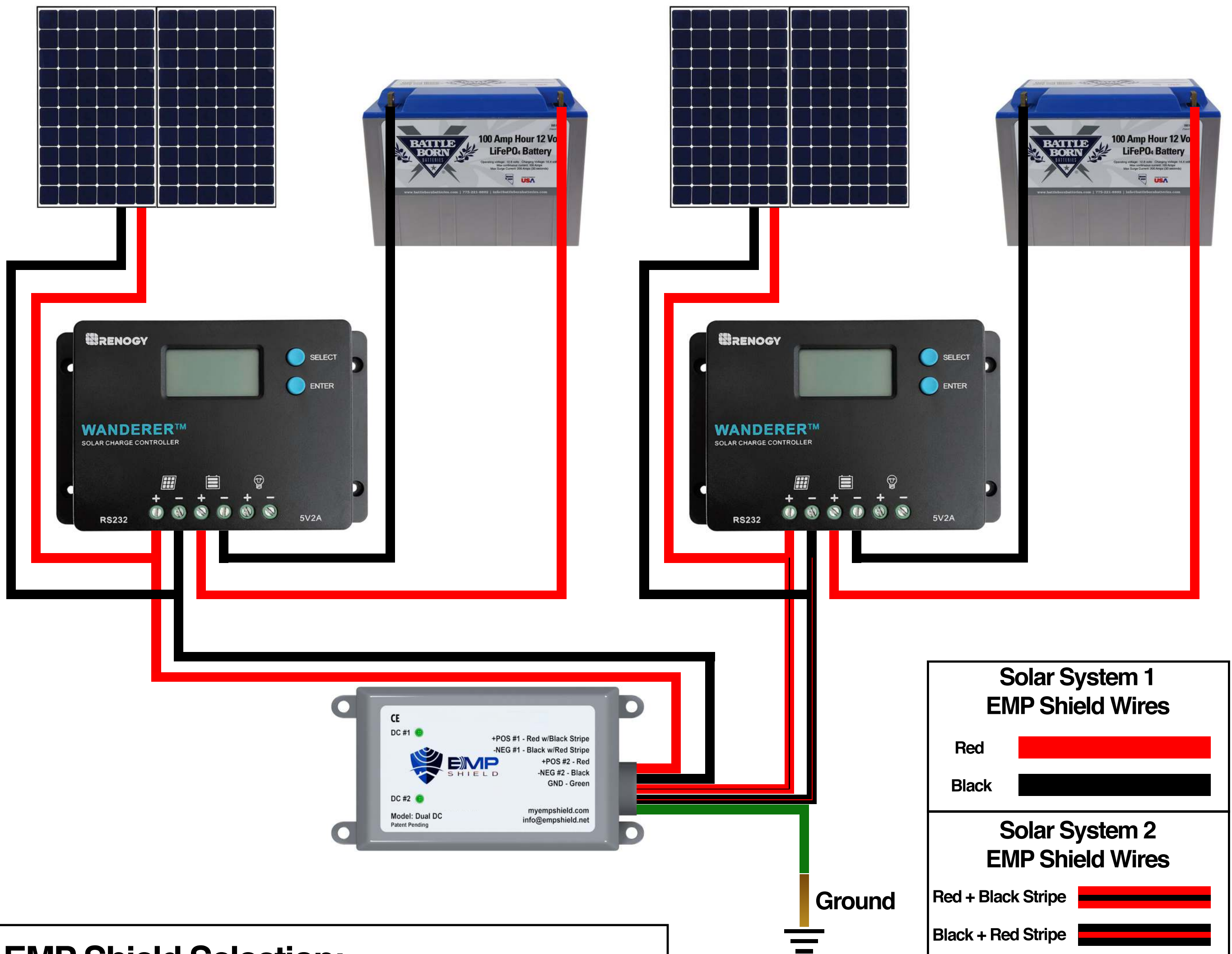
Solar System 1
