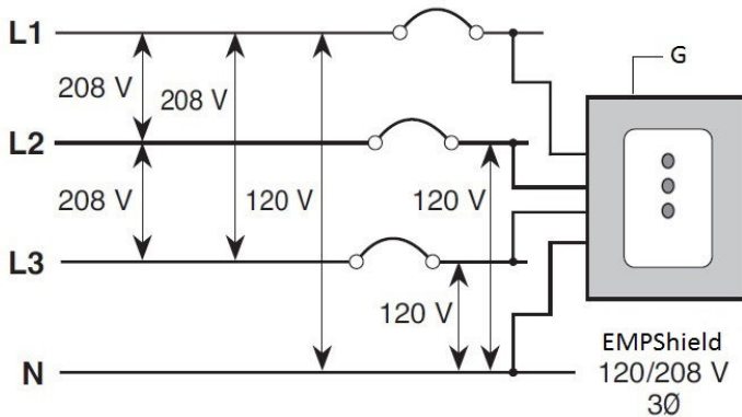
Figure 3 – Three Phase Installation
