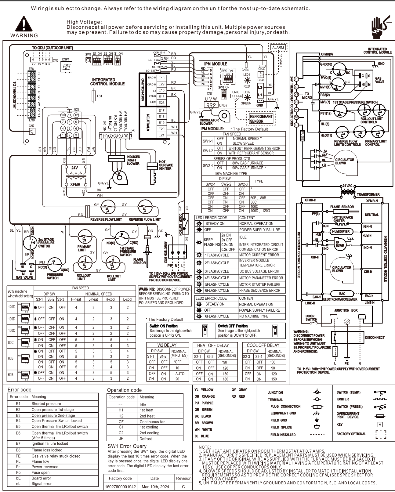
Figure 62: LNAVE060B1, LNAVE080B1, LNAVE080C1, LNAVE100C1, LNAVE120D1 96% Efficiency Gas Furnace Wiring Diagram.
