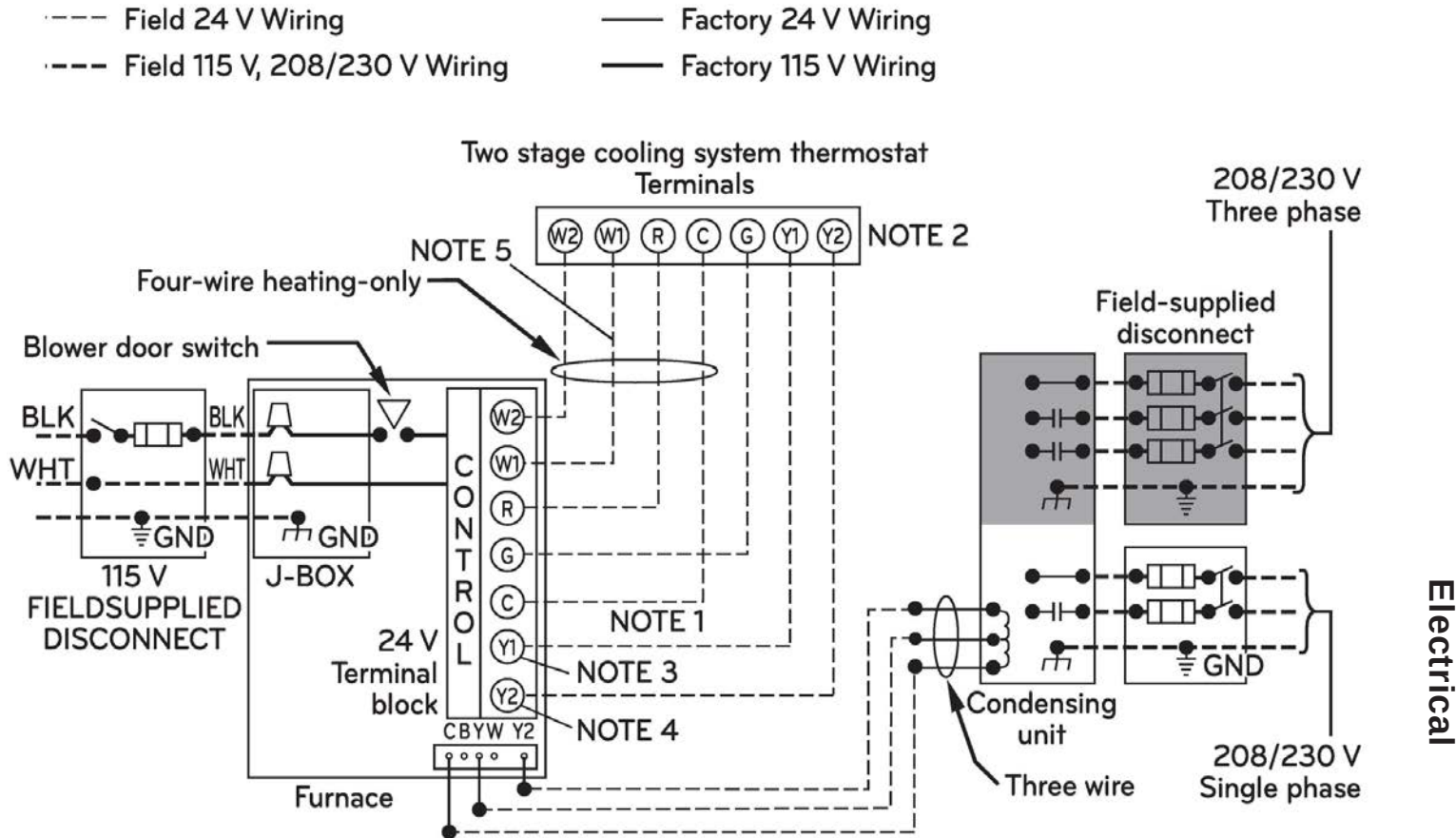
Figure 73: 96% Efficiency Gas Furnace—Heating and Cooling Application Wiring Diagram with Two-Stage Heating Thermostat.
