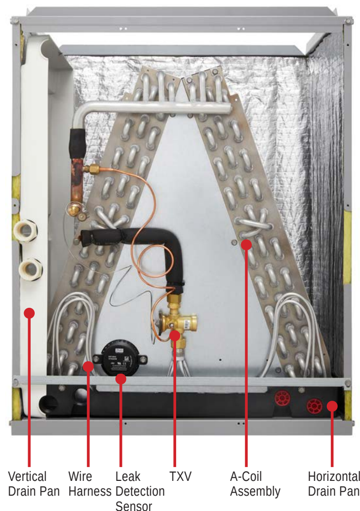
Figure 3: A-Coil Components.
