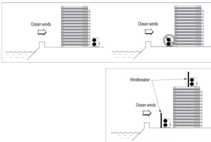
Figure 37: Oceanside Placement Using a Building as Shield, and Placement Using a Windbreaker.
