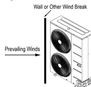
Figure 37: Oceanside Placement Using a Building as Shield, and Placement Using a Windbreaker.
