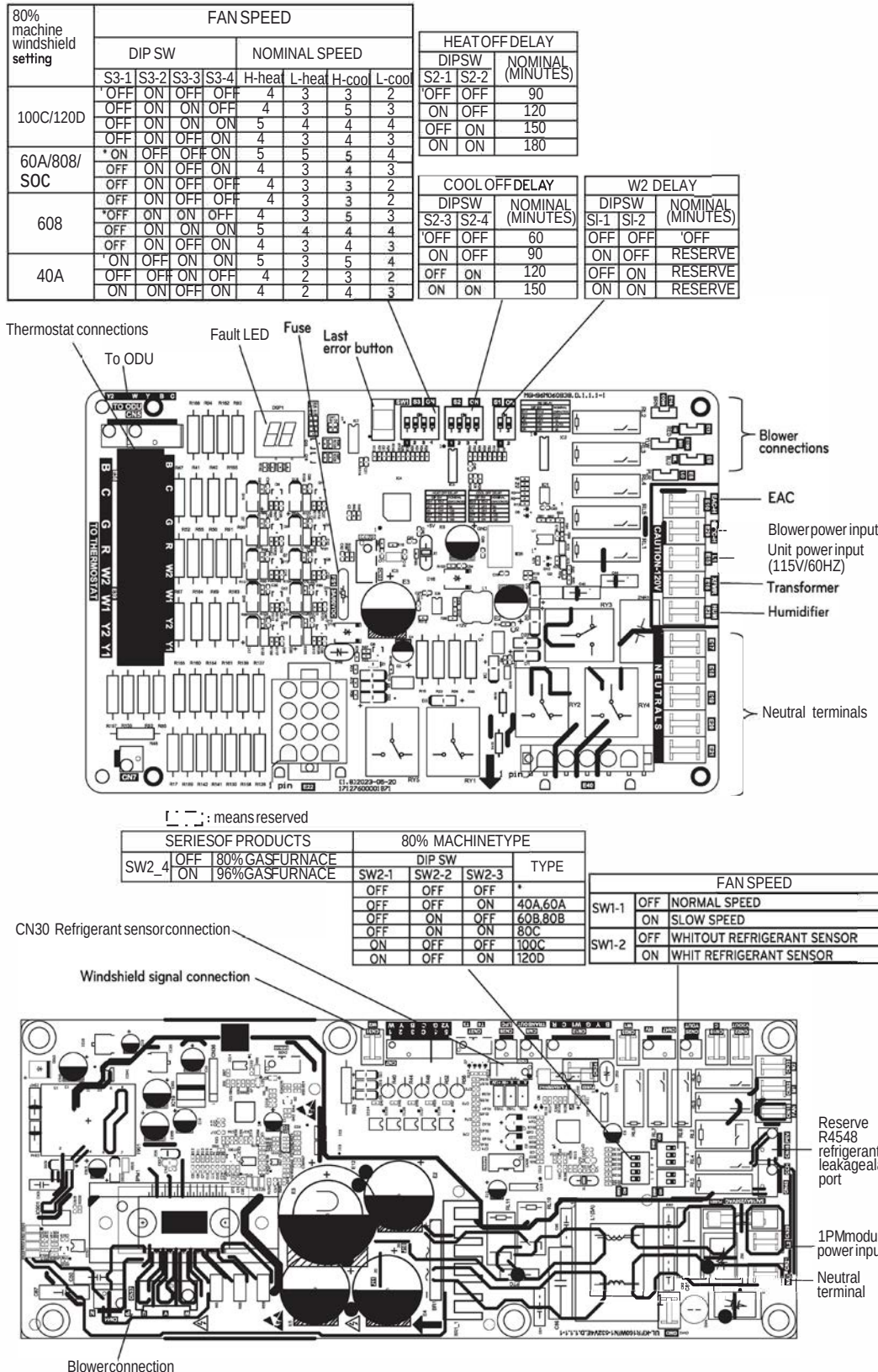
Figure 66: 80% Efficiency Gas Furnace—Furnace Control Module (For Reference).
