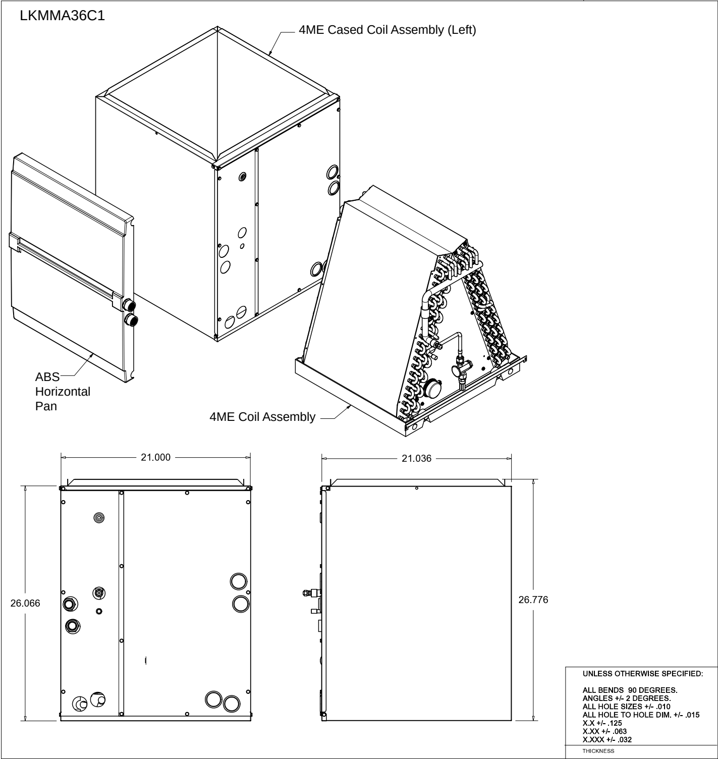
Figure 11: LKMMMA36C1 A-Coil Unit Dimensions.
