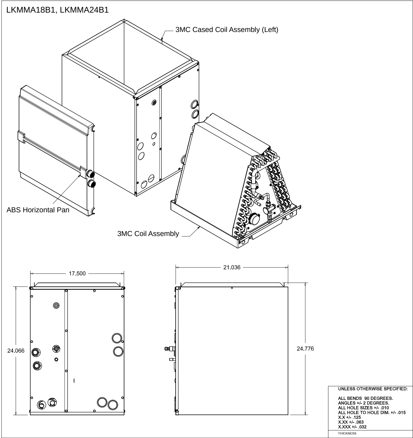
Figure 9: LKMMA18B1, LKMMA24B1 A-Coil Unit Dimensions.
