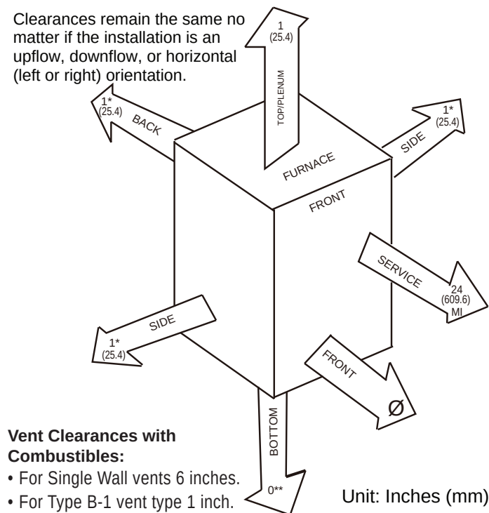
Figure 23: Clearance Requirements for 80% Efficiency Gas Furnaces.
