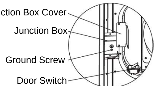
Figure 65: Junction Box.
