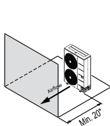
Figure 30: Proper Outdoor Unit Placement and Clearances When There Are Obstacles on the Discharge Side.
