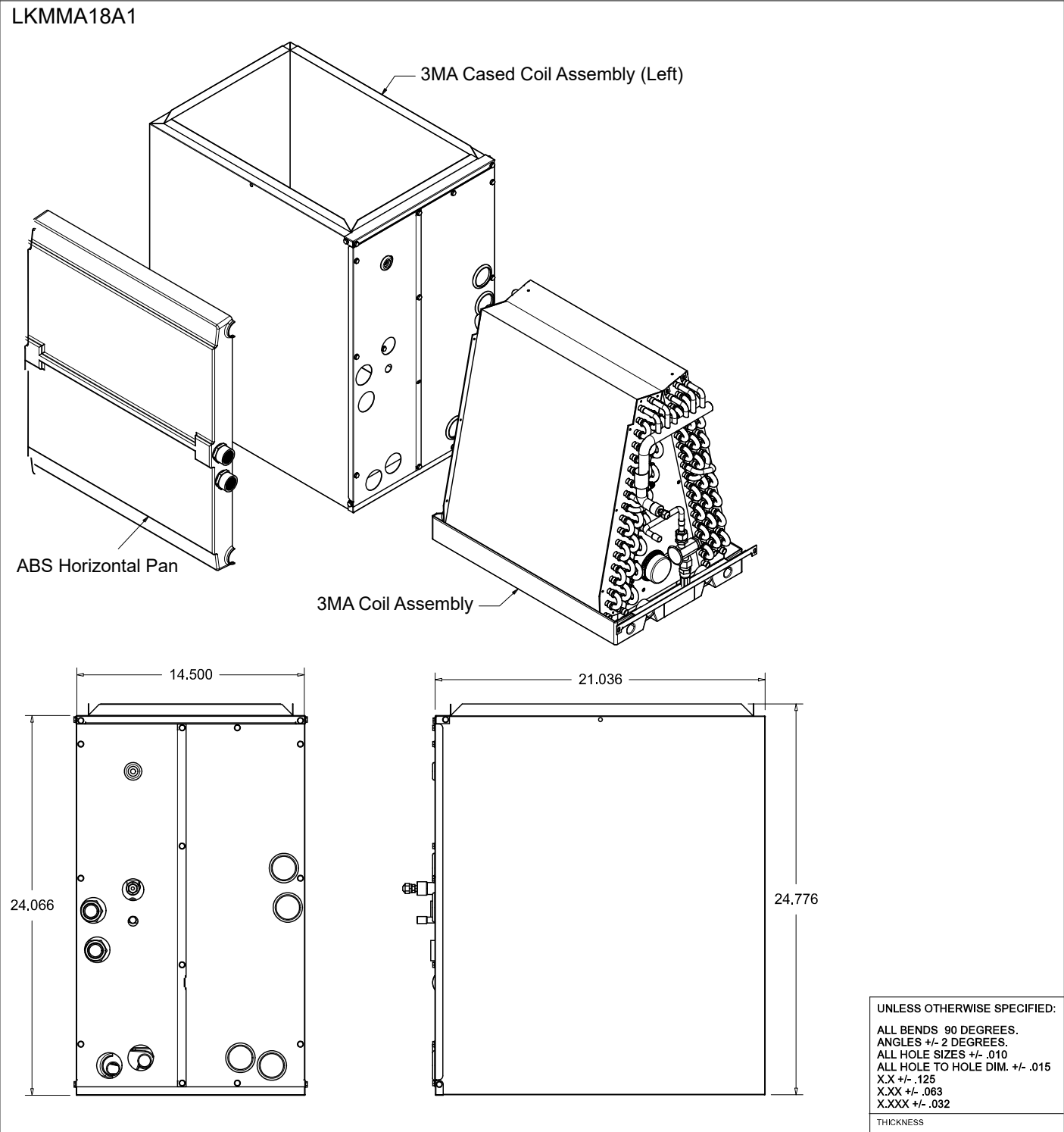
Figure 9: LKMMA18A1 A-Coil Unit Dimensions.
