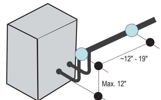
Figure 45: Pipe Support at A-Coil Unit.
