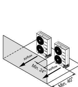
Figure 30: Proper Outdoor Unit Placement and Clearances When There Are Obstacles on the Discharge Side.
