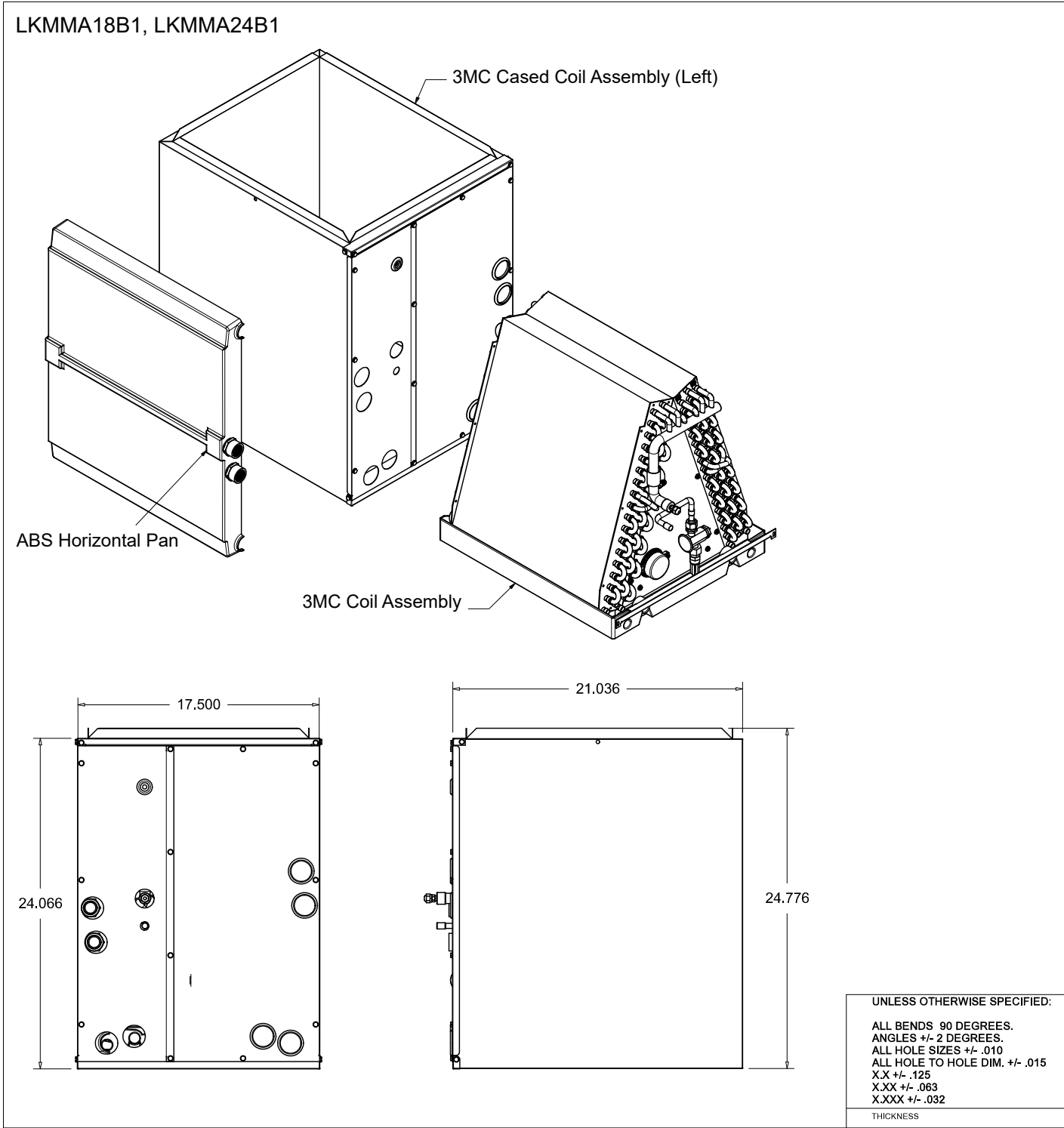
Figure 10: LKMMA18B1, LKMMA24B1 A-Coil Unit Dimensions.
