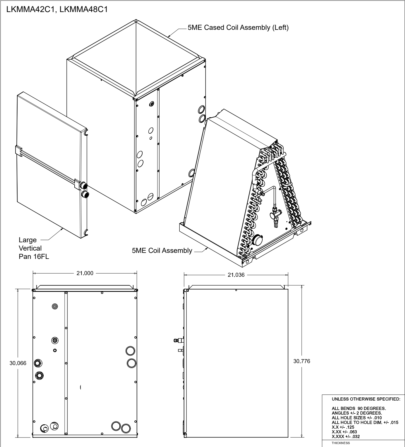
Figure 13: LKMMA42C1, LKMMA48C1 A-Coil Unit Dimensions.
