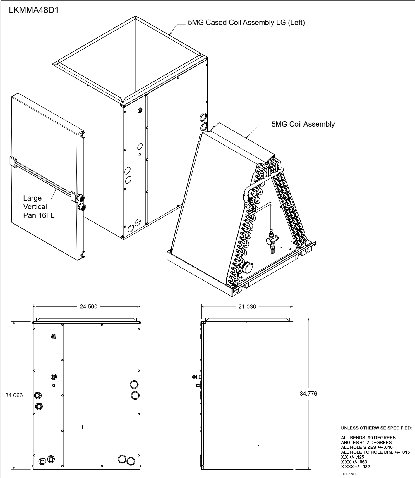
Figure 14: LKMMMA48D1 A-Coil Unit Dimensions.
