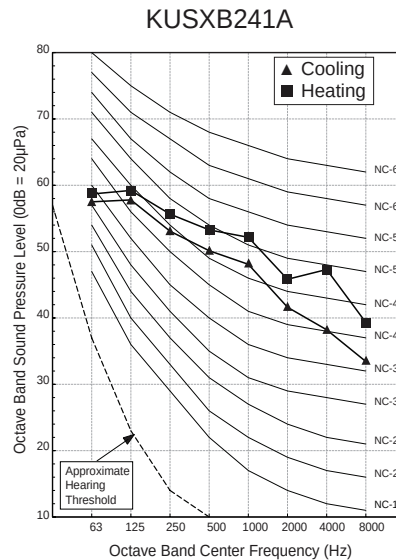
Figure 16: R32 Standard Single-Zone Systems - A-Coil Outdoor Unit Sound Pressure Level Diagrams.
