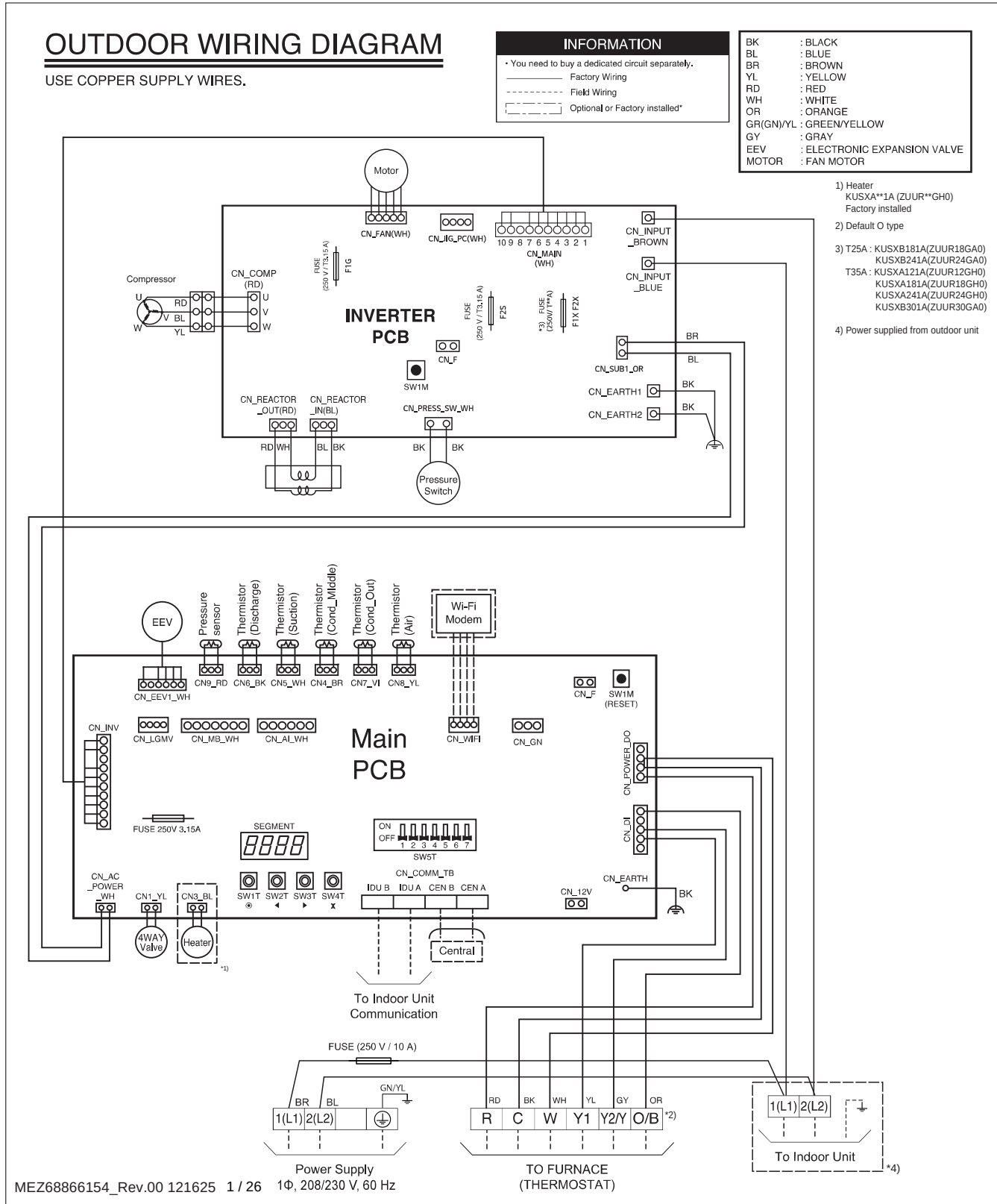
Figure 47: KUSXB181A, KUSXB241A, KUSXB301A Outdoor Unit Wiring Diagram.
