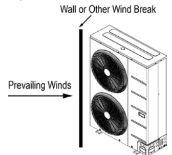
Figure 25: Wind Break.
