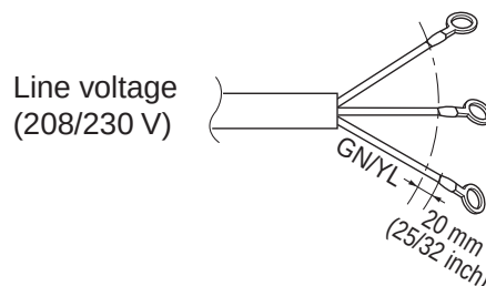
Figure 52: Power Wiring Example.
