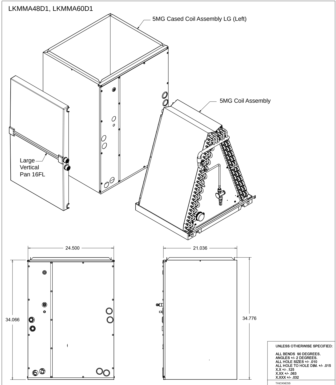
Figure 14: LKMMMA48D1, LKMMMA60D1 A-Coil Unit Dimensions.
