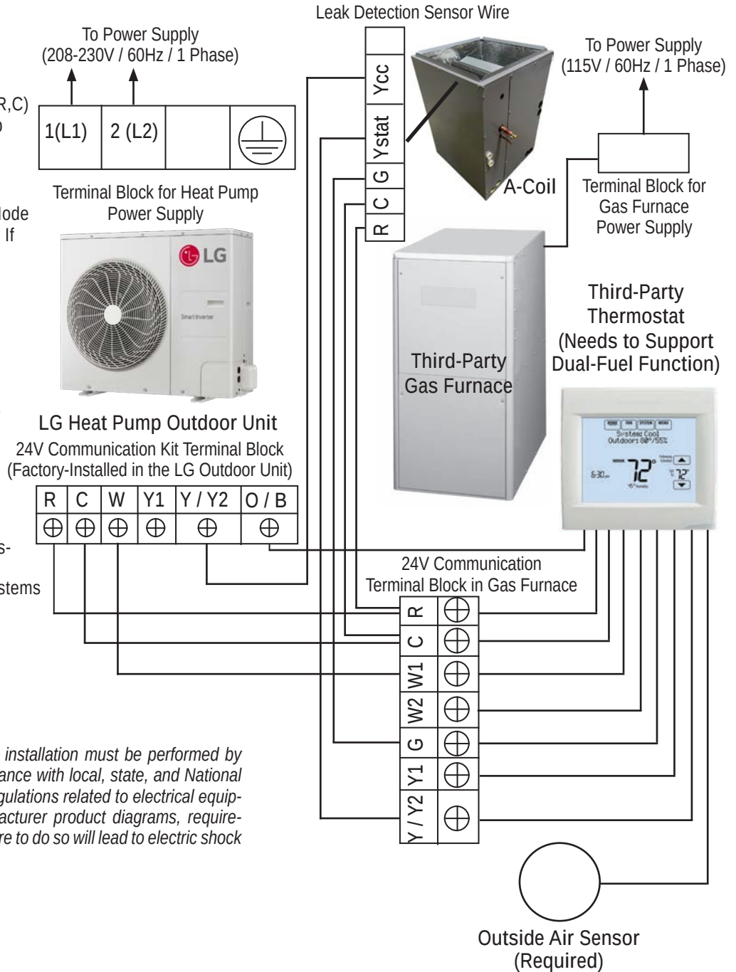
Figure 53: Detailed One-Stage Wiring Diagram (For Illustrative Purposes Only).
