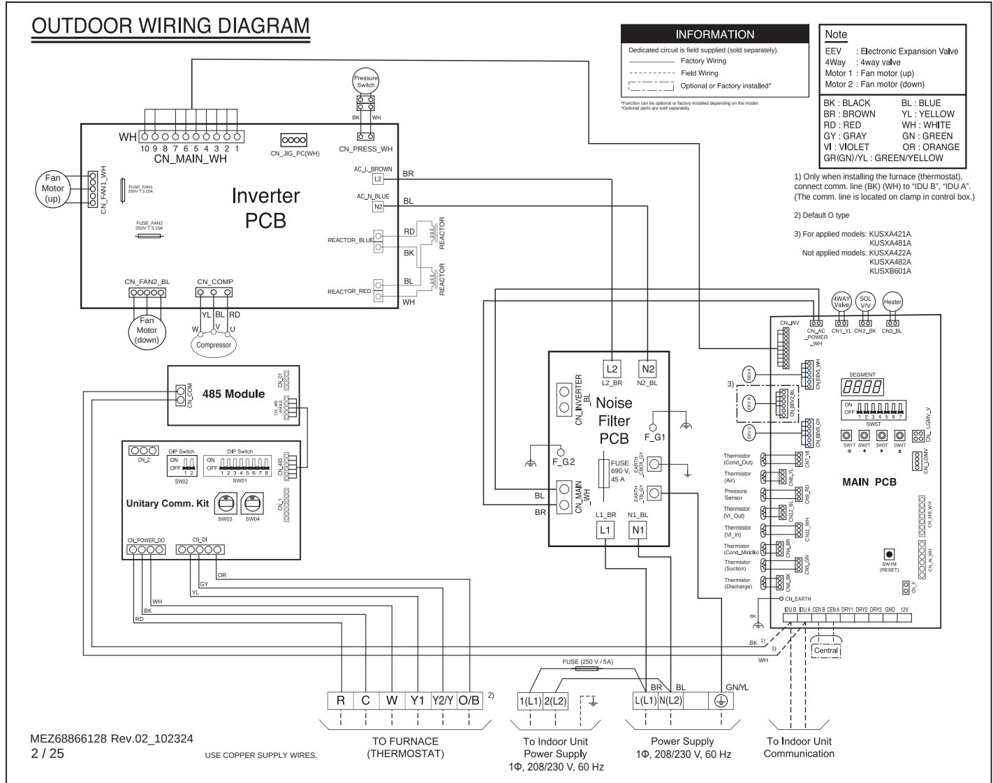
Figure 50: KUSXB601A Outdoor Unit Wiring Diagram.
