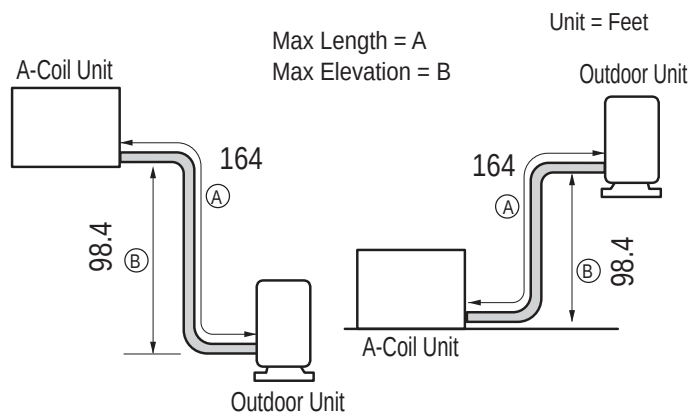
Figure 39: Typical KSSMB18AA ~ KSSMB30BA System Layout.
