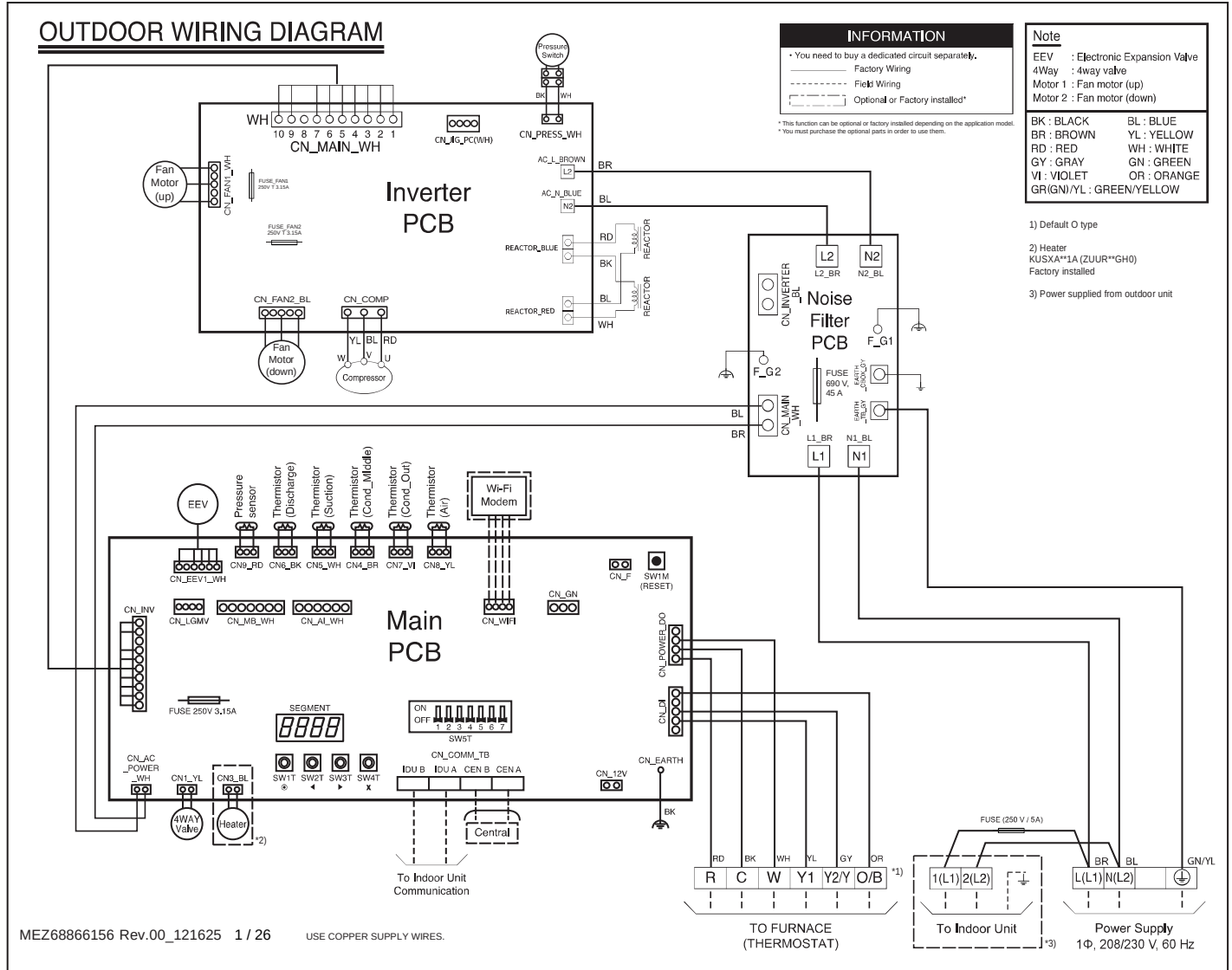
Figure 49: KUSXB421A, KUSXB481A Outdoor Unit Wiring Diagram.
