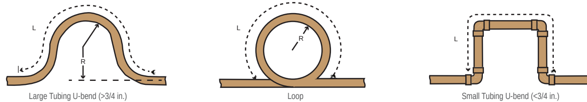
Figure 41: Coiled Expansion Loops and Offsets (Plan View).
