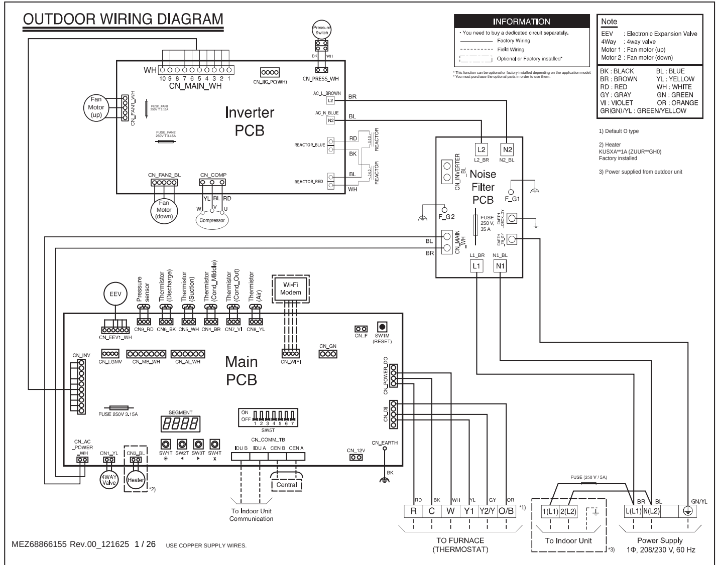
Figure 48: KUSXB361A Outdoor Unit Wiring Diagram.
