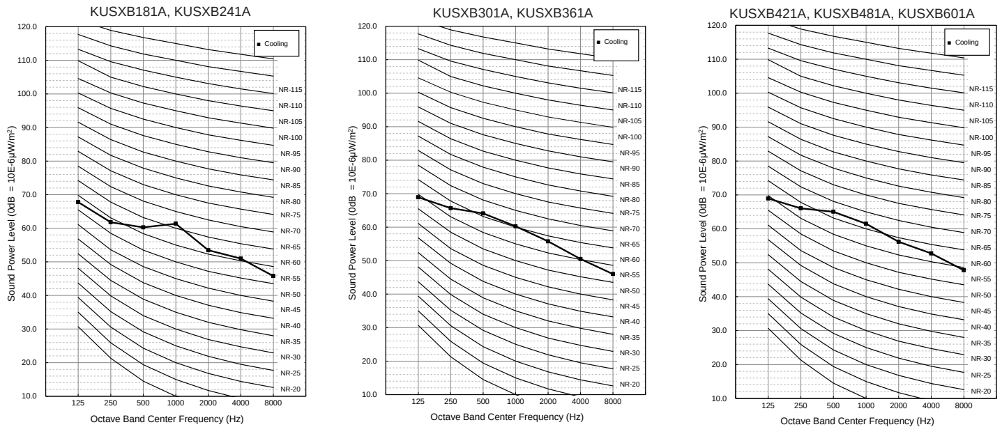
Figure 17: R32 Standard Single-Zone Systems - A-Coil Outdoor Unit Sound Power Level Diagrams.
