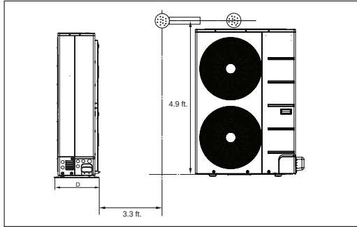
Figure 15: R32 Standard Single-Zone Systems - A-Coil Outdoor Unit Sound Pressure Level Measurement Location (For Illustrative Purposes Only; Appearance Depends on Model).
