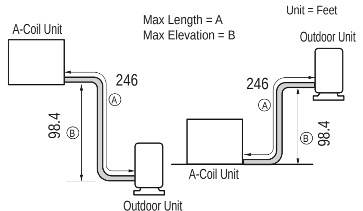
Figure 40: Typical KSSMB36BA ~ KSSMB60DA System Layout.
