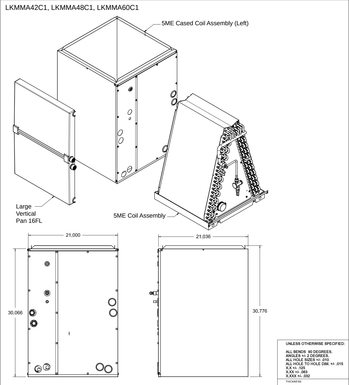
Figure 13: LKMMA42C1, LKMMA48C1, LKMMA60C1 A-Coil Unit Dimensions.
