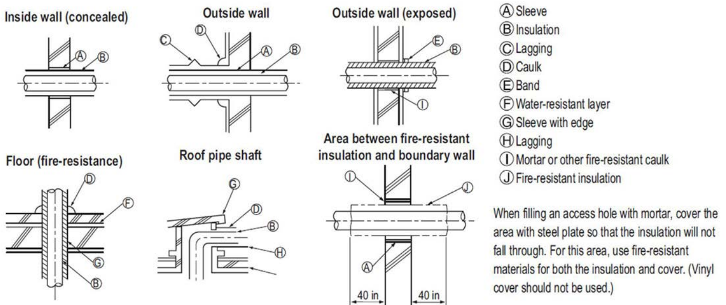
Figure 46: Pipe Sleeve Options.
