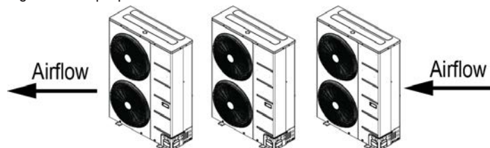
Figure 28: Improper Outdoor Unit Placement.
