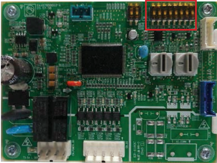
Figure 56: SW-01 DIP Switch Heat Pump Communication Kit Default Setting (All Off).
