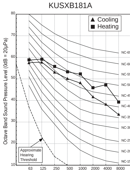
Figure 16: R32 Standard Single-Zone Systems - A-Coil Outdoor Unit Sound Pressure Level Diagrams.
