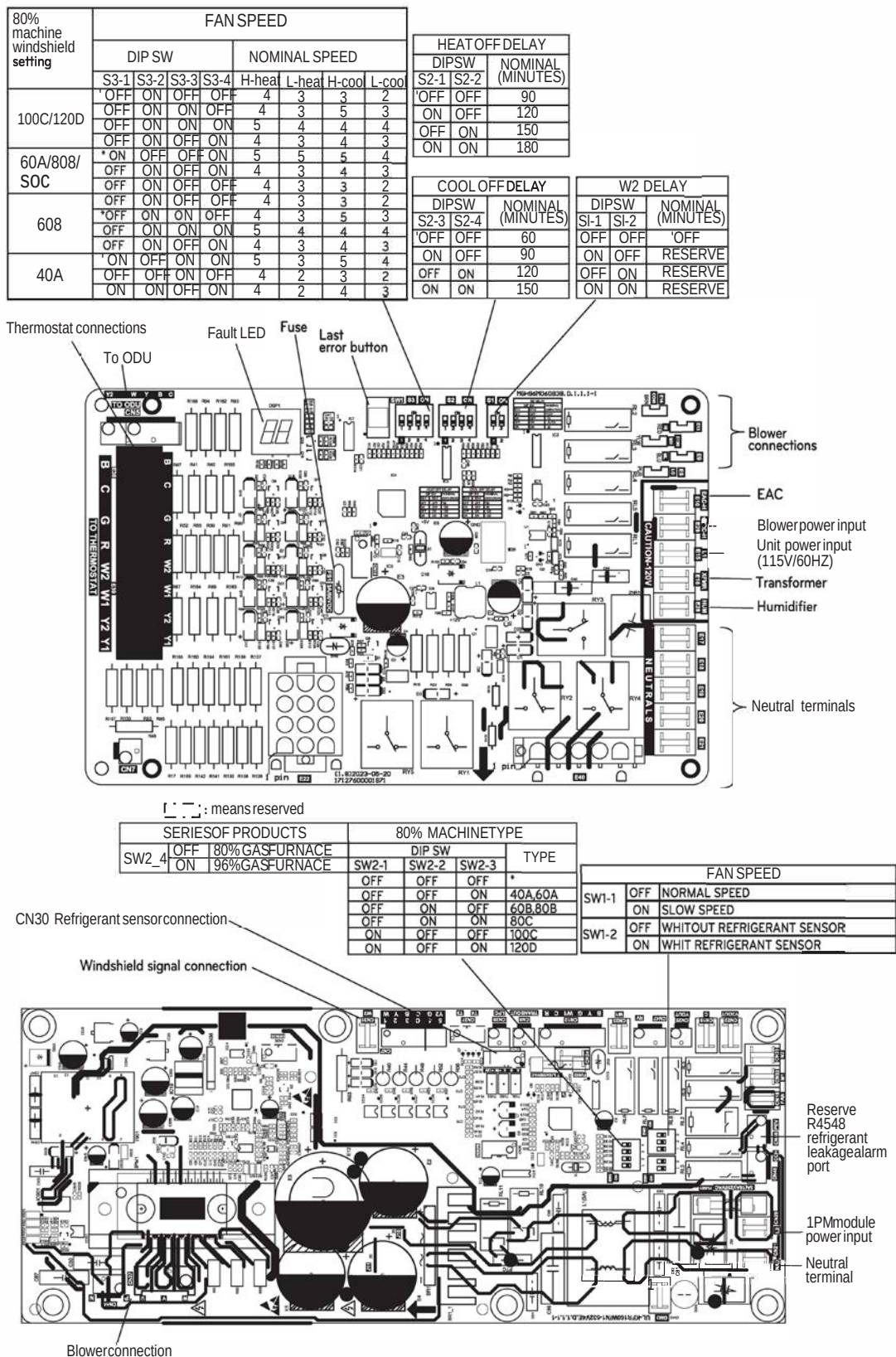
Figure 68: 80% Efficiency Gas Furnace—Furnace Control Module (For Reference).
