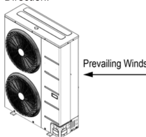
Figure 35: Prevailing Wind Direction.
