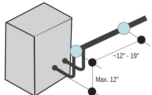
Figure 57: Pipe Support at A-Coil Unit.
