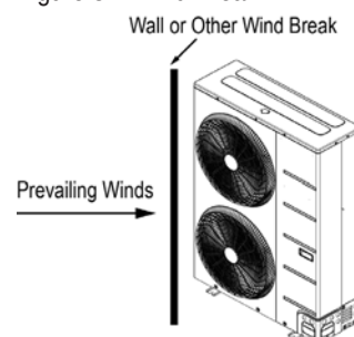
Figure 37: Wind Break.
