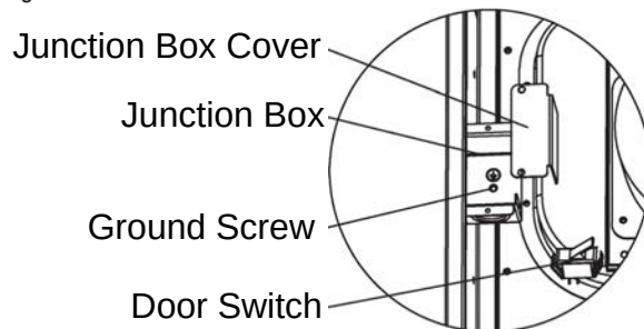
Figure 67: Junction Box.
