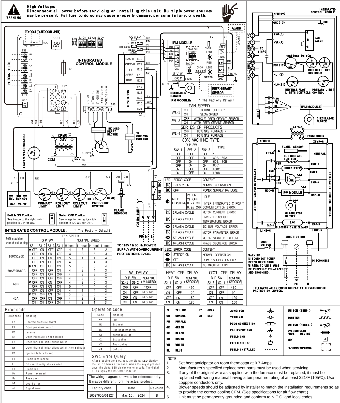
Figure 63: LNAEA040A1, LNAEA060B1, LNAEA080C1, LNAEA100C1, LNAEA120D1 80% Efficiency Gas Furnace Wiring Diagram.
