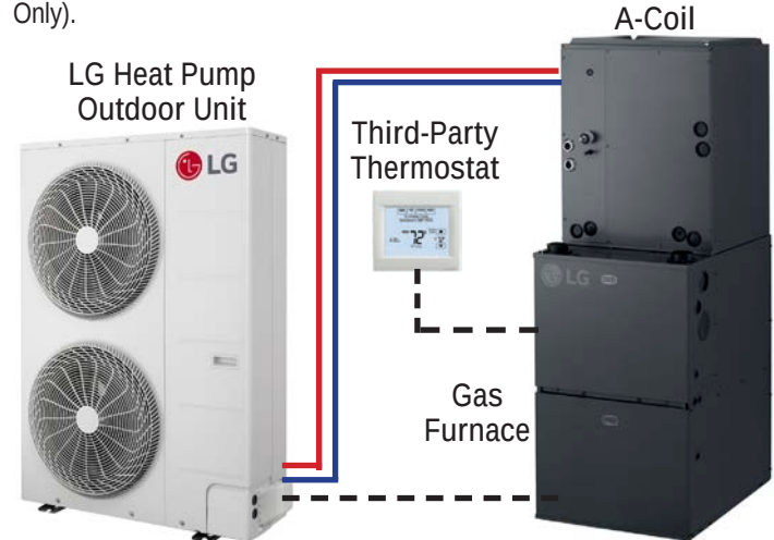
Figure 2: R32 Standard Single Zone Systems - A-Coil (KSSS-B361A060-B1 to KSSSB601A100-120-D1; For Illustrative Purposes Only).
