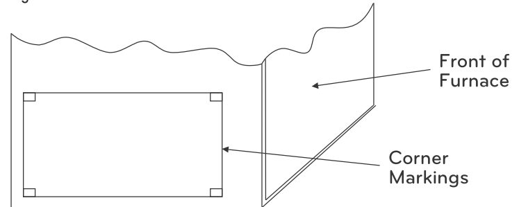
Figure 28: Side Return Cut-Out Marks.
