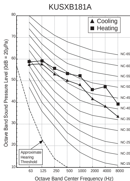
Figure 18: R32 Standard Single-Zone Systems - A-Coil /Gas Furnace Outdoor Unit Sound Pressure Level Diagrams.
