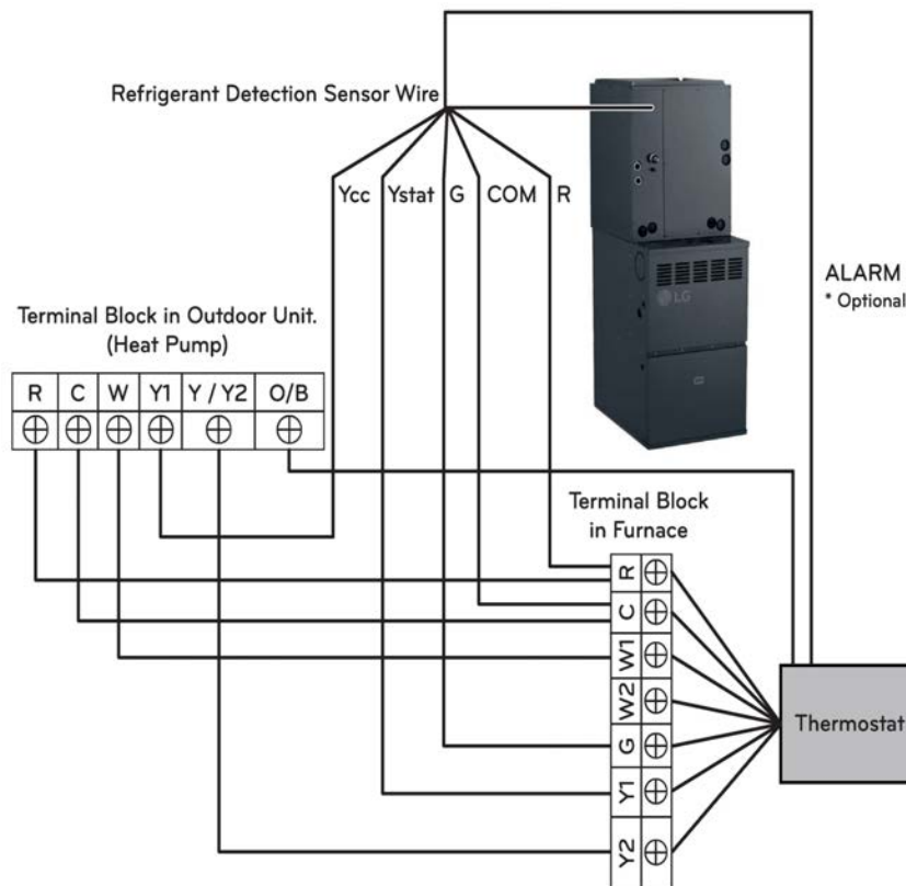
Figure 74: 96% Efficiency Gas Furnace—Wiring Diagram with Dual Fuel Two-Stage Cooling, Four-Stage Heating Thermostat.
