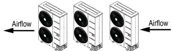
Figure 40: Improper Outdoor Unit Placement.
