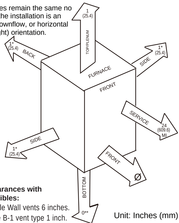
Figure 24: Clearance Requirements for 80% Efficiency Gas Furnaces.
