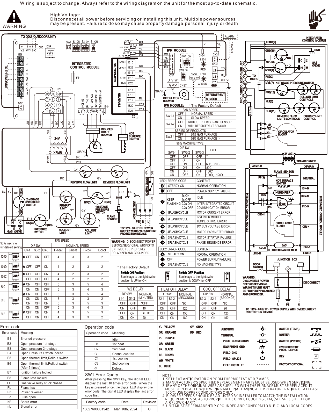
Figure 64: LNAVE060B1, LNAVE080B1, LNAVE080C1, LNAVE100C1, LNAVE120D1 96% Efficiency Gas Furnace Wiring Diagram.
