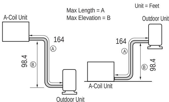
Figure 51: Typical 18k ~ 30k System Layout.
