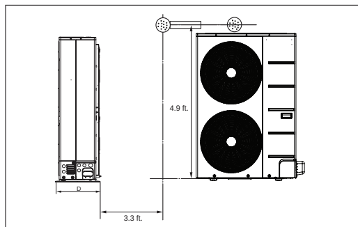
Figure 17: R32 Standard Single-Zone Systems - A-Coil + Gas Furnace Outdoor Unit Sound Pressure Level Measurement Location (For Illustrative Purposes Only; Appearance Depends on Model).
