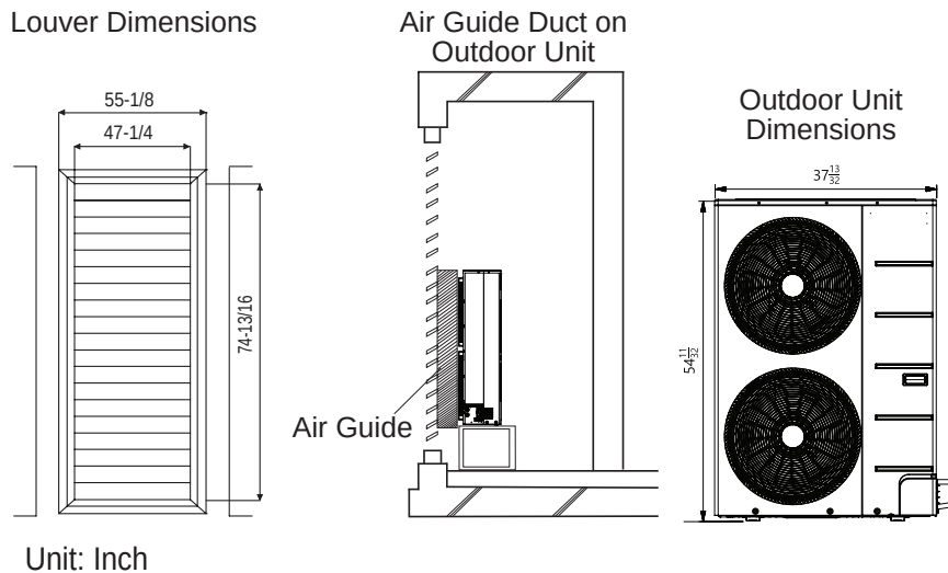
Figure 46: Example of Installing Outdoor Unit Indoors.
