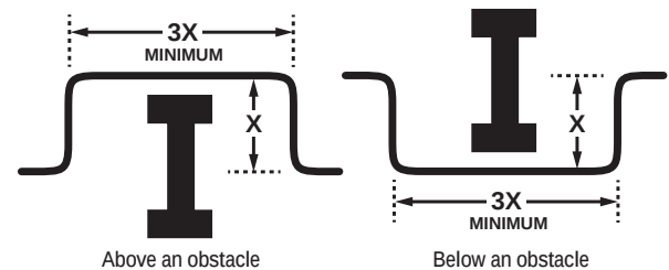
Figure 54: Installing Piping Above and Below an Obstacle.
