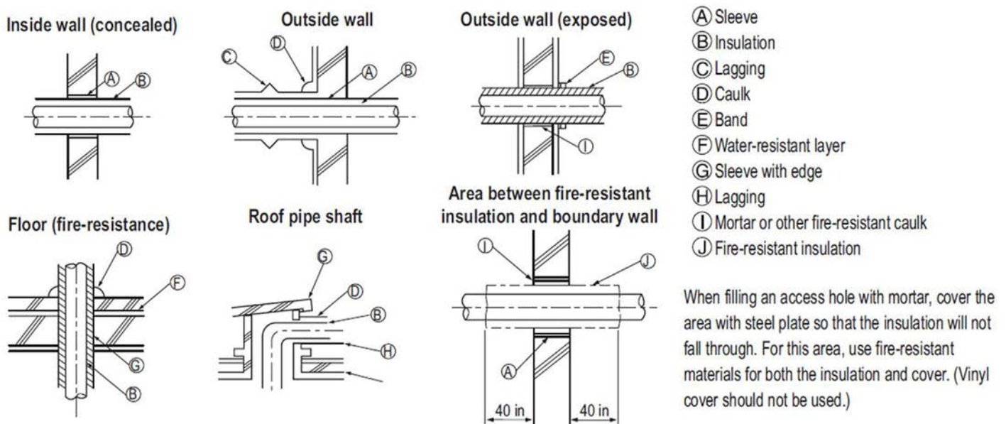
Figure 58: Pipe Sleeve Options.
