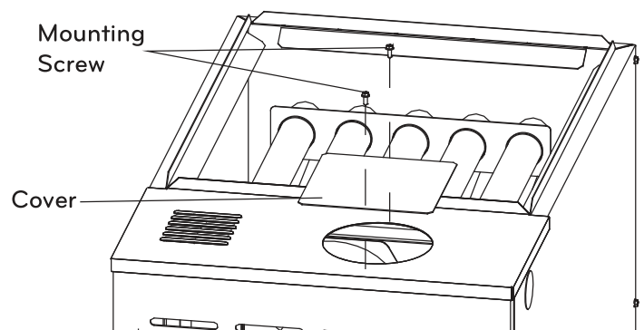
Figure 30: Cover the Hole in the Top When the Combustion Air Inducer is Rotated.
