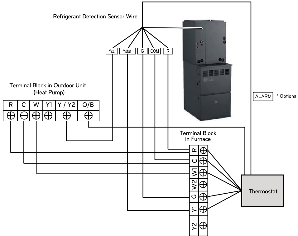
Figure 74: 96% Efficiency Gas Furnace—Wiring Diagram with Dual Fuel Two-Stage Cooling, Four-Stage Heating Thermostat.
