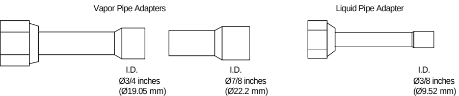
Figure 50: Adapters for A-Coil Piping.
