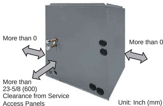
Figure 21: Example of an Upflow (Vertical) Installation.
