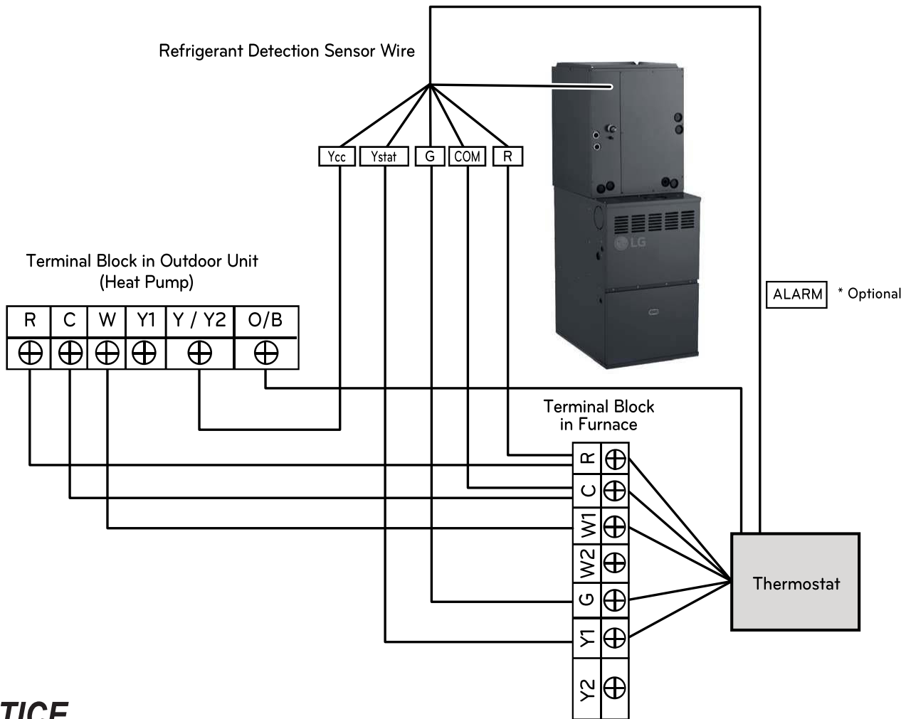
Figure 71: 80% Efficiency Gas Furnace—Wiring Diagram with Dual Fuel One-Stage Cooling, Two-Stage Heating Thermostat.
