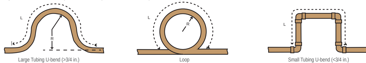
Figure 53: Coiled Expansion Loops and Offsets (Plan View).
