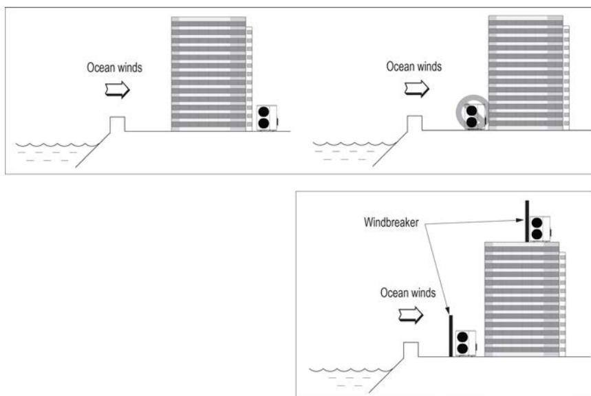
Figure 38: Oceanside Placement Using a Building as Shield, and Placement Using a Windbreaker.
