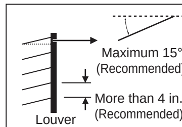
Figure 44: Louver Recommendations.
