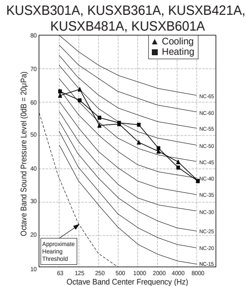
Figure 18: R32 Standard Single-Zone Systems - A-Coil /Gas Furnace Outdoor Unit Sound Pressure Level Diagrams.
