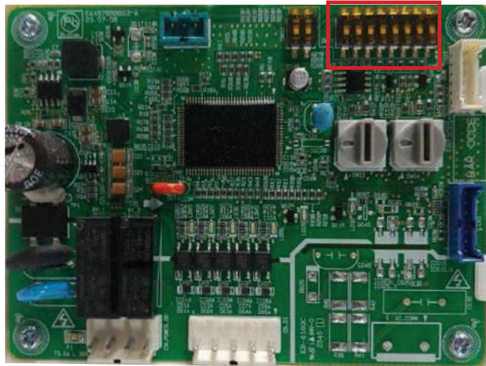
Figure 77: SW-01 DIP Switch Heat Pump Communication Kit Default Setting (All Off).
