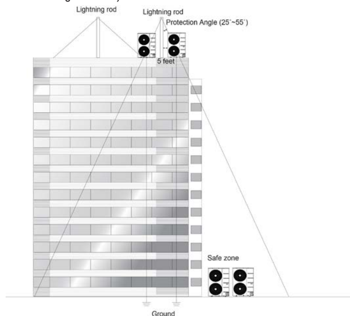
Figure 34: Lightning Protection Diagram (Outdoor Unit Appearances Differ According to Model).
