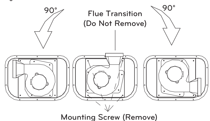
Figure 30: Cover the Hole in the Top When the Combustion Air Inducer is Rotated.
