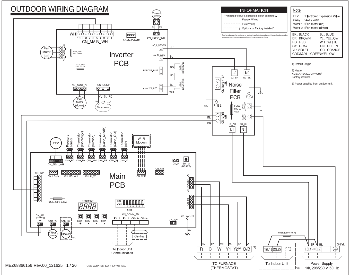
Figure 61: KUSXB421A, KUSXB481A Outdoor Unit Wiring Diagram.
