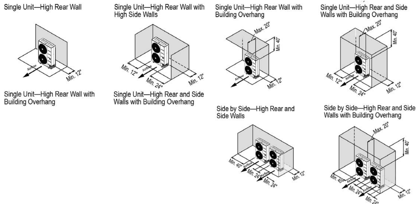
Figure 41: Proper Outdoor Unit Placement and Clearances When There Are Obstacles on the Suction Side.
