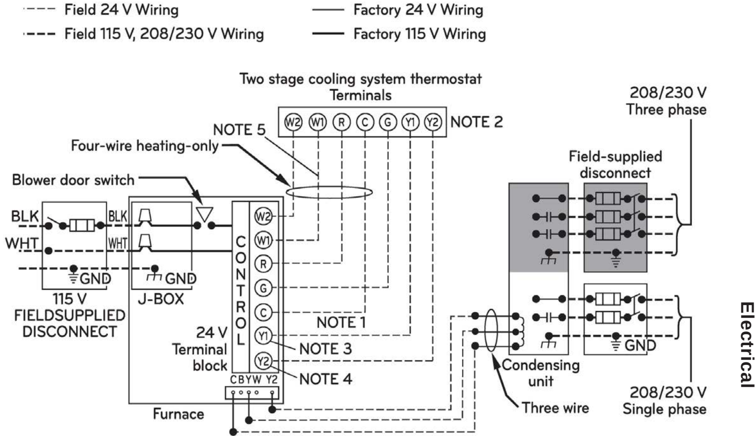
Figure 75: 96% Efficiency Gas Furnace—Heating and Cooling Application Wiring Diagram with Two-Stage Heating Thermostat.
