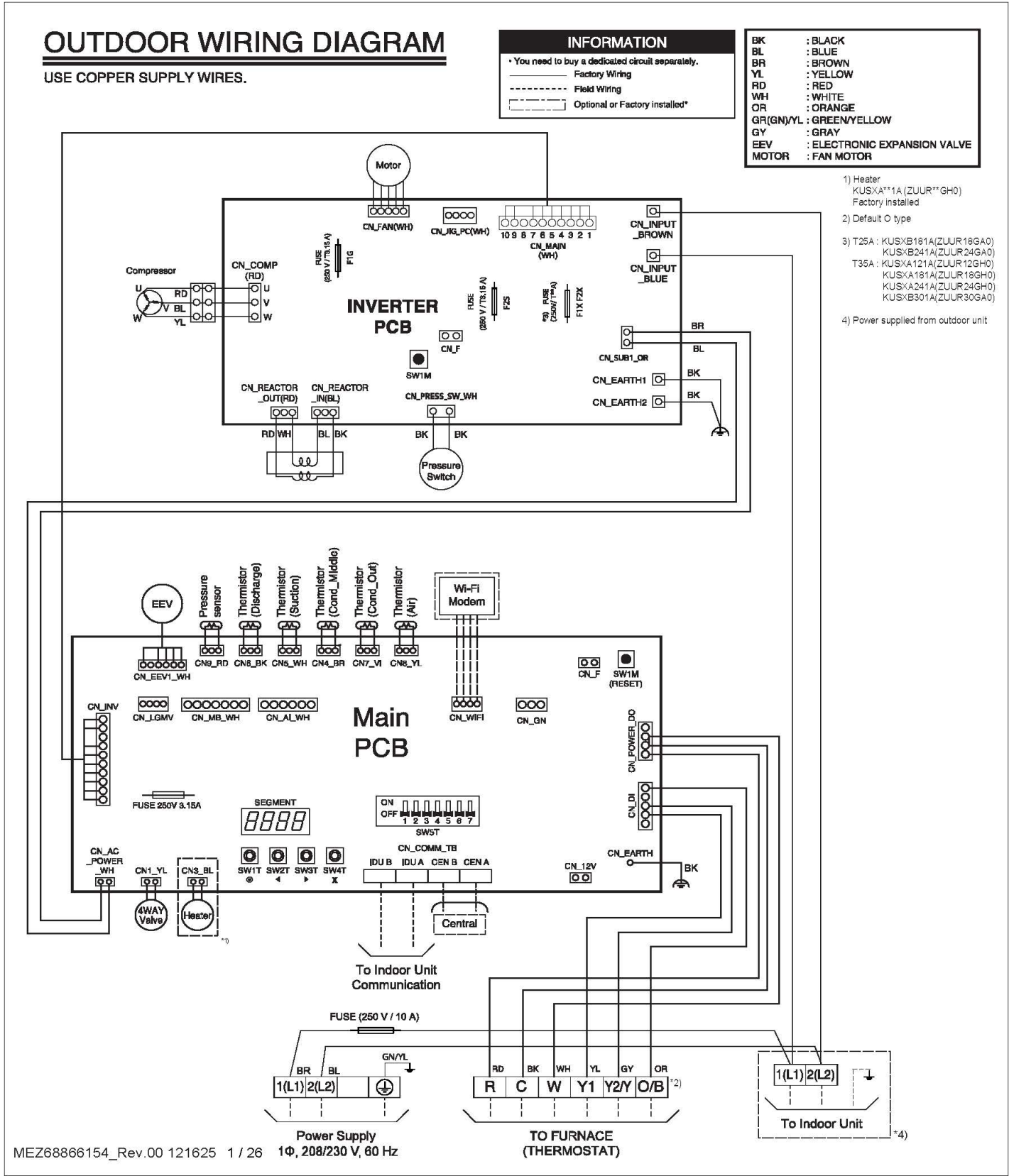
Figure 59: KUSXB181A, KUSXB241A, KUSXB301A Outdoor Unit Wiring Diagram.
