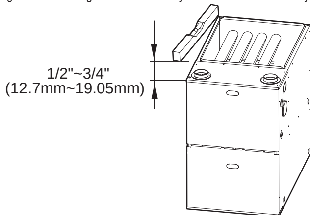
Figure 26: Installing the 96% Efficiency Gas Furnace Horizontally.
