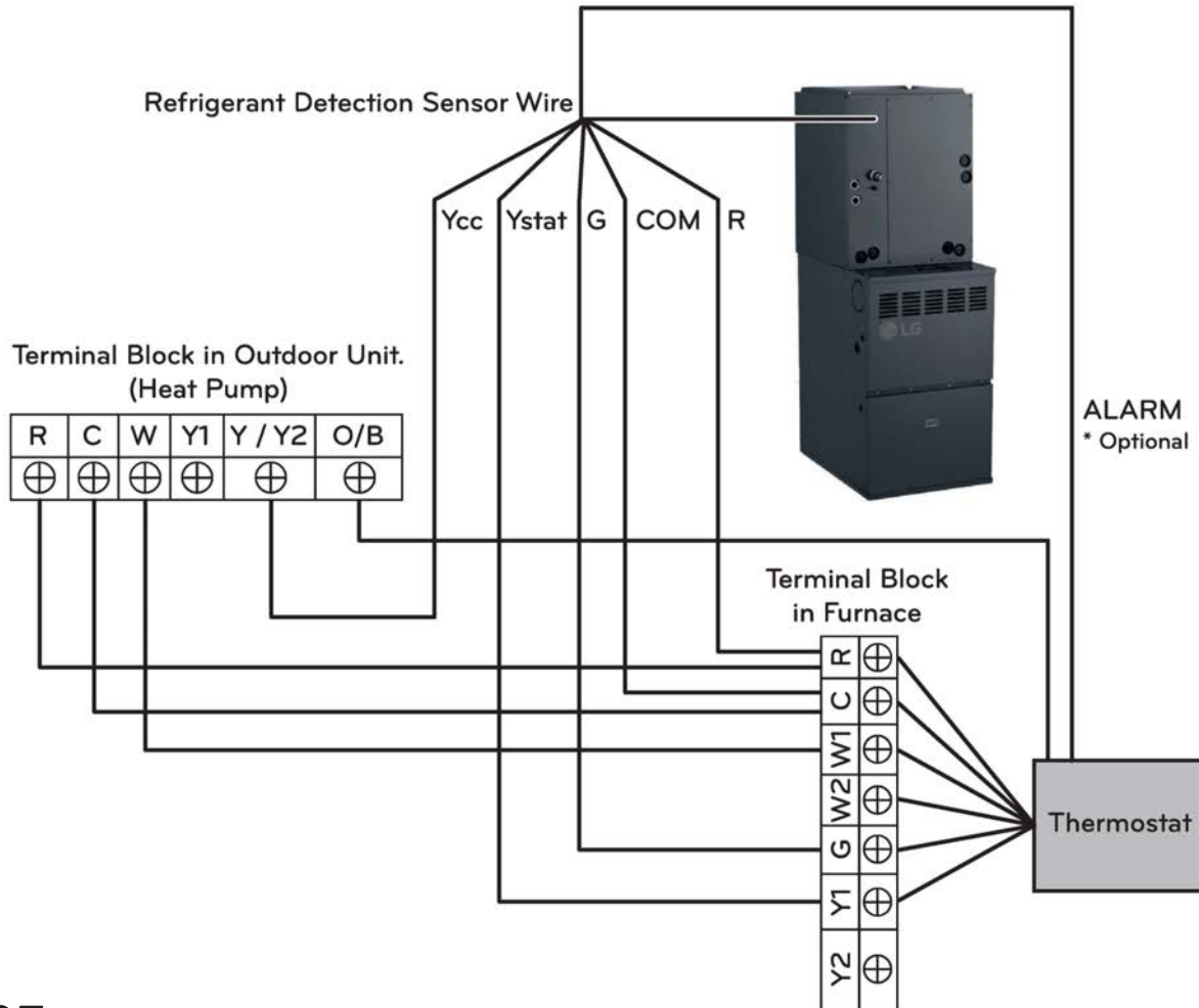
Figure 72: 96% Efficiency Gas Furnace—Wiring Diagram with Dual Fuel One-Stage Cooling, Three-Stage Heating Thermostat.
