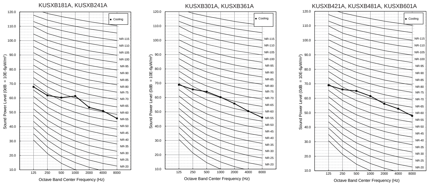
Figure 19: R32 Standard Singe-Zone Systems - A-Coil + Gas Furnace Outdoor Unit Sound Power Level Diagrams.
