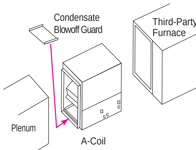
Figure 23: Horizontal Installation with Condensate Blowoff Guard.
