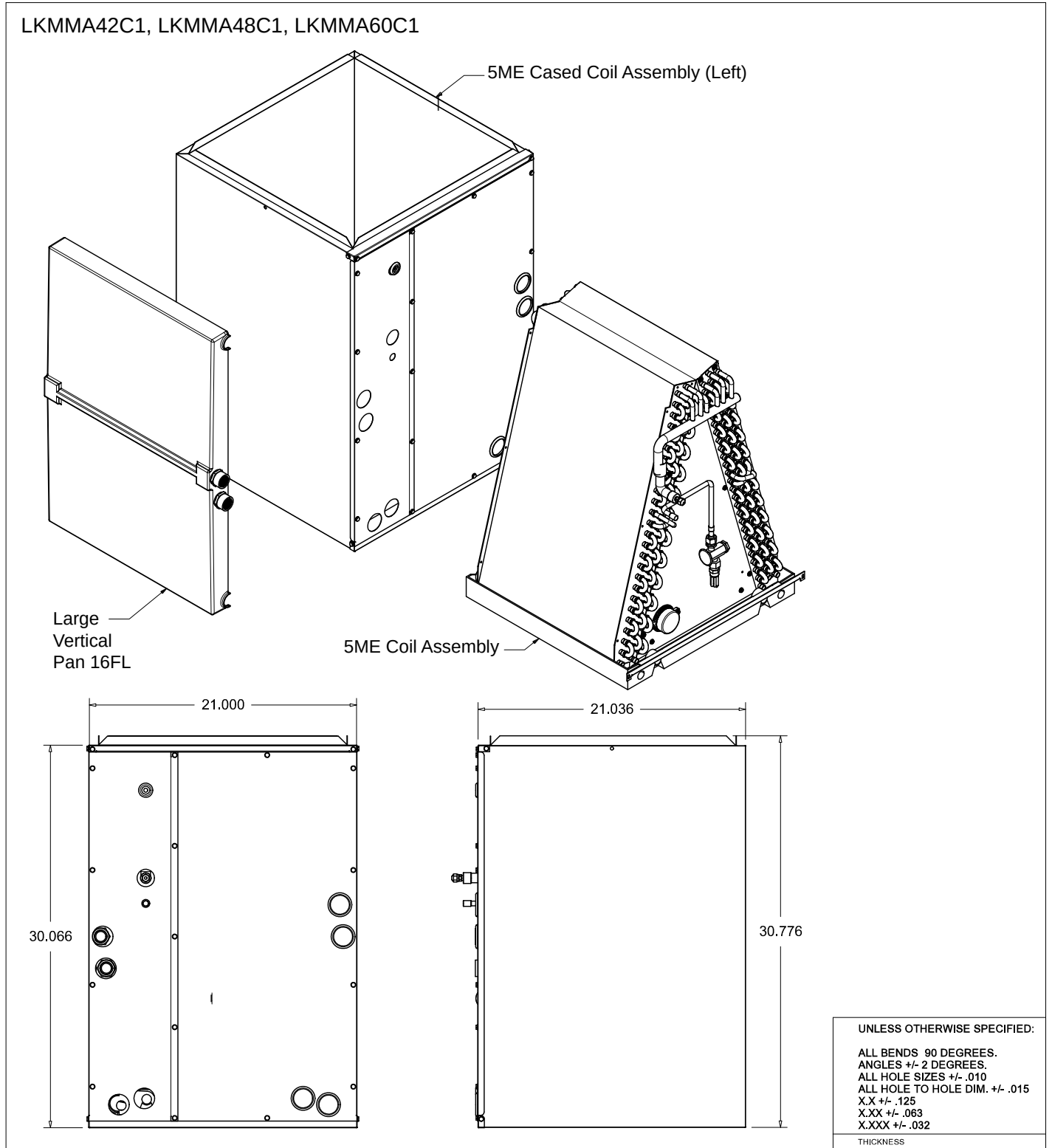
Figure 13: LKMMMA42C1, LKMMMA48C1, LKMMMA60C1 A-Coil Unit Dimensions.
