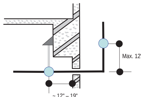
Figure 56: Typical Pipe Support Location—Change in Pipe Direction.
