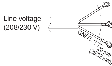
Figure 65: Power Wiring Example.
