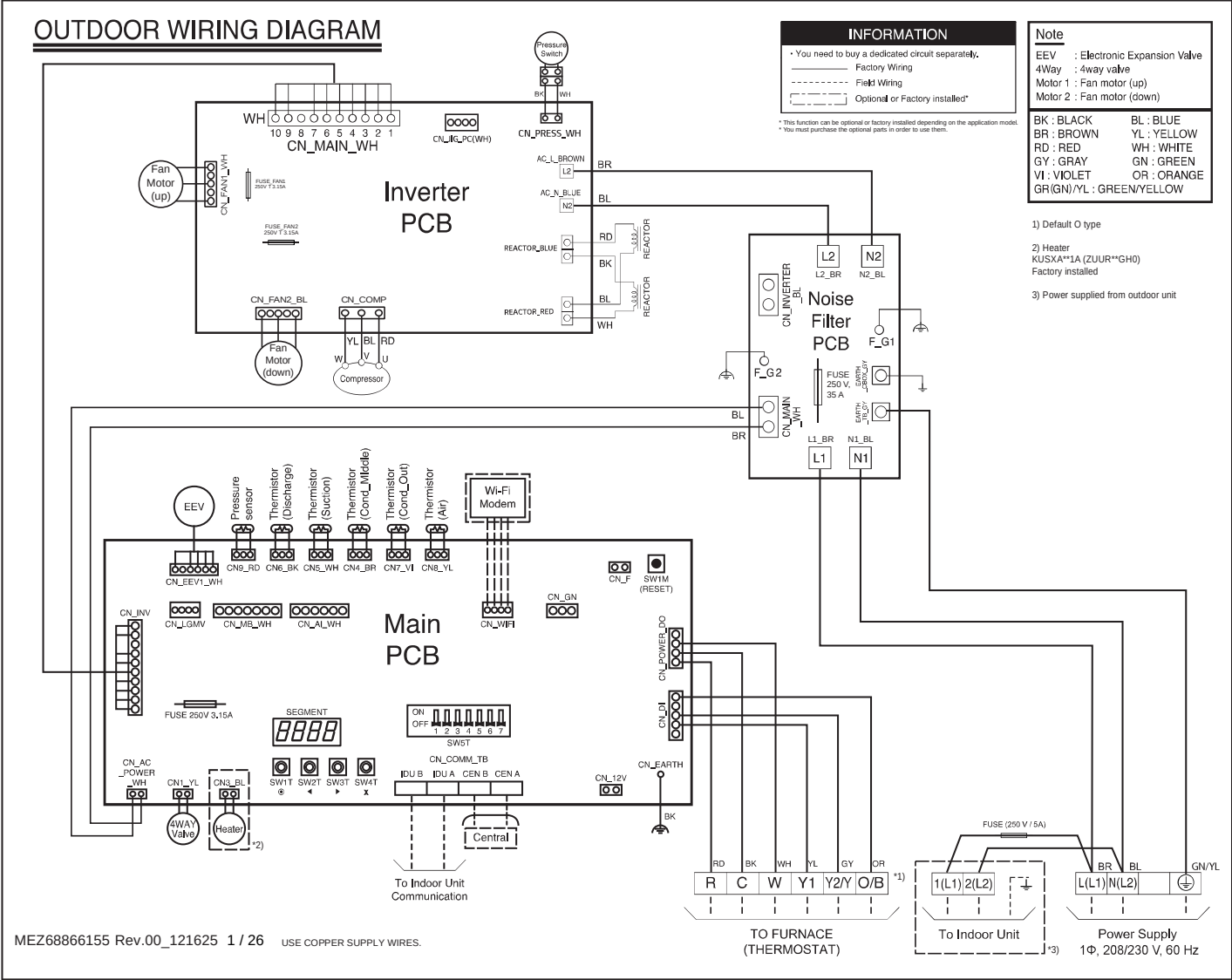
Figure 60: KUSXB361A Outdoor Unit Wiring Diagram.
