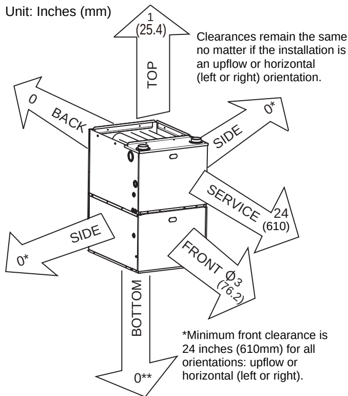
Figure 25: Clearance Requirements for 96% Efficiency Gas Furnaces.
