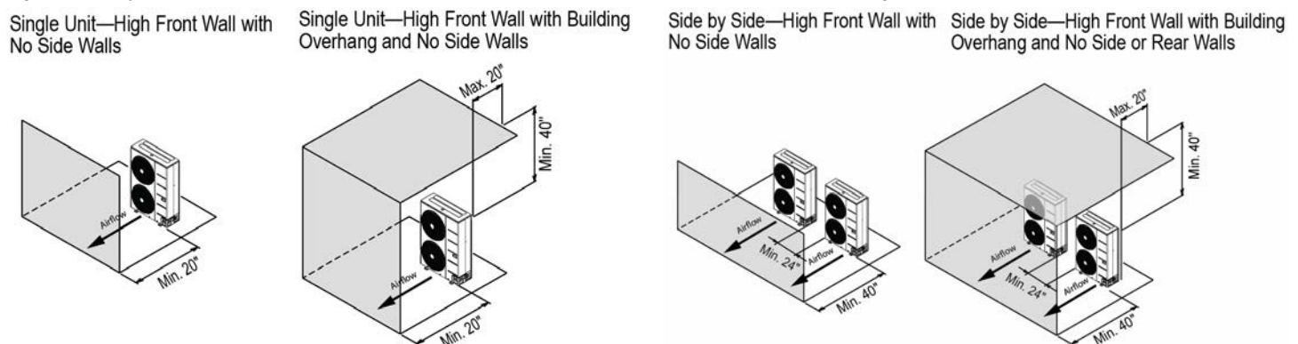
Figure 42: Proper Outdoor Unit Placement and Clearances When There Are Obstacles on the Discharge Side.
