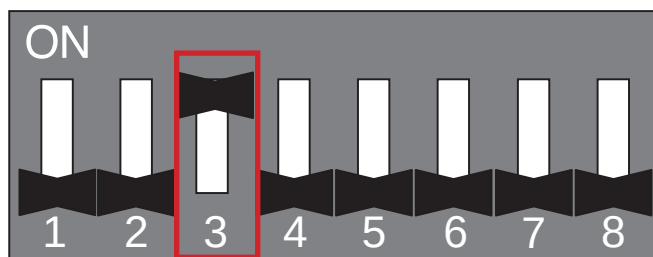
Figure 78: SW-01 DIP Switch Heat Pump Communication Kit Setting for A-Coil / Third-Party Furnace.
