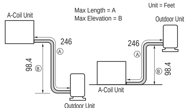
Figure 52: Typical 36k ~ 60k System Layout.
