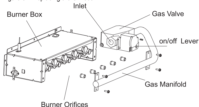
Figure 32: Replacing the Orifices.
