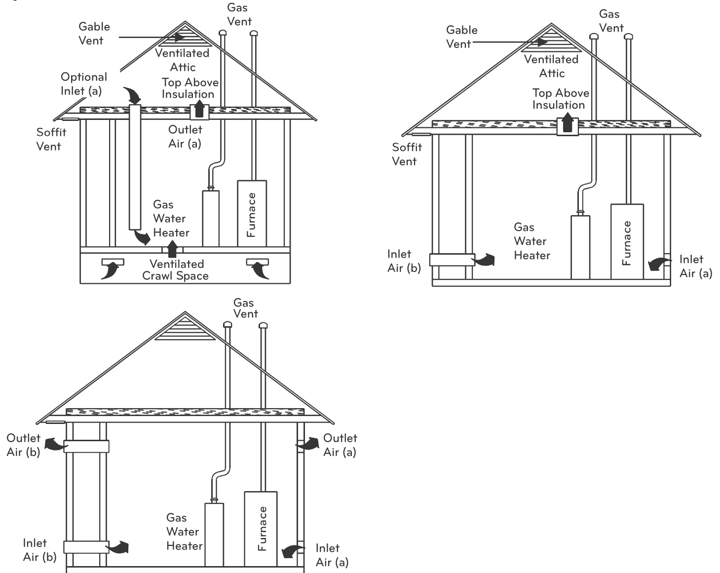
Figure 31: Outside and Ambient Combustion Air Considerations.
