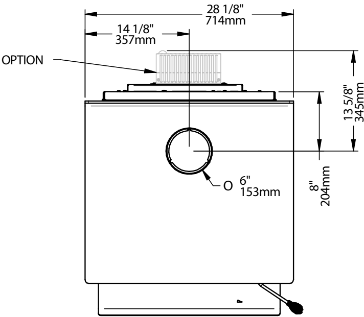
Figure 1: Top View
