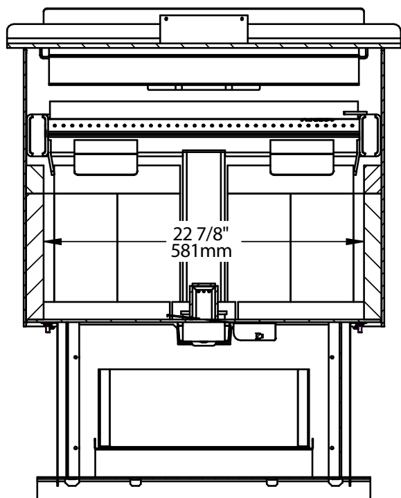
Figure 5: Front View - Combustion Chamber
