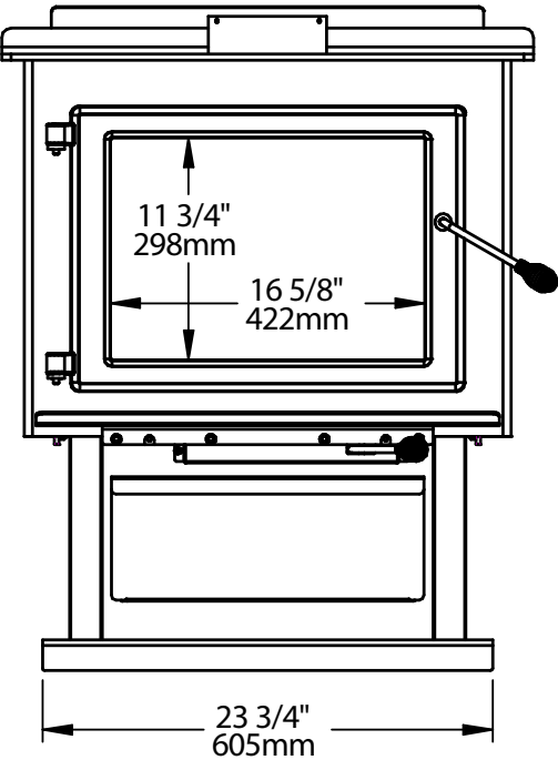
Figure 2: Front View
