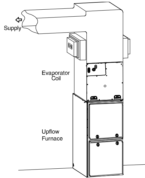
Fig. 16 – Humidifier Application A221127
