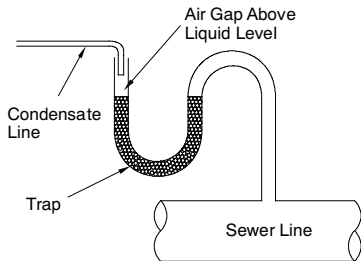
Fig. 15 – Condensate Drain to Waste Line A10216
