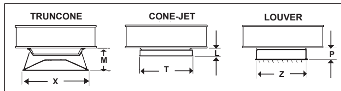
Figure 4 - Vertical Air Outlet Accessories
