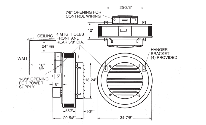
Figure 11 - Model PTE Dimensions (inches)
