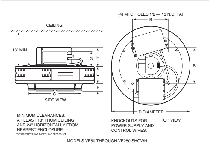
Figure 12 - Model VE Dimensions (inches)
