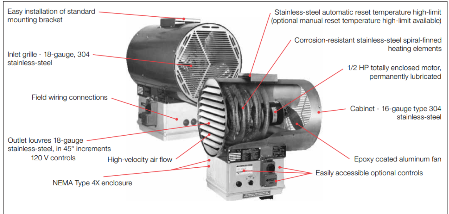
Figure 3 - Model MEW Controls and Features
