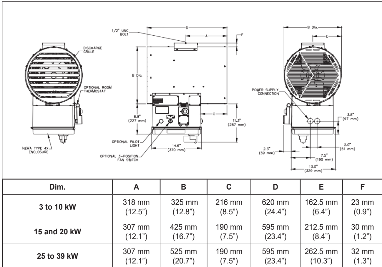
Figure 14 - Model MEW Dimensions
