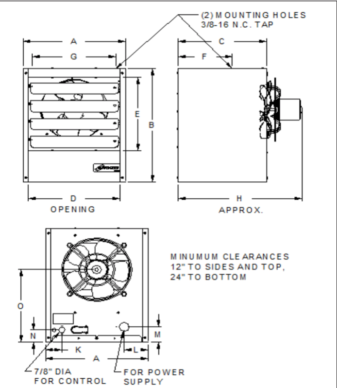
Figure 10 - Model HER Dimensions (inches)
