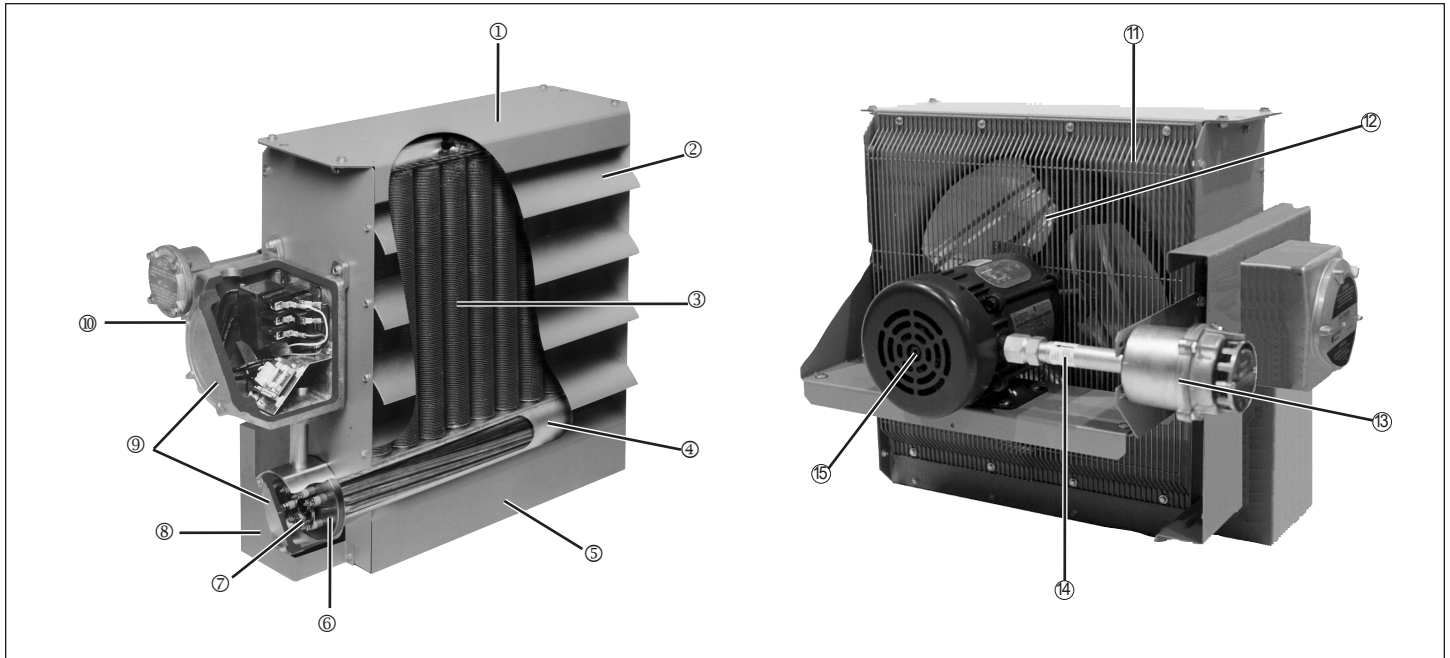
Figure 2 - Model HEX Controls and Features
