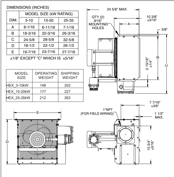
Figure 13 - Model HEX Dimensions (inches)
