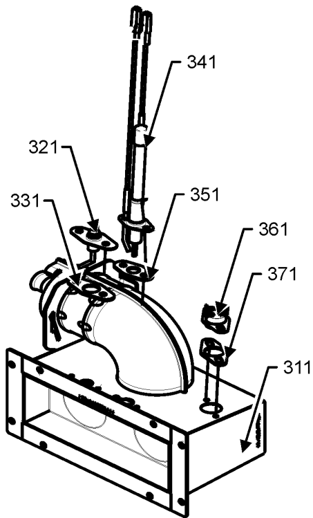
BURNER ASSEMBLY
