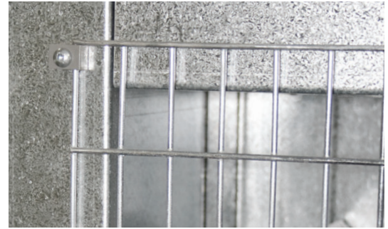
Removable 12-gauge 1" x 2" wire mesh guards are hot dip galvanized after welding. The guard is attached to the housing with poly guard clips to reduce noise and vibration.
