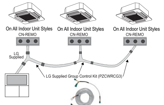
Figure 300: Example of Indoor Unit Group to Zone Controller Connections (CN-REMO).
