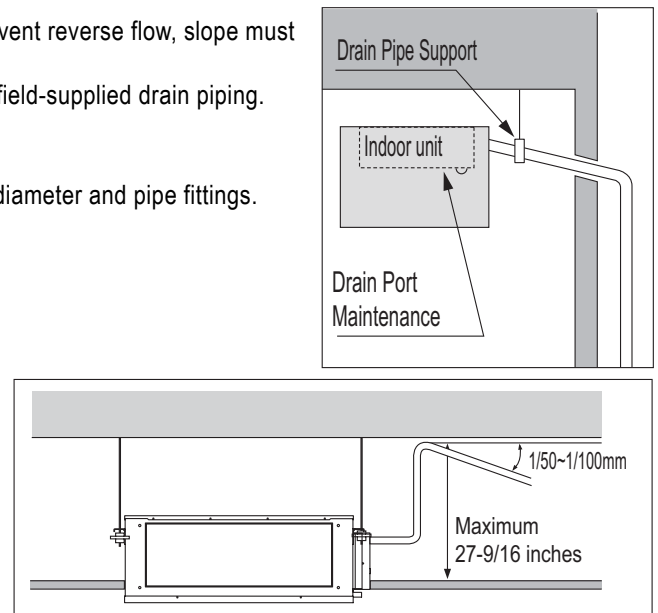
Figure 166: Indoor Unit Drain Piping.
