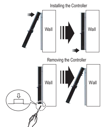
Figure 214: Installing / Removing the Controller.
