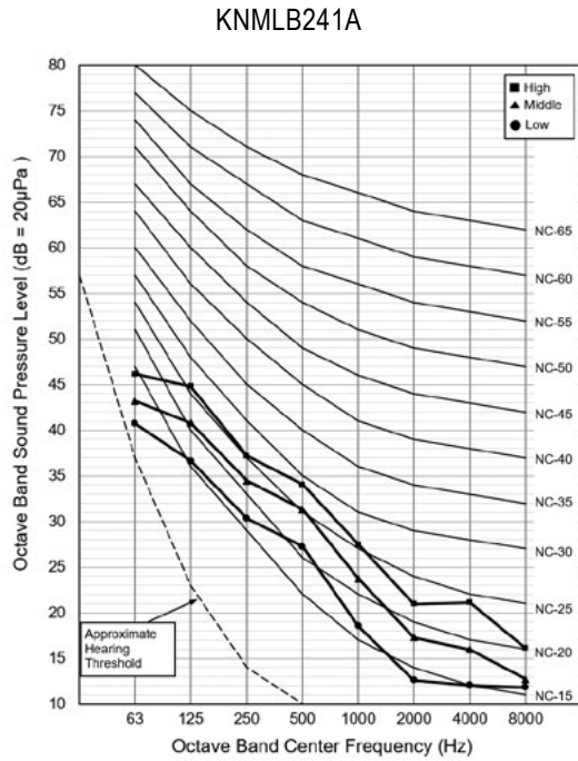
Figure 248: Sound Pressure Level Diagrams - continued.
