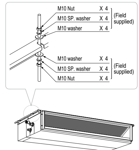
Figure 102: Hanging the Indoor Unit.
