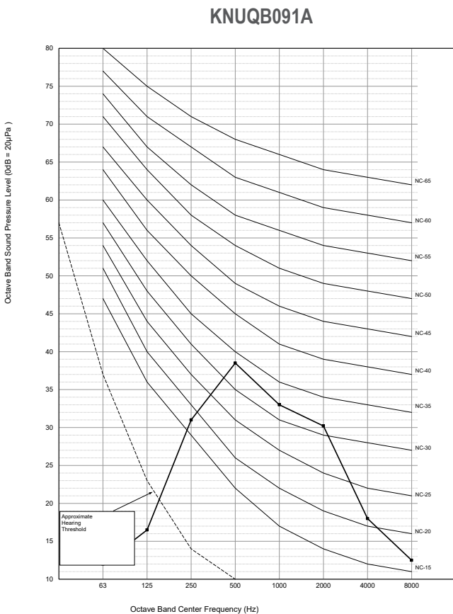
Figure 67: KNUQB091A and KNUQB121A Sound Pressure Level Diagrams.
