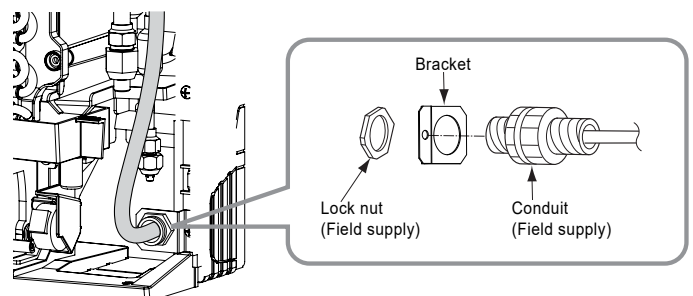
Figure 81: Securing Wiring to Unit.
