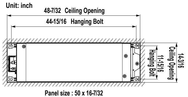
Figure 225: Ceiling Opening Dimensions and Bolt Locations.
