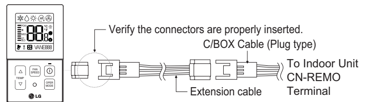
Figure 175: Wired Controller Connections on the Indoor Unit Terminal Block.
