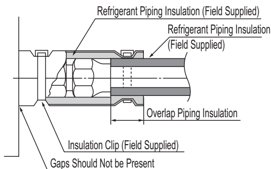
Figure 266: Close Up of Refrigerant Piping Connection Insulation.
