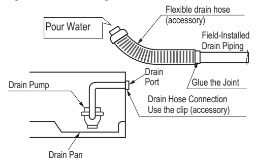
Figure 230: Checking the Drain Pump.
