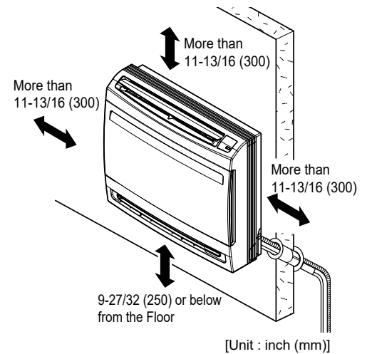
Figure 73: Minimum Clearance Requirements.
