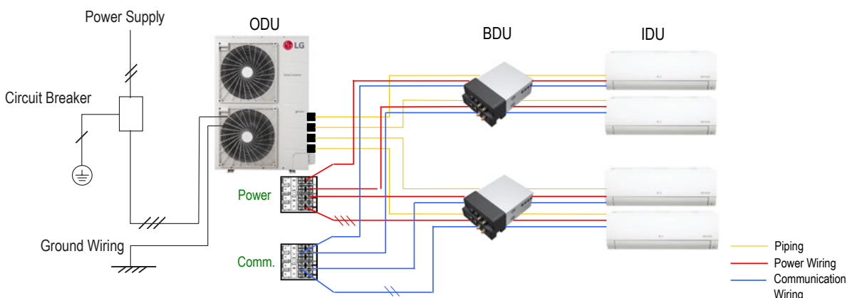
Figure 291: Example of a Multi F MAX with LGRED System General Power / Communications System Schematic.
