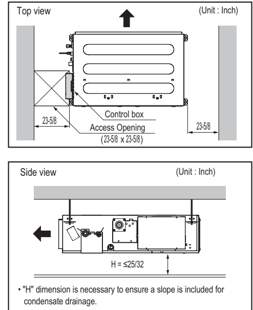
Figure 96: General Installation Guidelines.
