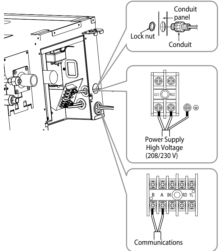
Figure 173: Exterior View of Conduit Installation.
