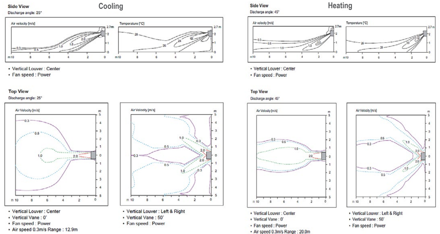
Figure 7: KNUAK181A Air Velocity and Temperature Distribution Charts.
