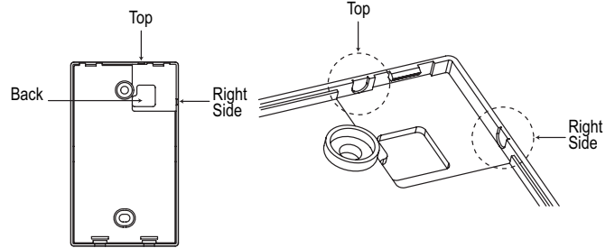
Figure 60: Removing the Cable Guide Grooves.
