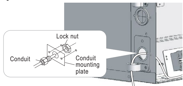
Figure 110: Exterior View of Conduit Installation.
