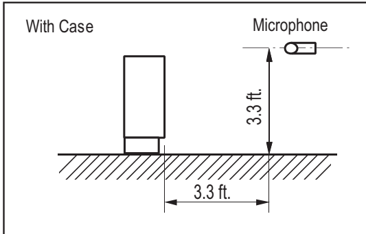
Figure 246: Sound Pressure Level Measurement Location.
