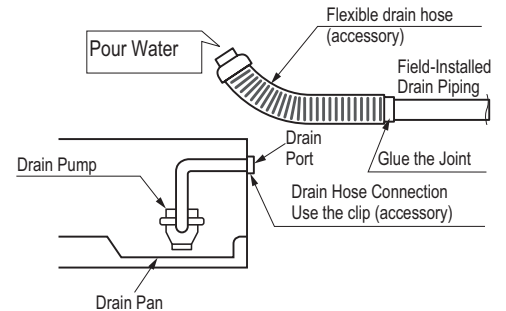
Figure 136: Checking the drain pump.
