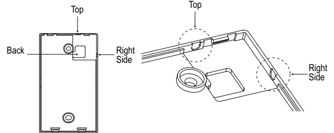
Figure 179: Installing / Removing the Controller.
