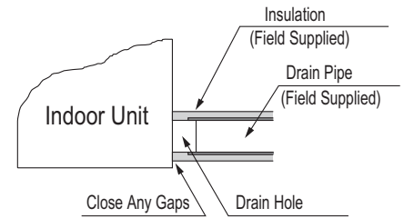
Figure 103: Drain Connection.
