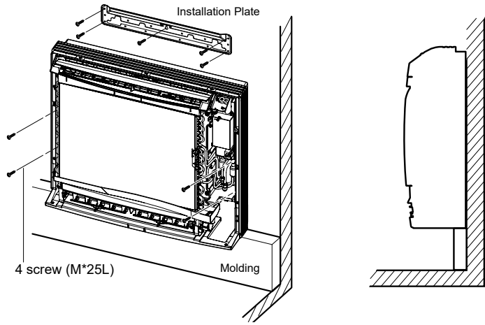
Figure 75: Wall Installation.
