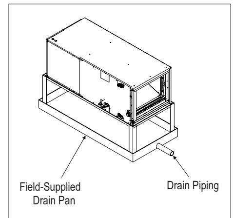
Figure 261: Typical Horizontal Left/Right Installation Drain System.
