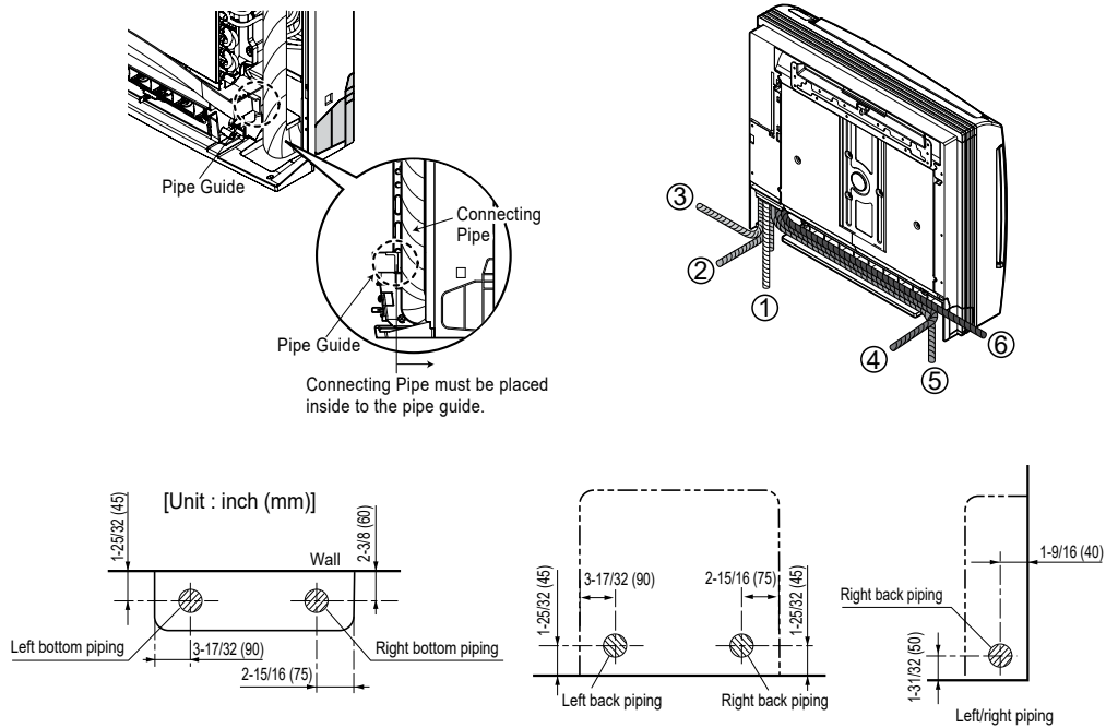
Figure 77: Pipe Holes and Routing.
