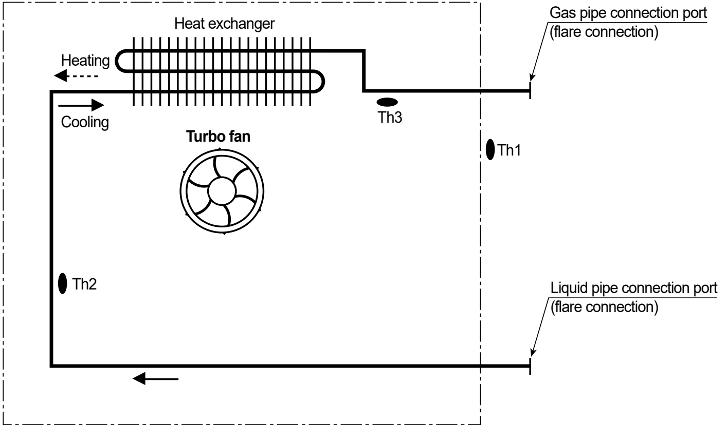
Figure 193: Multi F Four-Way Ceiling-Cassette Indoor Unit Refrigerant Flow Diagram.
