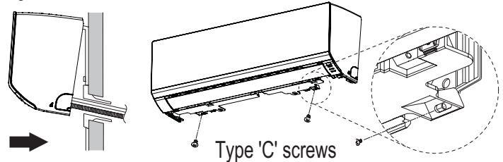
Figure 59: Attach Bottom of Indoor Unit to Installation Plate.
