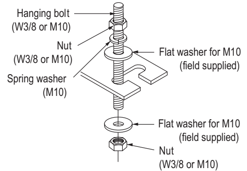
Figure 228: Hanging the Indoor Unit.
