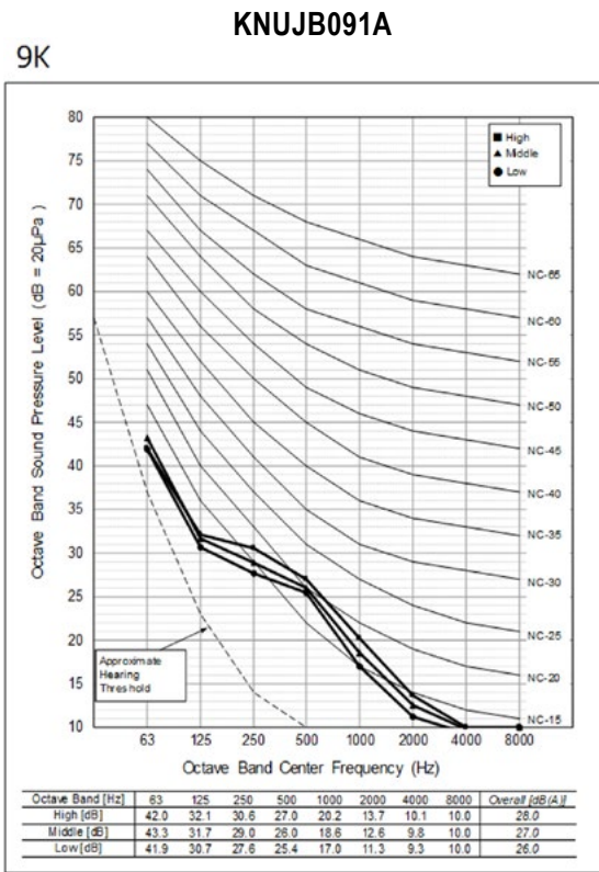
Figure 123: Multi F Convertible Mid Static Duct Sound Pressure Level Diagrams.
