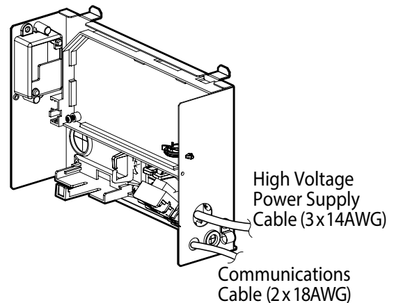
Figure 171: Access Holes Location.
