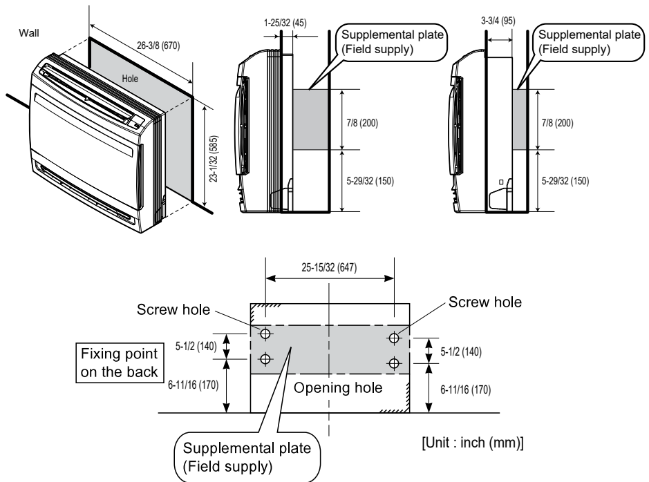
Figure 76: Recessed Installation.
