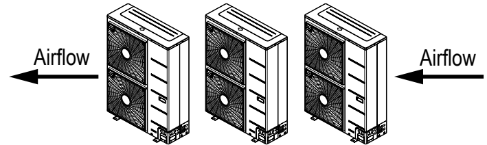
Figure 280: Proper Outdoor Unit Placement and Clearances When There Are Obstacles on the Suction Side.
