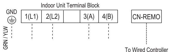
Figure 175: Wired Controller Connections on the Indoor Unit Terminal Block.
