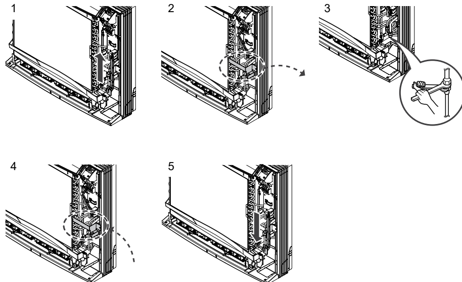
Figure 78: Pipe Connection.
