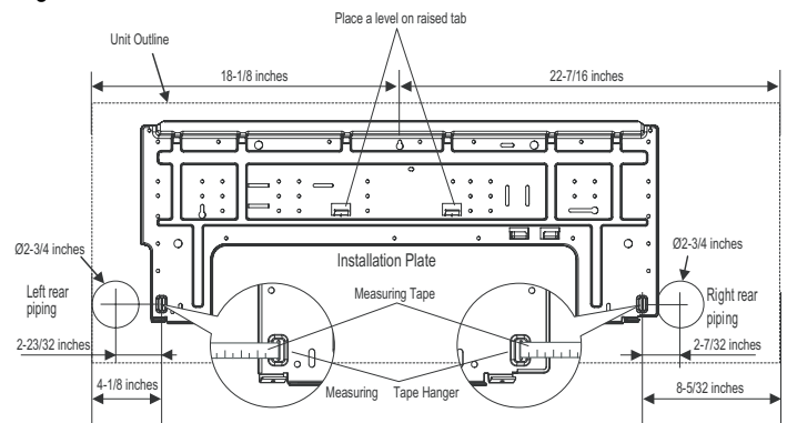
Figure 45: Installation Plate for KNUAB181A and KNMAB241A Units.
