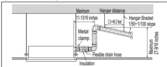
Figure 135: Drain Piping Installation Dimensions.
