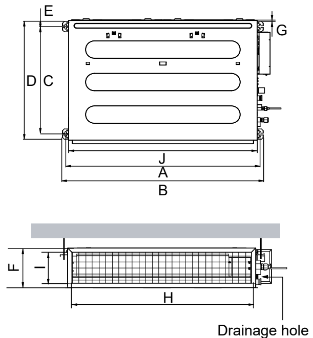
Figure 162: Indoor Unit Bolt Locations.
