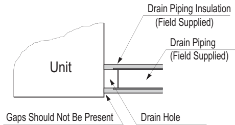
Figure 262: Close up of Drain Piping Connection.
