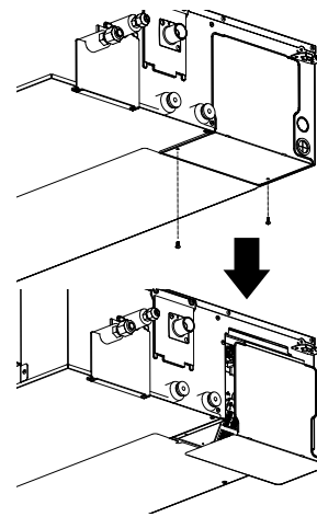
Figure 142: Access Holes Location.
