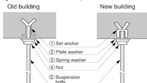
Figure 101: Console Bolt Options.
