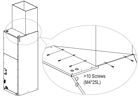
Figure 259: Securing the Ducts to the Unit.
