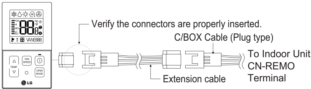
Figure 270: PZCWRC1 LG Wired Remote Extension Cable.
