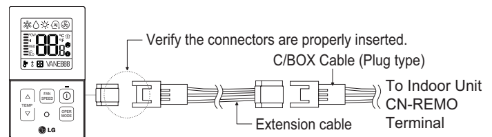
Figure 236: PZCWRC1 LG Wired Remote Extension Cable.
