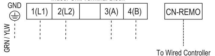
Figure 237: Wired Controller Connections on the Indoor Unit Terminal Block.
