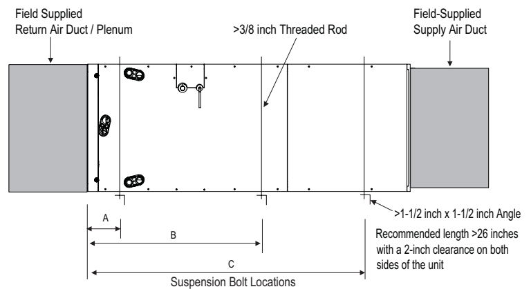
Figure 258: Typical Horizontal Right Installation.
