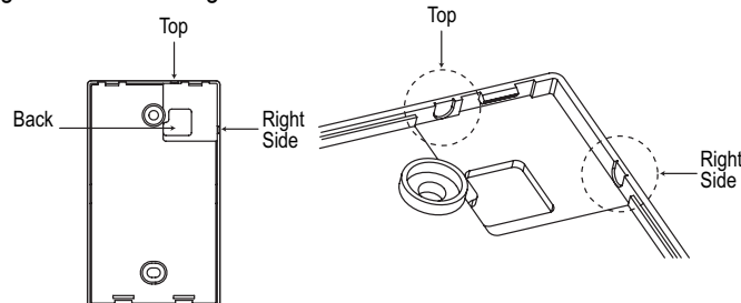
Figure 150: Installing / Removing the Controller.
