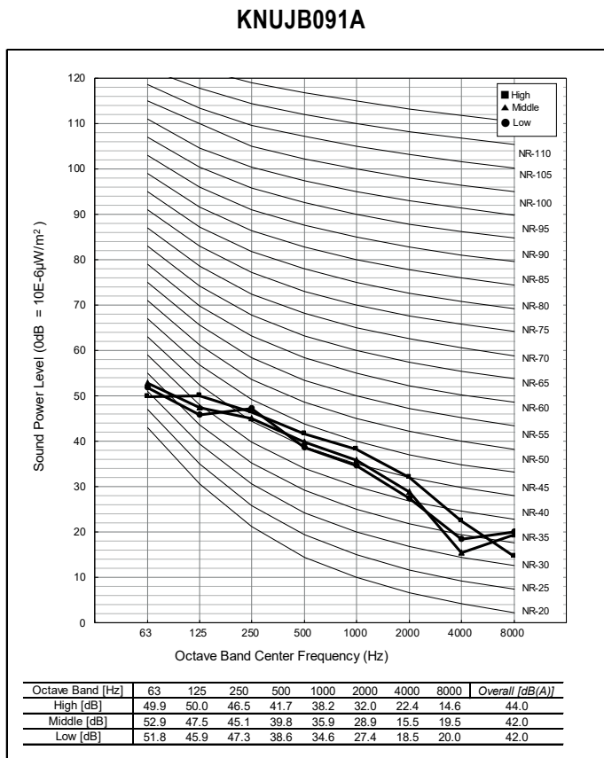
Figure 124: Sound Power Level Diagrams, KNUJB091A, KNUJB121A.
