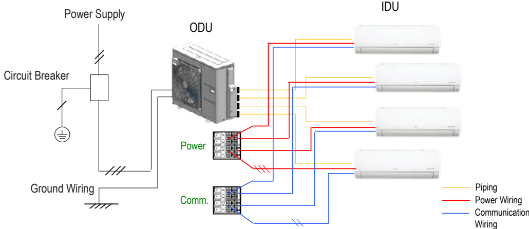
Figure 290: Example of a Multi F with LGRED System General Power / Communications System Schematic.
