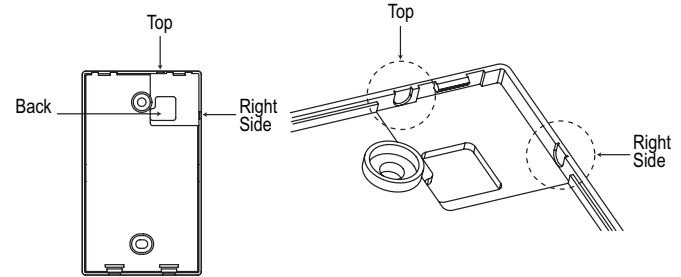
Figure 240: Attaching the Wall Plate.
