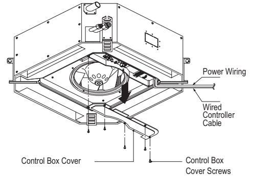
Figure 205: Power Wiring and Communications Cable Connection Access.
