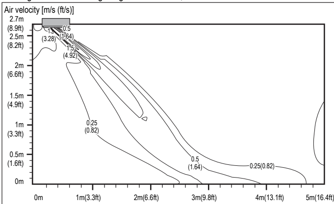
Heating: 12kBtu - Discharge angle : Outer – 53°, Inner – 47°
