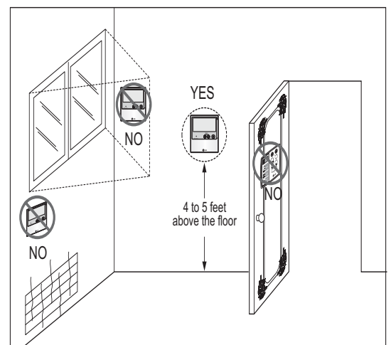
Figure 116: Proper Location for the Wired Controller.
