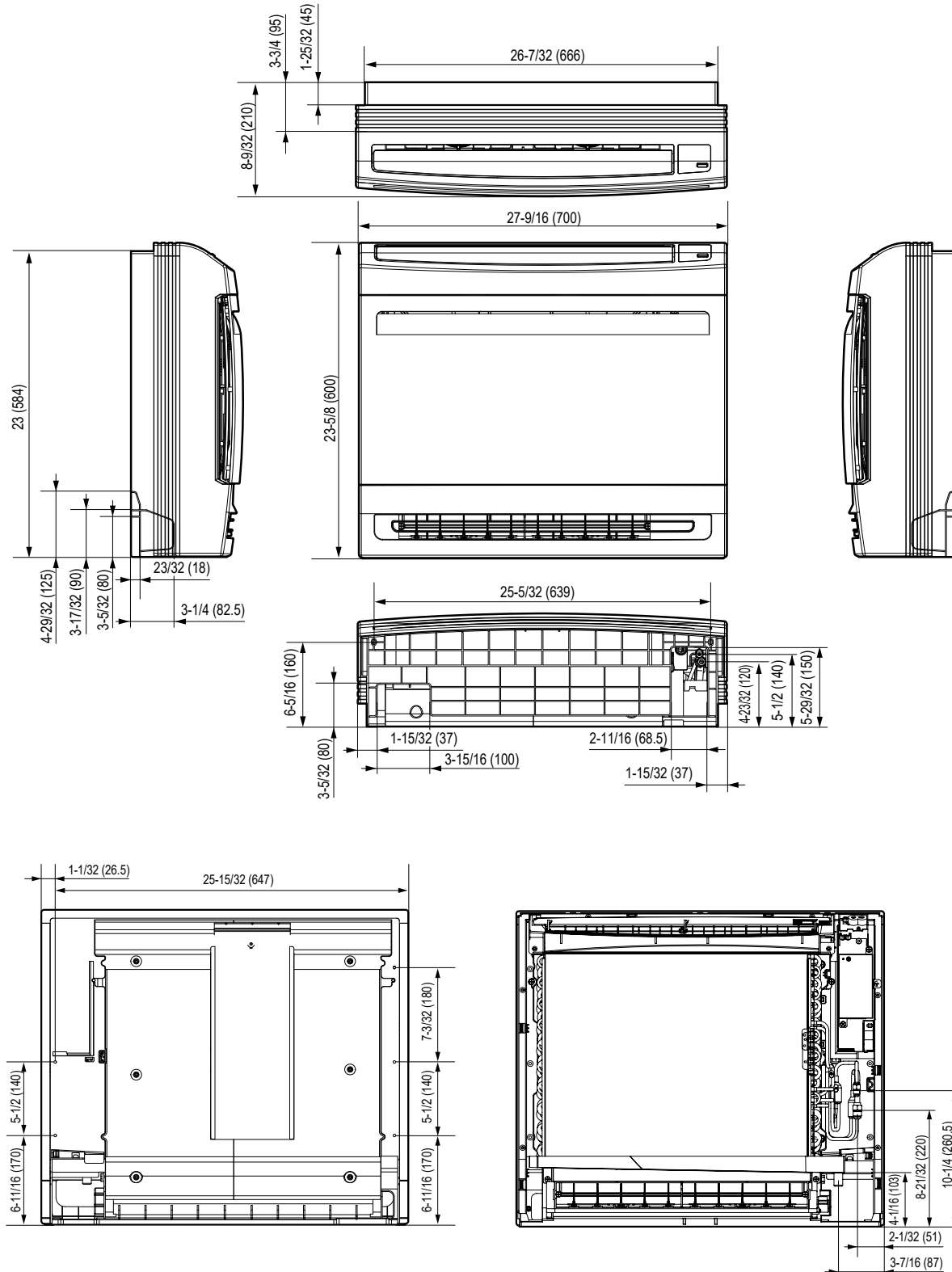
Figure 65: KNUQB091A, KNUQB121A, and KNMQB151A Dimensions.
