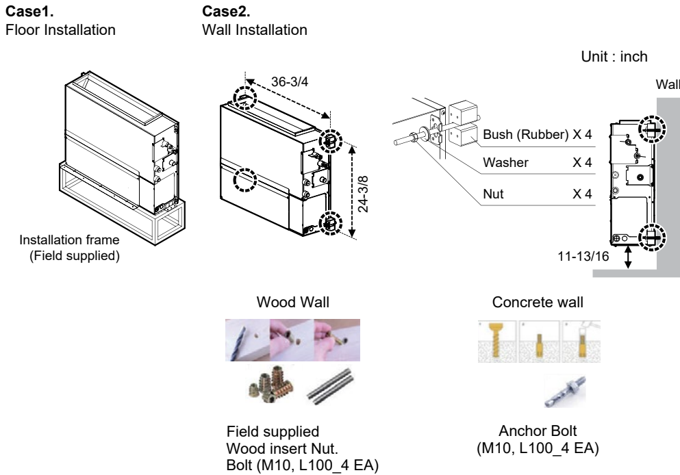
Figure 140: Convertible Mid Static Duct IDU Vertical Installation Drain.
