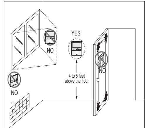
Figure 58: Proper Location for the Wired Controller.
