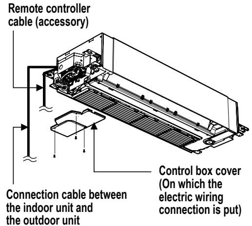
Figure 232: Power Wiring and Communications Cable Connection Access.
