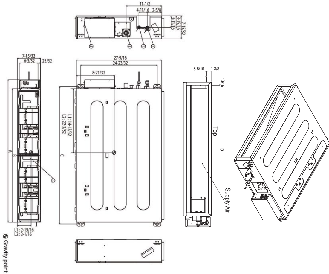
Figure 89: KNMKB091A, KNMKB121A, and KNMKB181A Dimensions.
