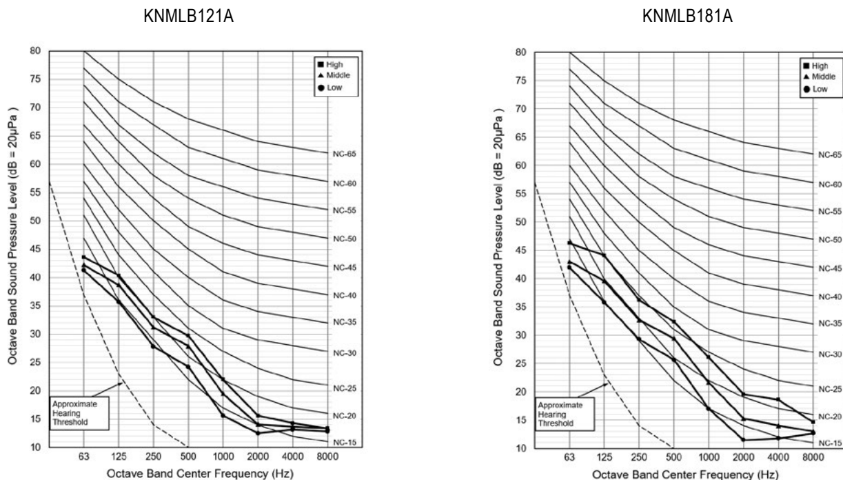
Figure 247: Sound Pressure Level Diagrams.
