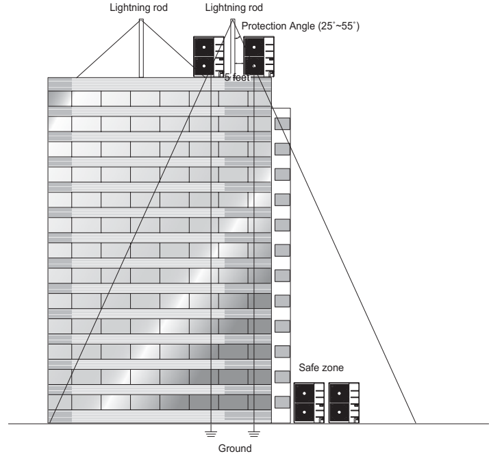
Figure 277: Lightening Protection Diagram.
