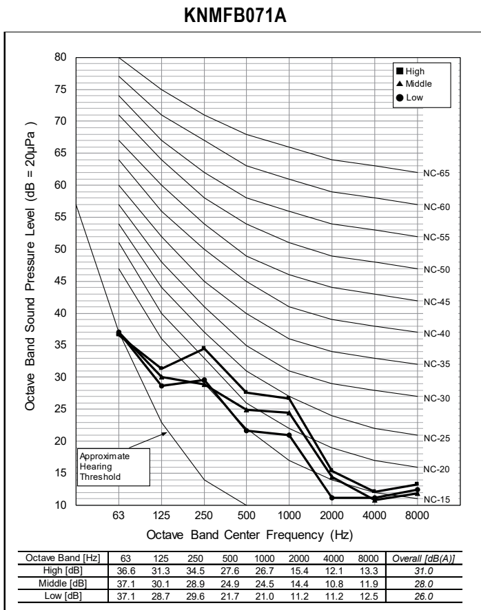
Figure 218: KNMFB071A and KNUFB091A Sound Pressure Level Diagrams.
