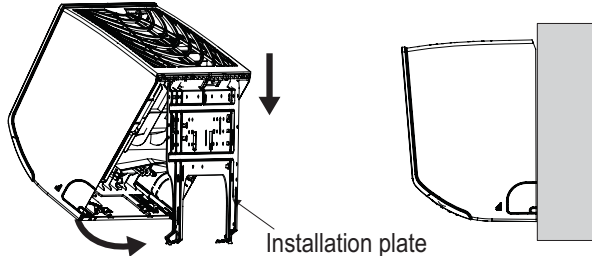
Figure 47: Locking the Indoor Unit onto the Installation Plate.
