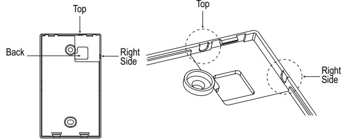
Figure 85: Removing the Cable Guide Grooves.
