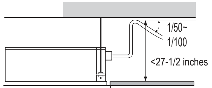
Figure 202: Indoor Unit Drain Piping.
