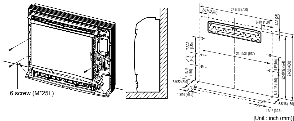
Figure 74: Floor Installation
