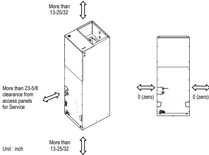
Figure 252: Clearance Requirements.
