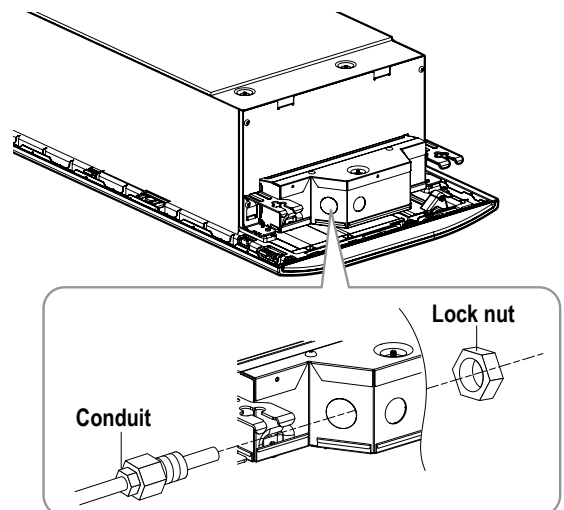
Figure 234: Using a Conduit.
