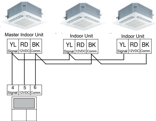
Figure 299: Example of Indoor Unit Group to Zone Controller Connections (Sig-12V-GND [Comm.] Terminal).
