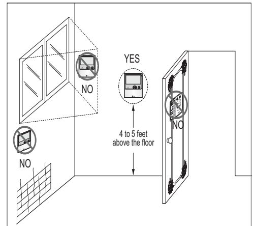
Figure 84: Proper Location for the Wired Controller.
