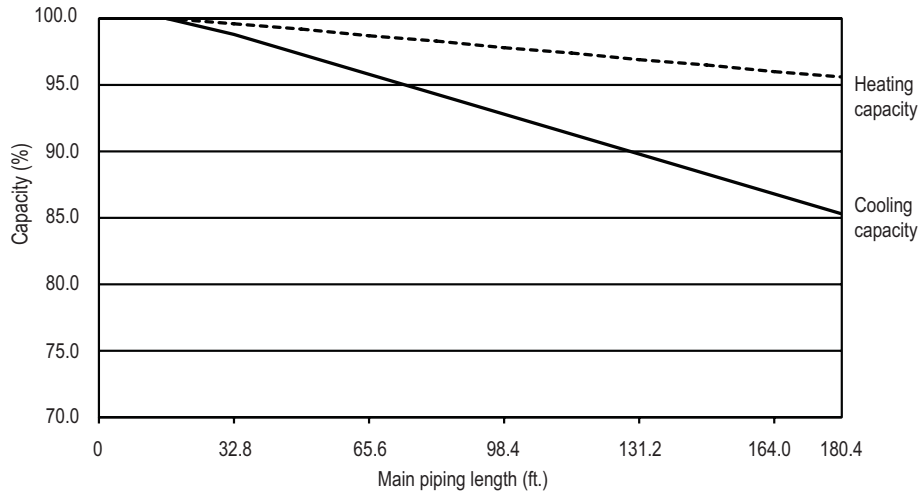
Figure 276: Multi F MAX / Multi F MAX with LGRED Outdoor Unit to Branch Distribution Unit Refrigerant Line Length Derate Chart.
