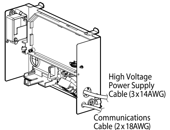
Figure 142: Access Holes Location.
