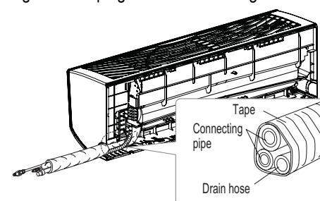
Figure 52: Piping Installed to the Right.
