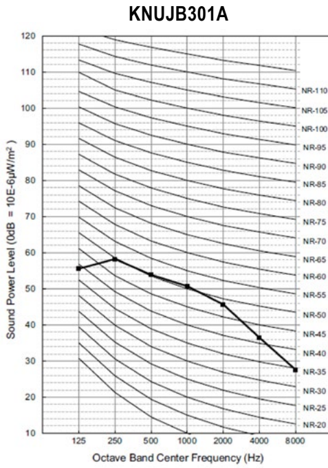
Figure 158: Sound Power Level Diagrams.
