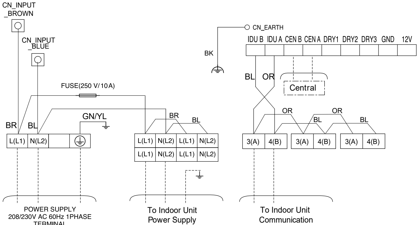
Figure 293: Multi F KUMXB301A and KUMXB361A System Power Wiring and Communications Wiring.
