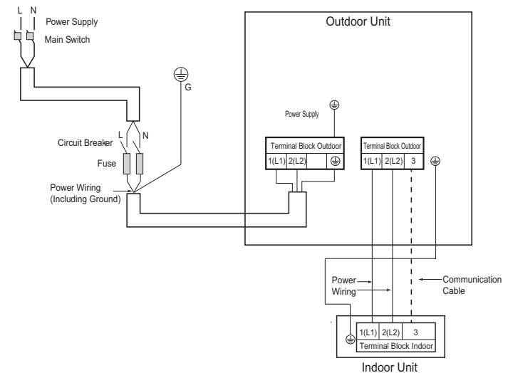
Figure 50: General Standard Efficiency, Mega, and Mega 115V Single Zone System Power / Communications System Schematic (Appearance May Vary).
