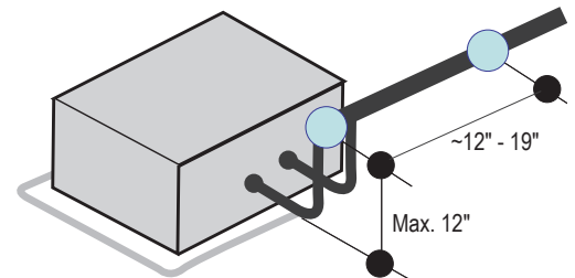
Figure 44: Pipe Support at Indoor Unit.
