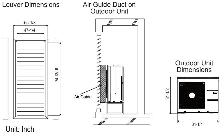
Figure 37: Example of Installing Outdoor Unit Indoors.
