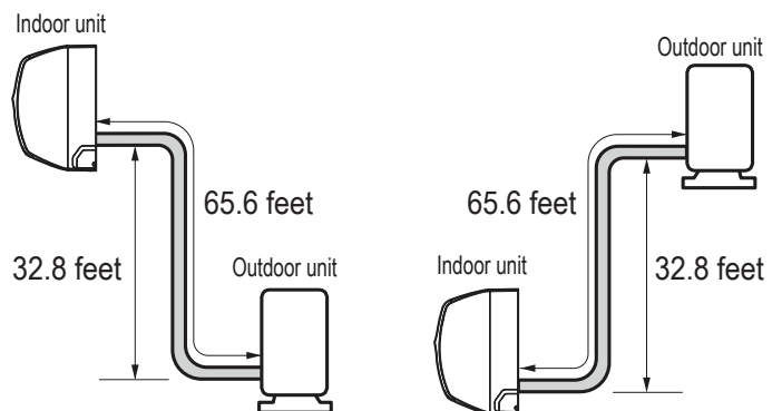
Figure 39: Typical Standard Efficiency and Mega 18,000 Btu/h and 24,000 Btu/h System Layout.
