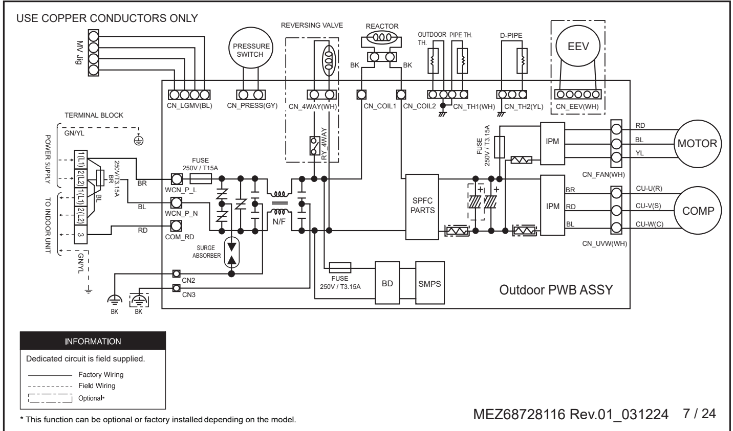
Figure 46: Standard Efficiency KUSAE091A and KUSAE121A, Mega KUSAC091A and KUSAC121A Outdoor Unit Wiring Diagram.
