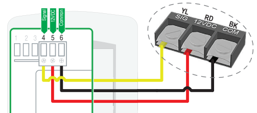
Figure 58: Example of Wired Controller Terminals.
