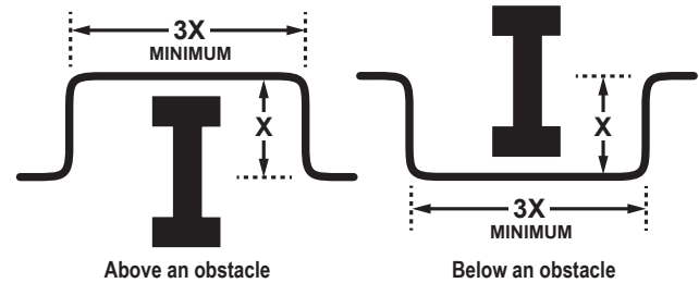
Figure 41: Installing Piping Above and Below an Obstacle.
