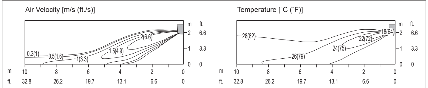
Figure 16: Standard Efficiency KNSAE241A and Mega KNSAC241A Air Velocity and Temperature Distribution Charts.
