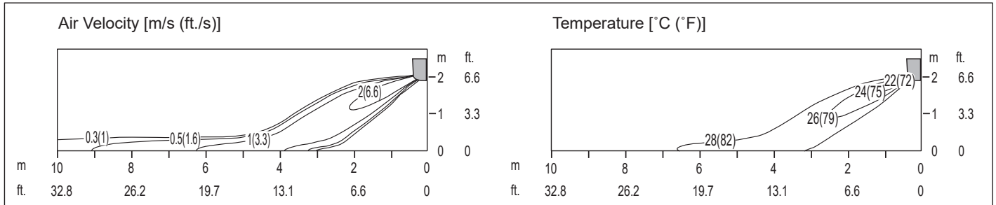
Figure 10: Standard Efficiency KNSAE091A and Mega KNSAC091A Air Velocity and Temperature Distribution Charts.
