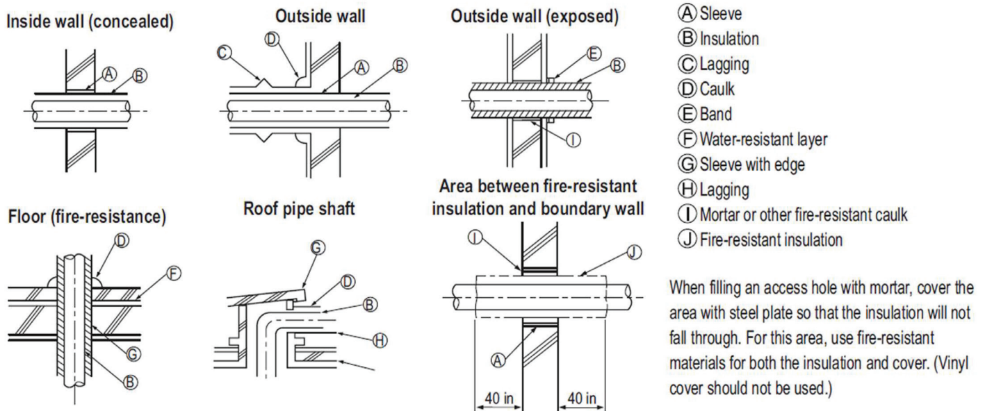
Figure 45: Pipe Sleeve Options.
