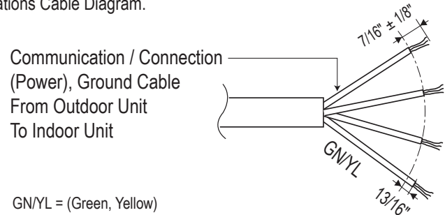
Figure 52: Single Zone Outdoor Unit to Indoor Unit Wiring and Communications Cable Diagram.
