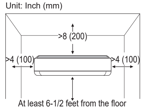
Figure 26: Wall-Mounted Indoor Unit Clearance Requirements.
