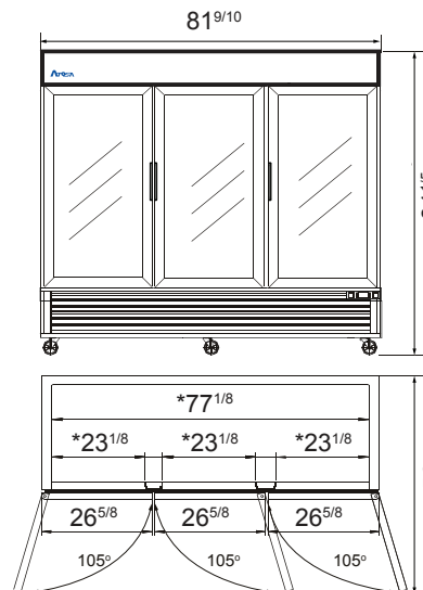
MCF8728GR
