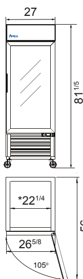
MCF8720GR
