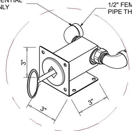
BRACKET DETAIL
