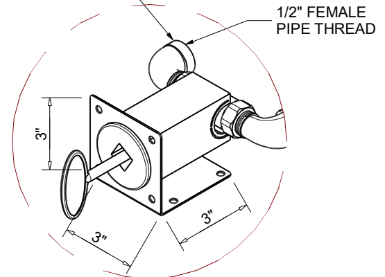
BRACKET DETAIL
