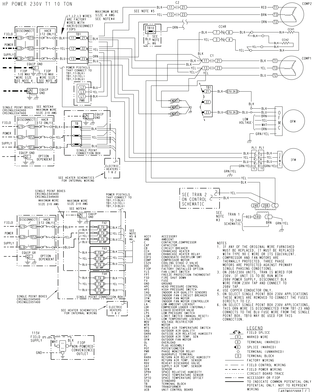
RHV120 Power Wiring Diagram, 230V-3-60 Shown
