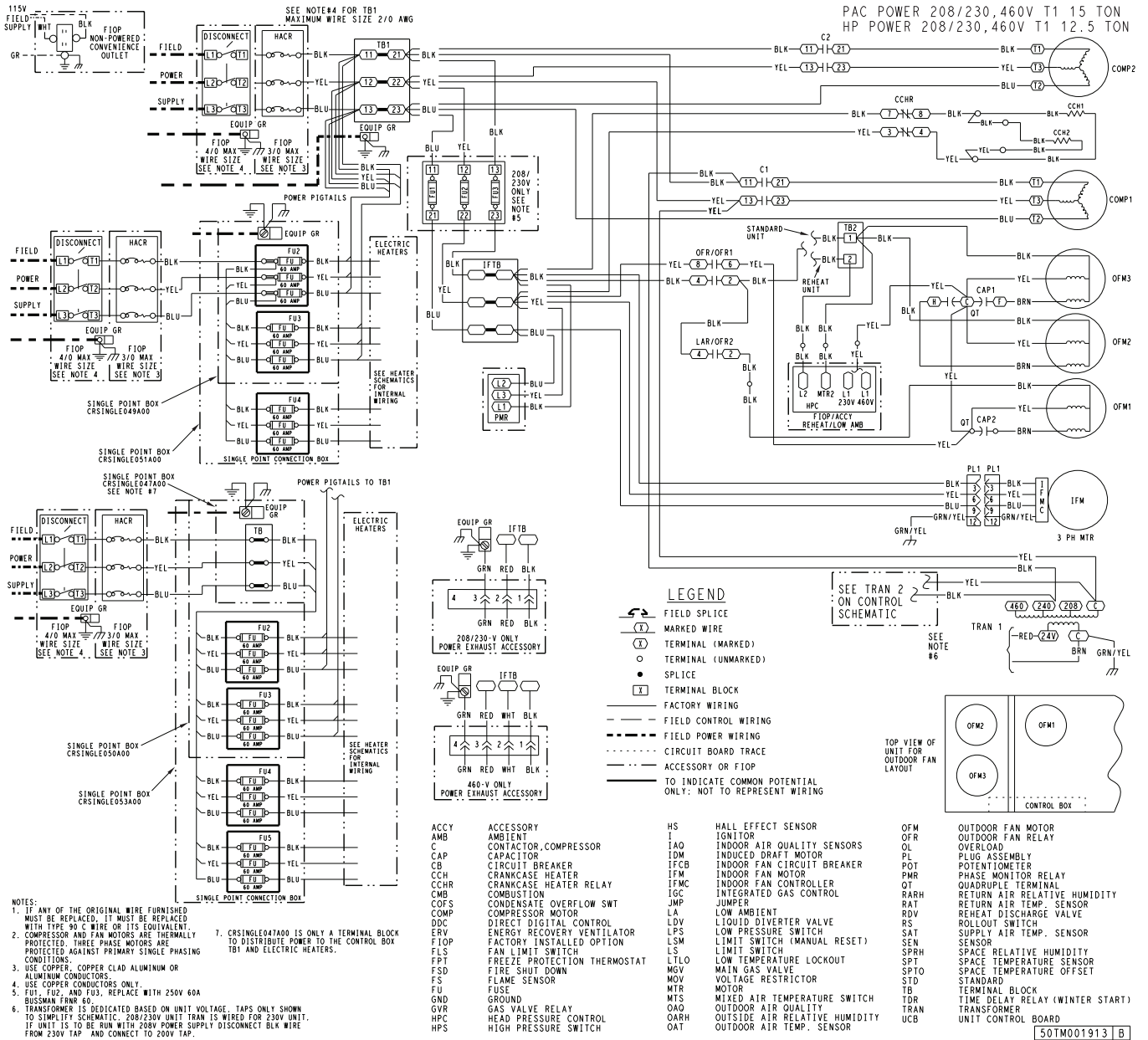
RHV150 Power Wiring Diagram, 208/230, 460V-3-60 Shown
