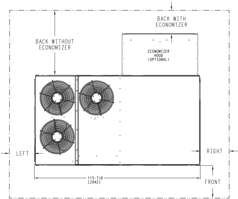
RHV150 Base Unit Dimensions — Clearances
