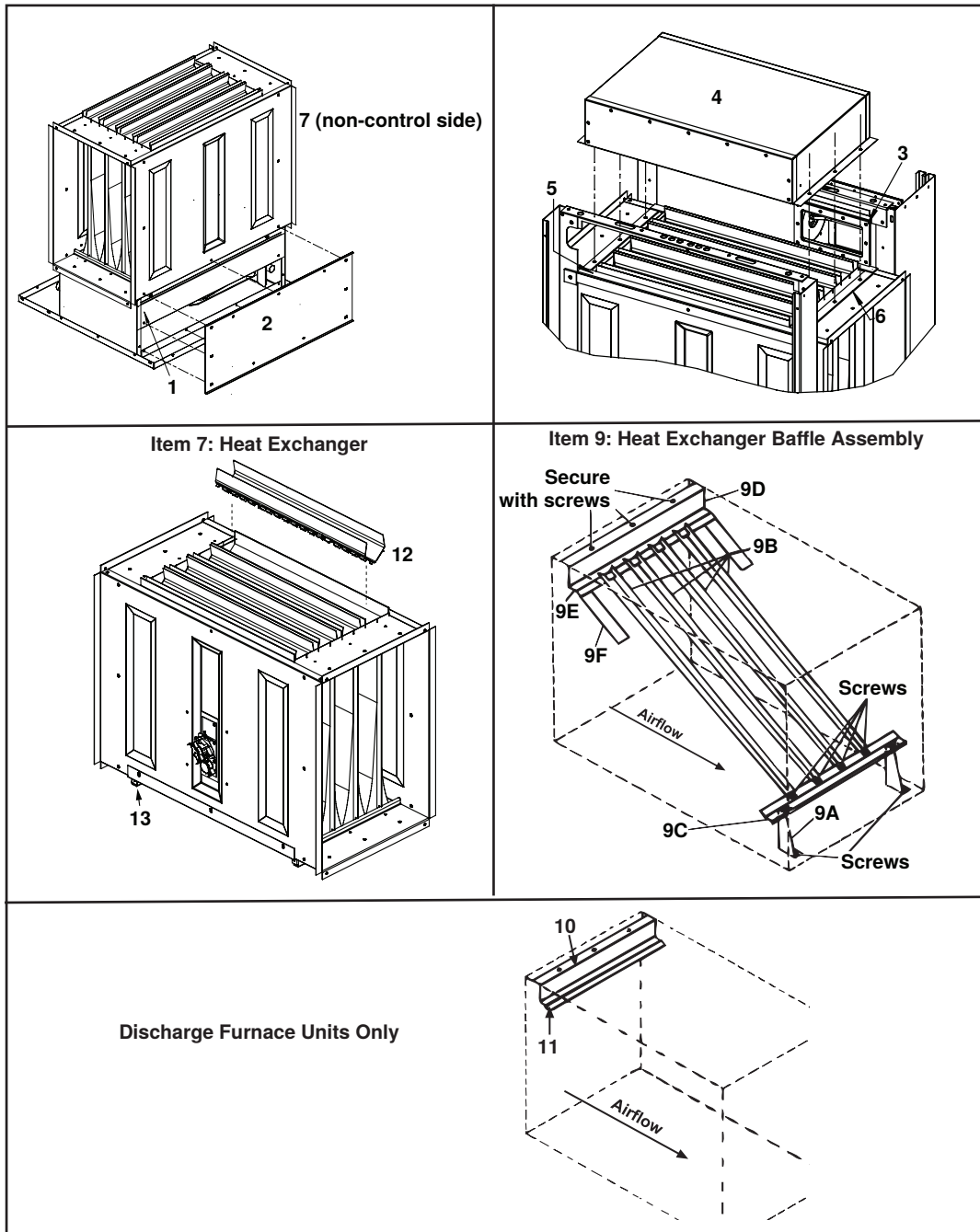
Figure 6. Heat Exchanger Components (Refer to Table 8 )
