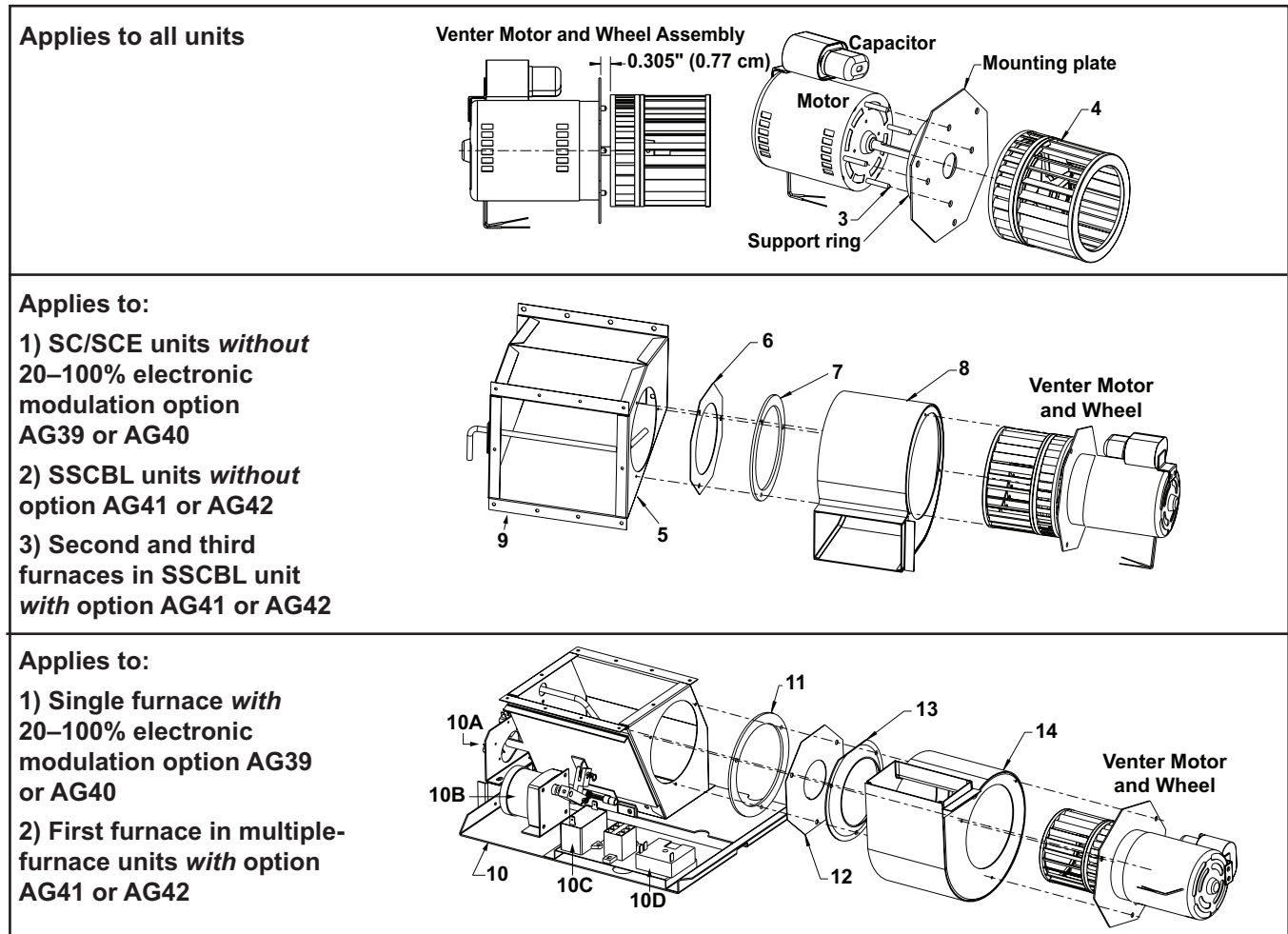
Figure 5. Venter Motor and Wheel Assembly with Flue Duct Components (Refer to Table 6 )
