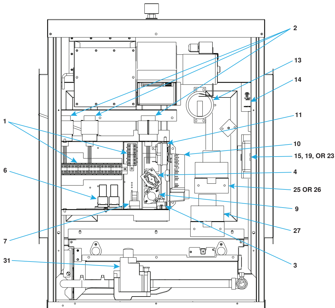
Figure 1. Electrical Components (Refer to Table 2 )
