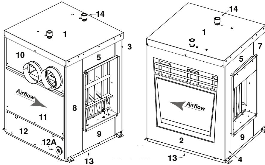
Figure 9. Cabinet Components (Refer to Table 13 )
