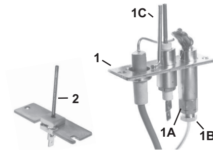
Figure 8. Vertical Spark Pilot (Refer to Table 12 )
