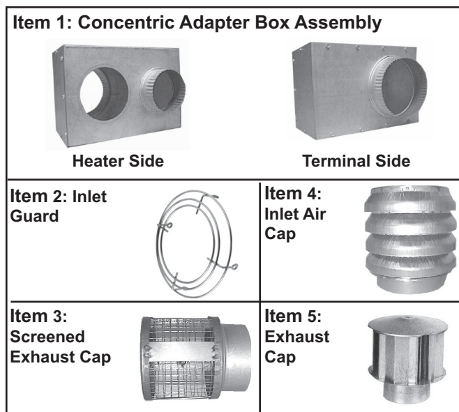
Figure 11. Vent/Combustion Air Kit Components (Refer to Table 14 )
