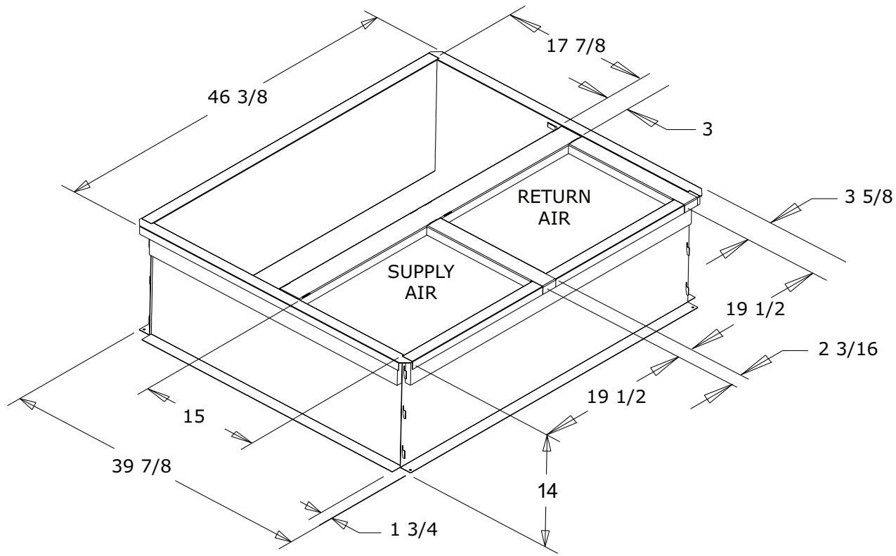
Figure 3. 2.0 — 3.0 Ton Models BAYCURB050A Full Perimeter Roof Mounting Curb
