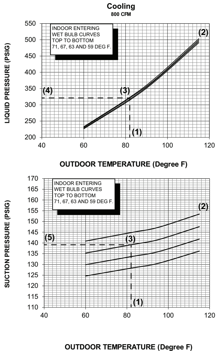
Figure 1. Pressure Curves for A5PA3024
