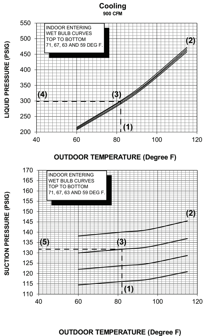
Figure 1. Pressure Curves for A5PA3030
