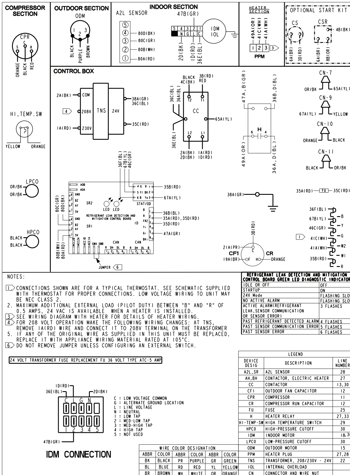
Figure 2. A5PA3030
