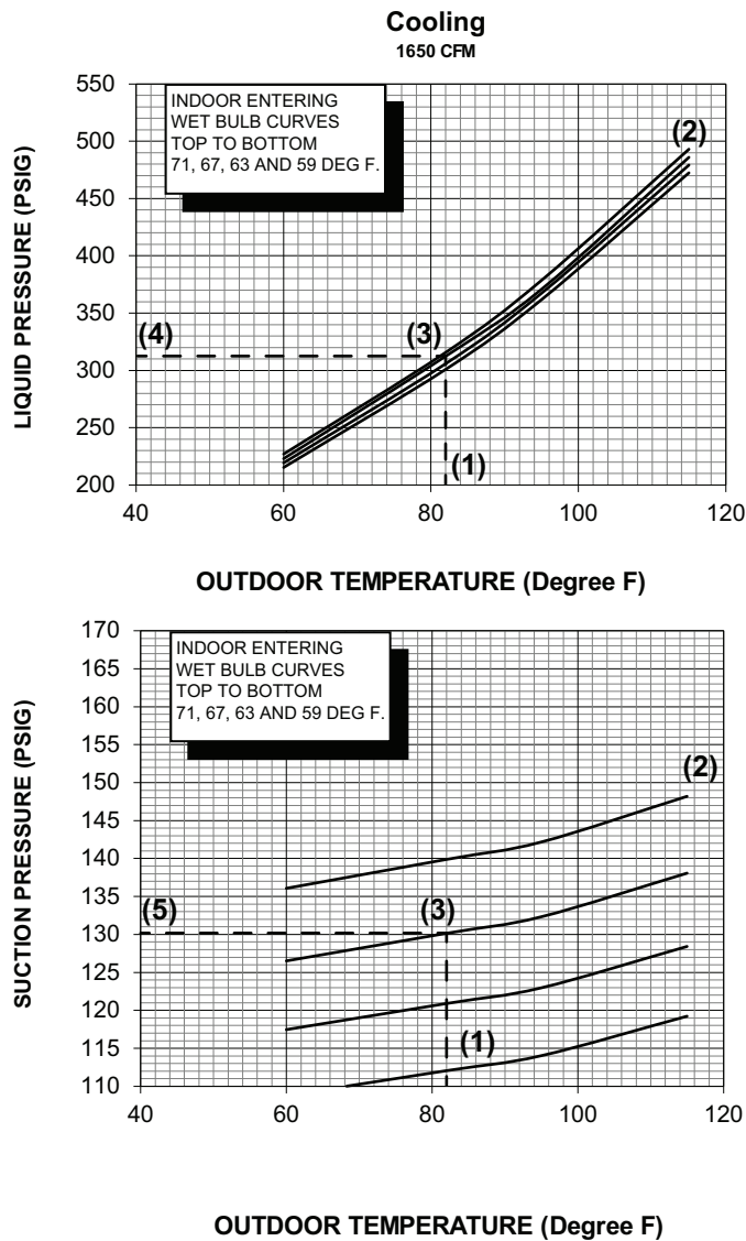
Figure 1. Pressure Curves for A5PA3048
