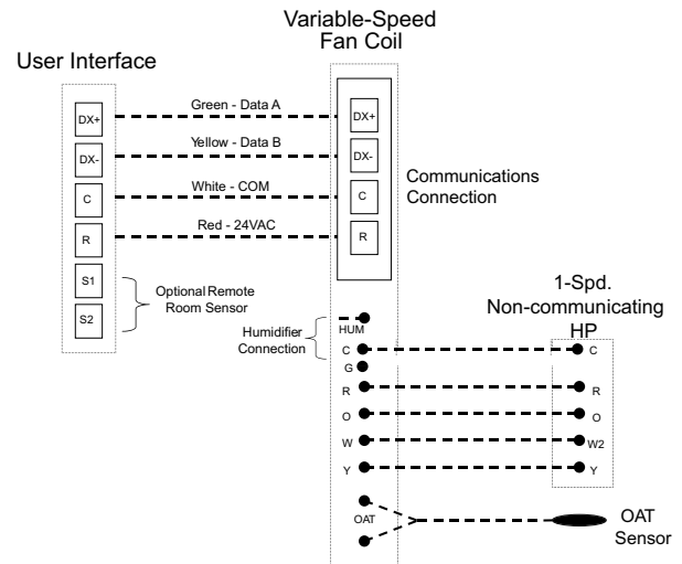
Fig. 3 – Connection Diagram for FCM Fan Coil with Non-Communicating 1-Stage HP
