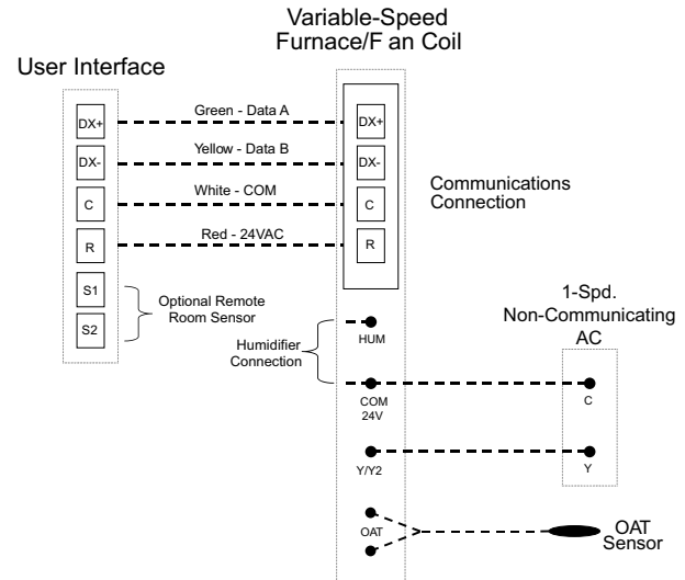
Fig. 2 – Connection Diagram for Furnace or FCM4 Fan Coil w/1-Stage AC
