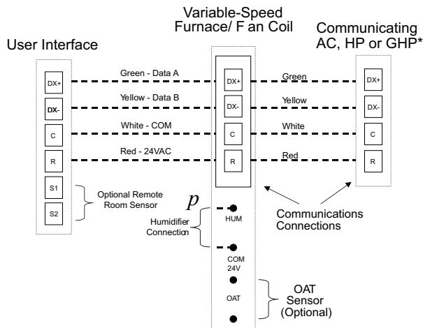
Fig. 1 – Four-Wire Connection Diagram
