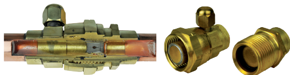
Cutaway of FitRight® Fitting
