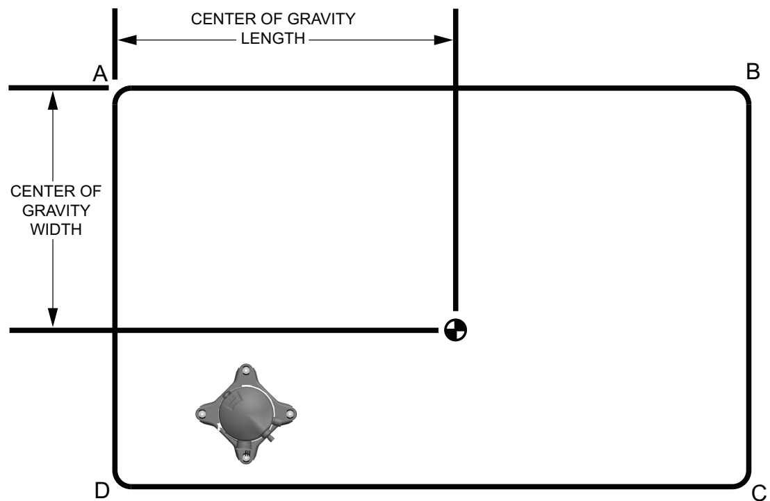
Figure 9. Corner weights
