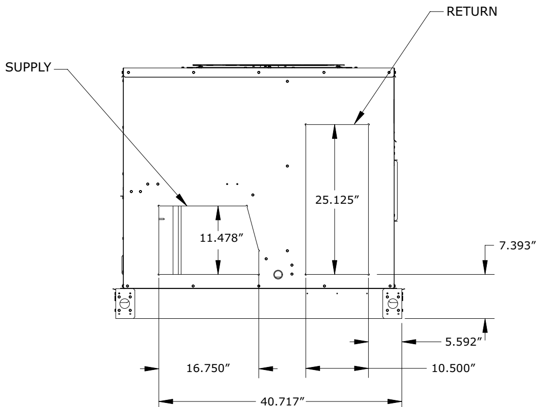
Figure 4. Cooling with optional electrical heat and gas/electric units — back view (horizontal configuration)
