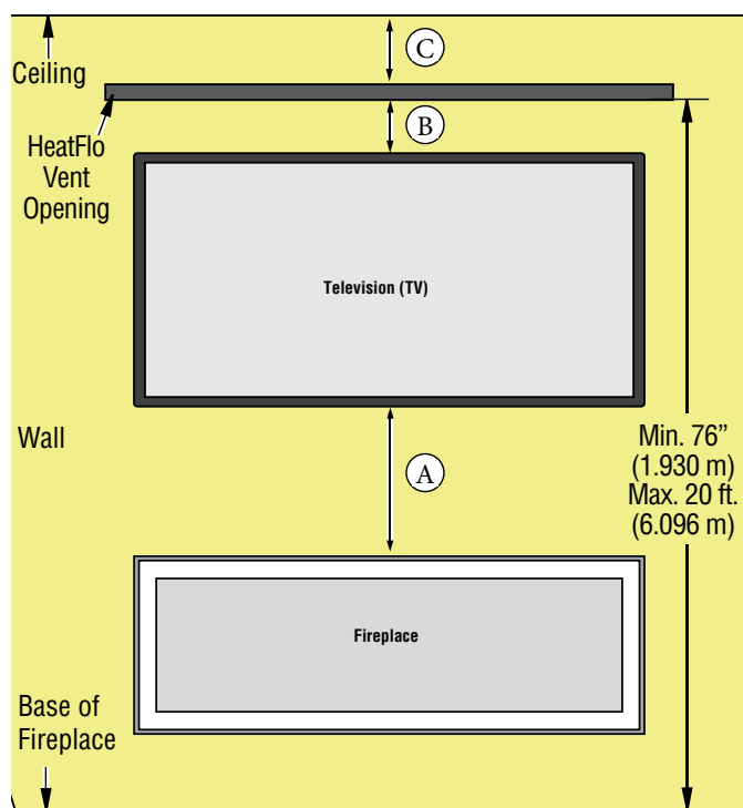
Figure 5 - Minimum Dimensions for Television (TV) Installed Above Fireplace (Flush Wall) when the optional HeatFlo Kit is installed.
