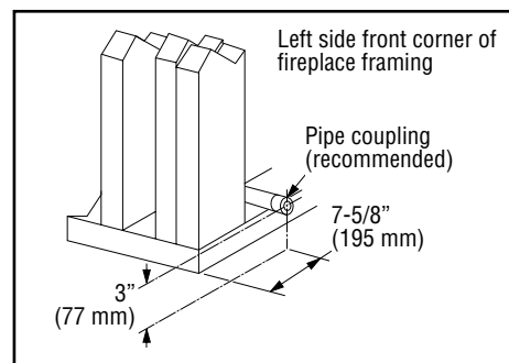
Figure 7 - Routing the gas line - all models
