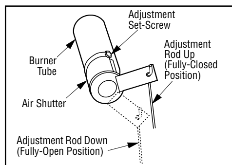
Figure 15 - Air Shutter Adjustment Rod
