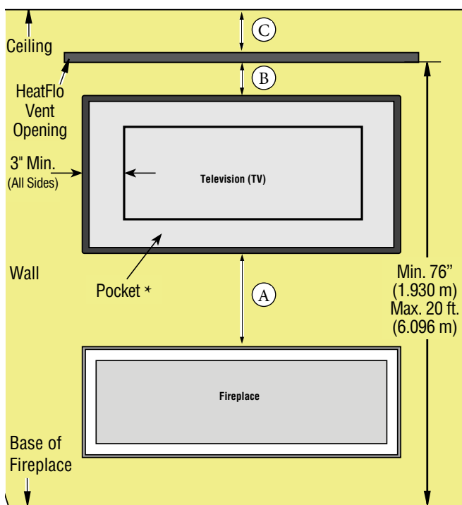
Figure 5A - Minimum Dimensions for Television (TV) Installed Above Fireplace on a Recessed Wall Pocket when the optional HeatFlo Kit is installed.
