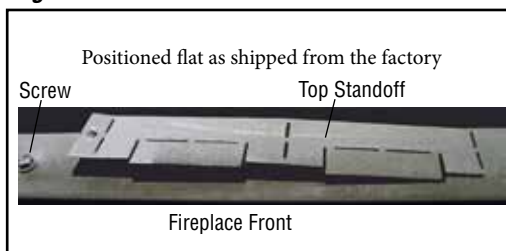
Figure 6 - Unassembled standoff
