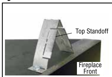
Figure 6A - Assembled standoffs
